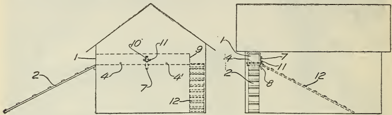
FIG. 15.—Front and side views of trap and feed house, with trap installed
