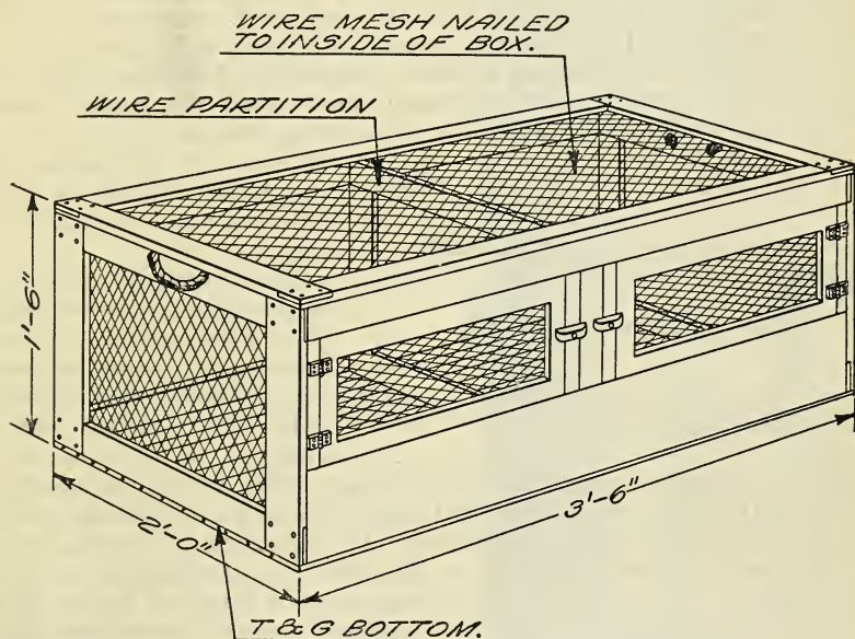
FIG. 24.—Shipping crate for two foxes, made of \frac{3}{8} -inch material, tongue-and-groove bottom, and 1-inch mesh, 14-gauge wire netting
