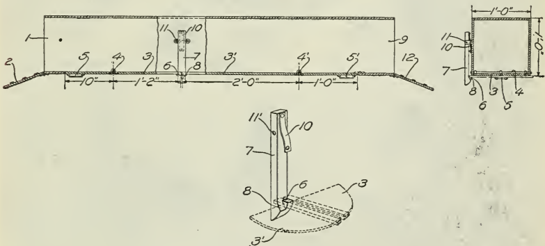
FIG. 17.—Details of construction of trap for feeding house. Operation described in text
