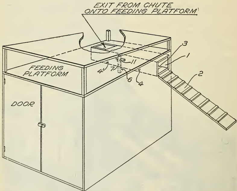
FIG. 16.—Trap and feed box that can be installed in a house of almost any description
