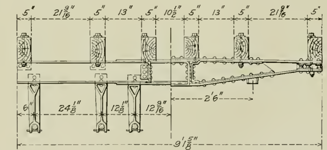
Half-Sections Through the Underframe
