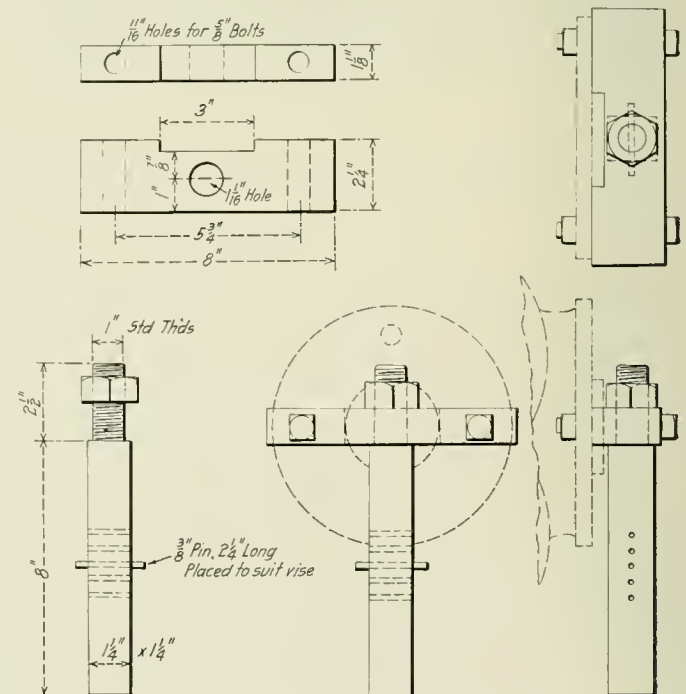
Arrangement for Holding Distributing Valve.
