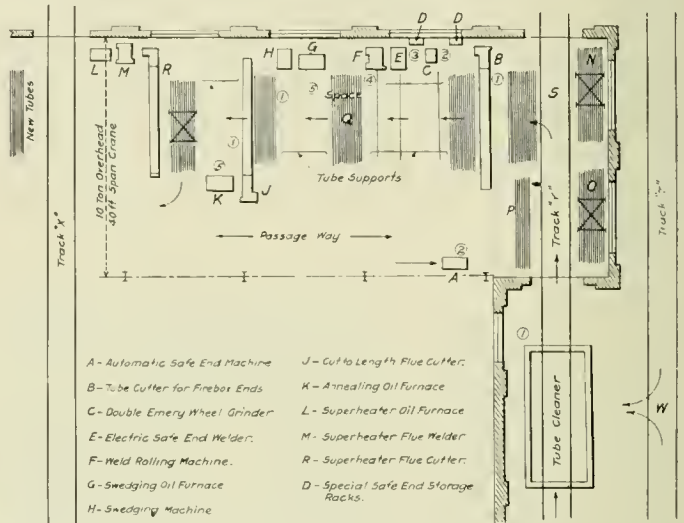
Layout of the Flue Shop
