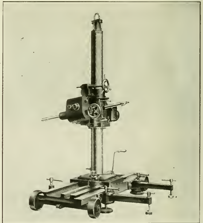
Portable Drilling and Tapping Machine
