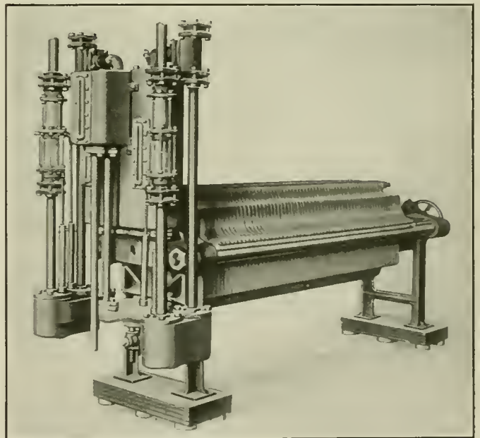
Bipolar Continuous Oxygen and Hydrogen Generator
