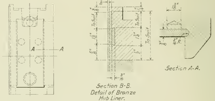
Details of Method of Reclaiming Worn Driving Boxes on the Union Pacific
