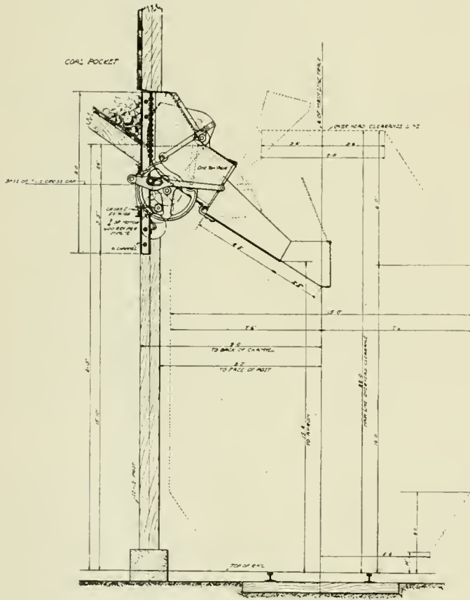
Device for Coaling Stations
