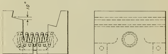
Fig. 8—Jig for Forming Wheel Boring Tools
