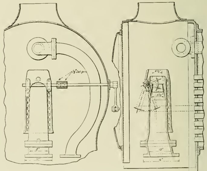
Jones Variable Exhaust Nozzle
