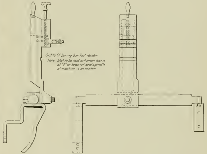
Turret Attachment for Jones & Lamson Turret Lathe
