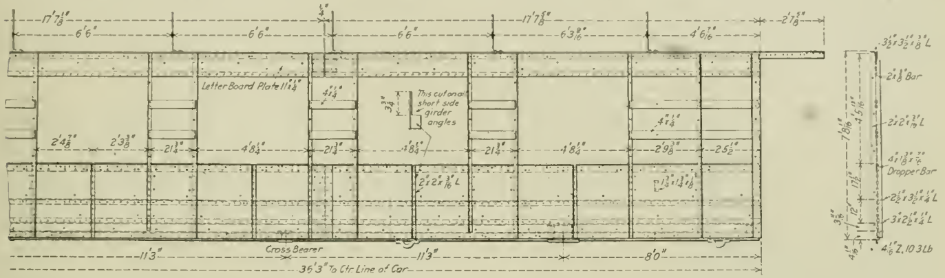
Steel Side Frame of the Dining Cars
