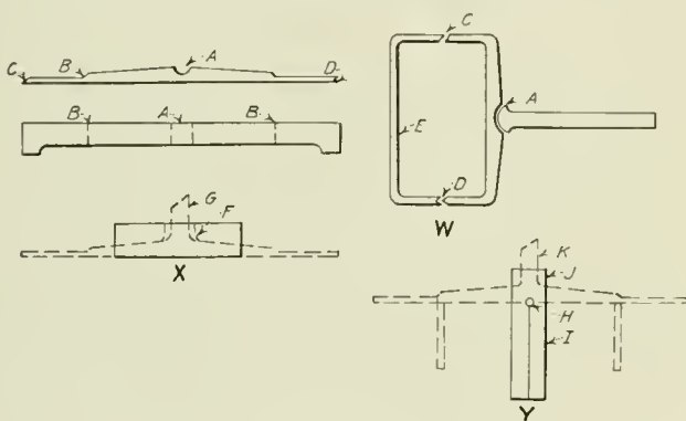
Fig. 5—Forging Valve Yokes
