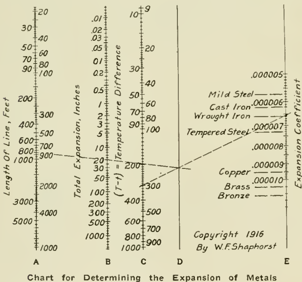
Chart for Determining the Expansion of Metals
