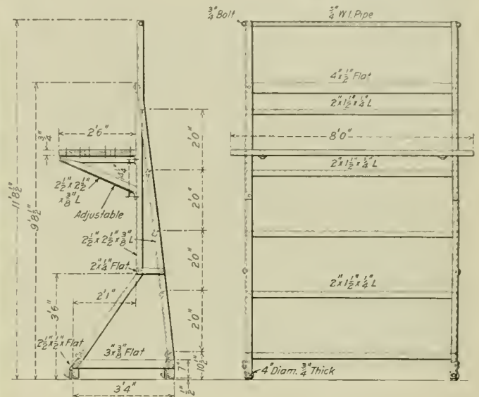
Fig. 3—Portable Scaffold for Boiler Work
