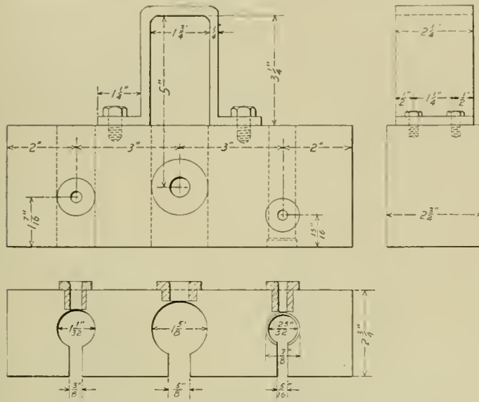
Fig. 6—Drill Jig for Brake Staffs
