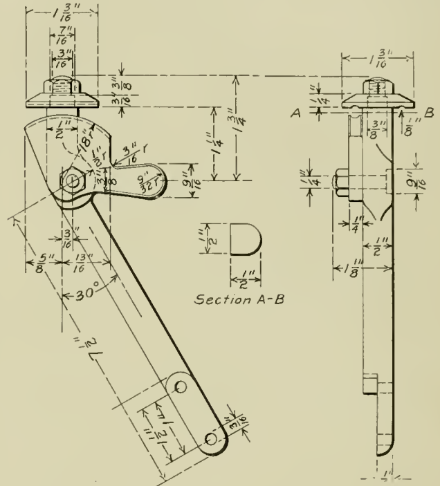
Simple Carbon or Wire Holder for Use in Electric Welding
