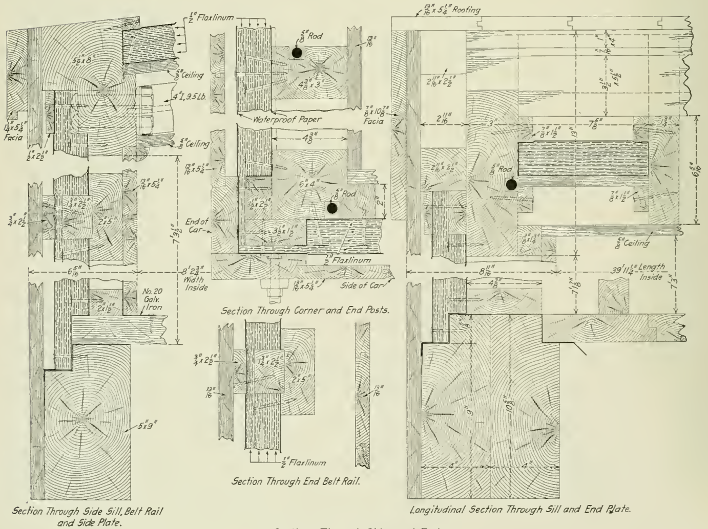
Sections Through Sides and Ends
