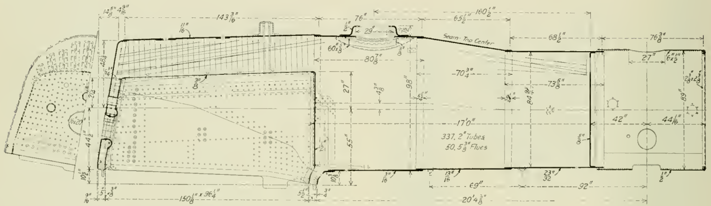
Boiler of the New York, Ontario & Western Locomotive
