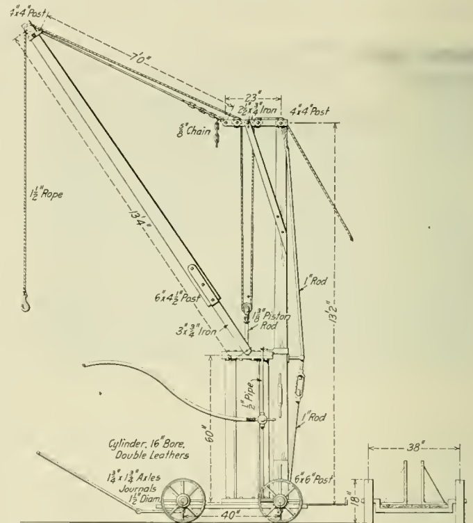
Portable Air Hoist for Roundhouses
