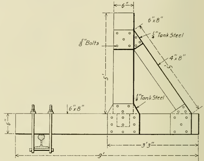
Fig. 4—Jack Support for Straightening Steel Car Sills
