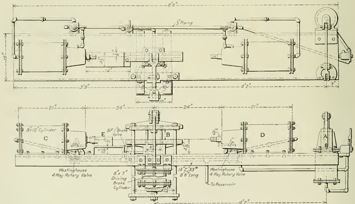
Machine for Stripping and Mounting Air Brake and Signal Hose
