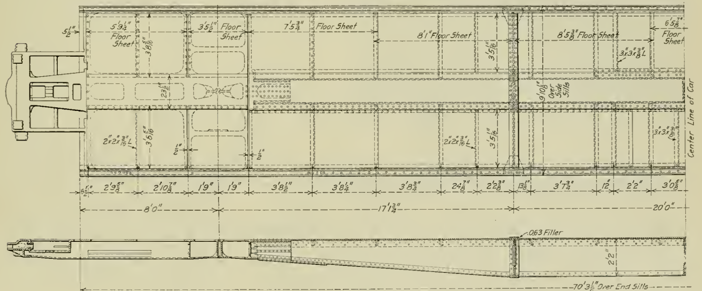
Underframe of the Boston & Maine Coach
