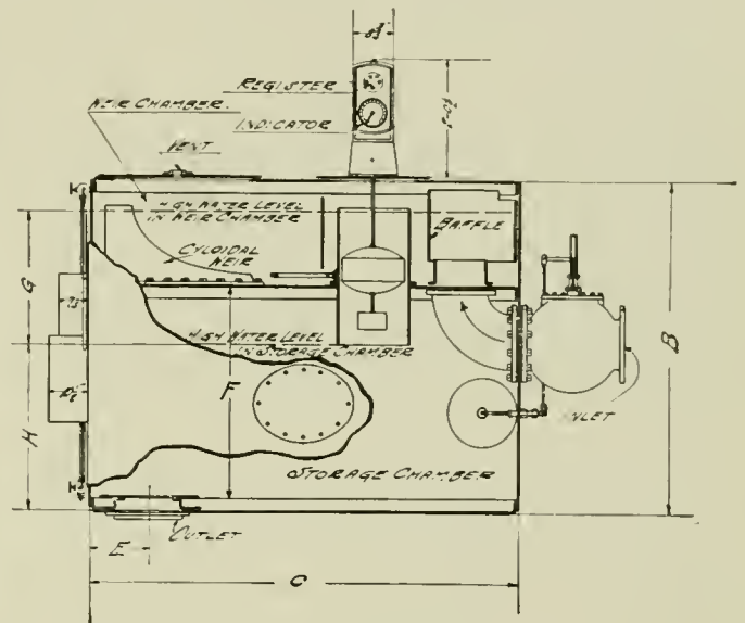
Cycloidal Weir Meter; Rate of Flow Varies Directly with the Head
