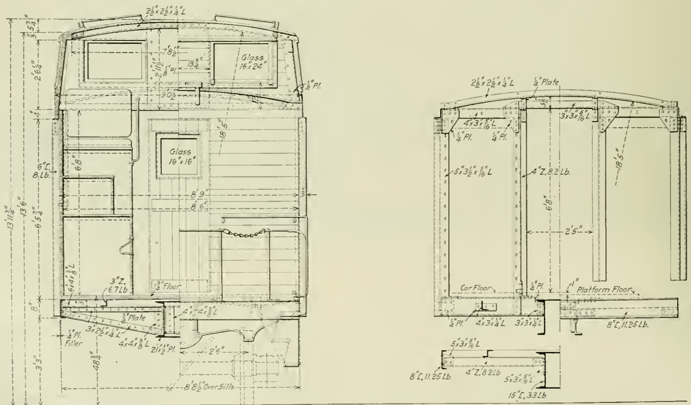
End Elevation and Sections of the N. C. & St. L. Caboose Cars
