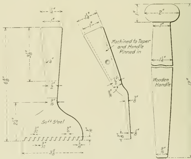
Carpet Stretcher for Use at Car Terminals
