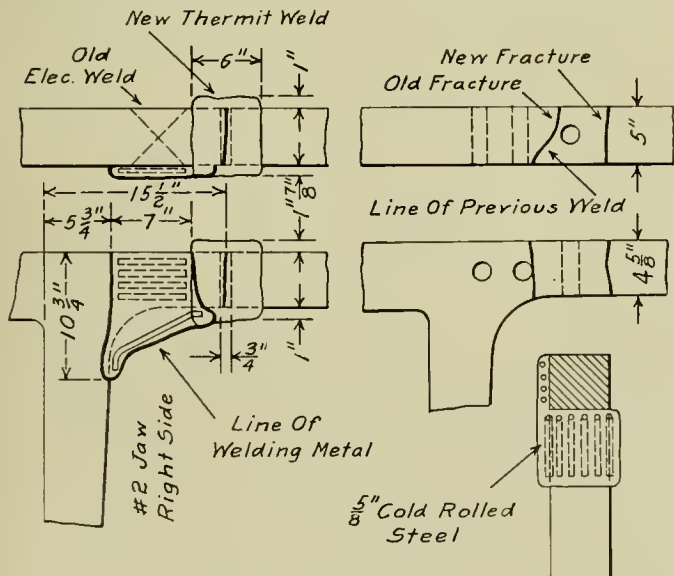
Fig. 2—Cast Steel Frame Thermit Weld
