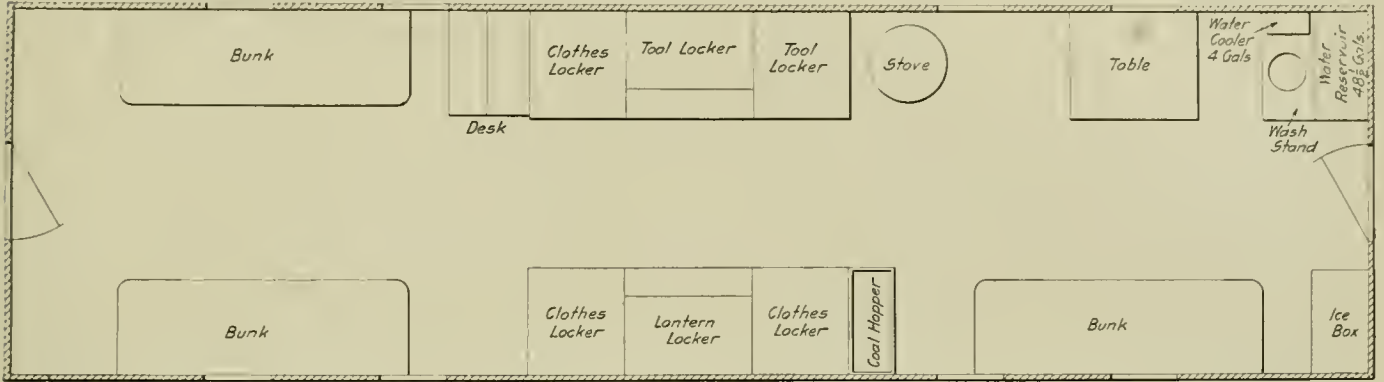
Floor Plan of N. C. & St. L. Caboose Cars
