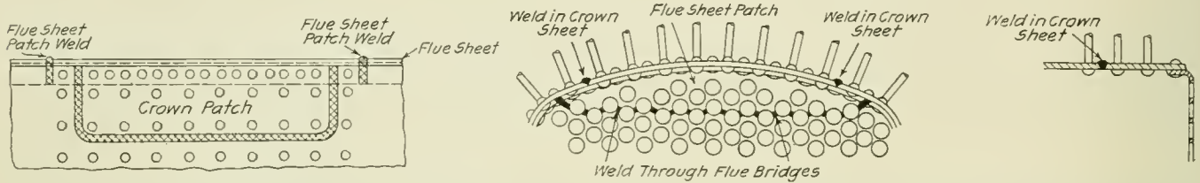
Fig. 6—Crown and Tube Sheet Patch Made by Oxy-Acetylene Welding Process
