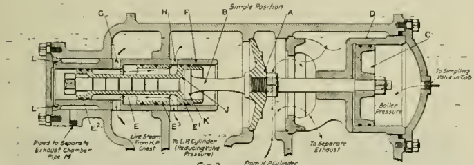
Sections Showing the Construction and Operation of the Simplex Intercepting Valve
