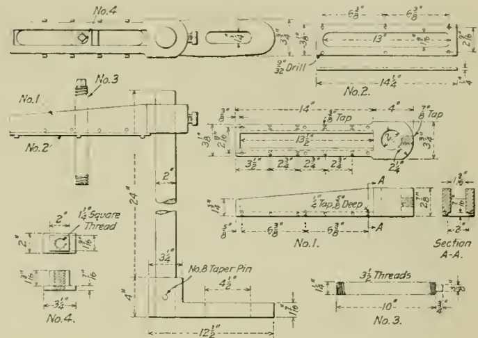
Details of Drilling Post with Adjustable Center
