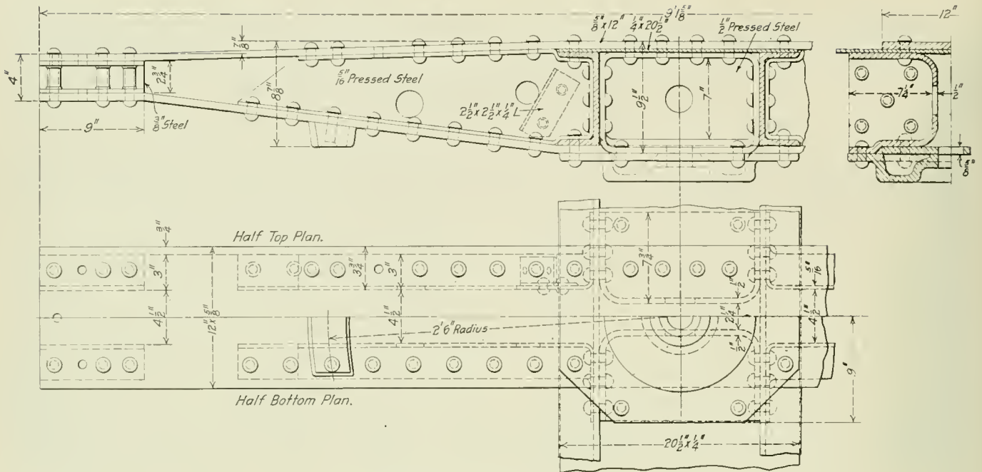
Body Bolster for Santa Fe Box Cars
