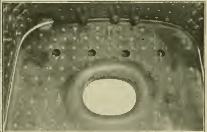
Fig. 2—Door Sheet of New Firebox Partially Welded In
