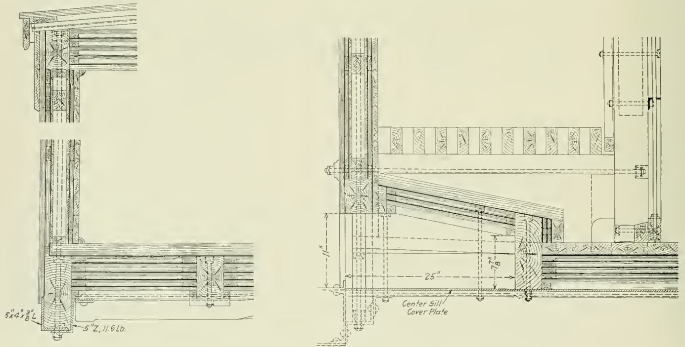
Sections Through Side, Roof, End and Floor, Showing Recess for Buffer
