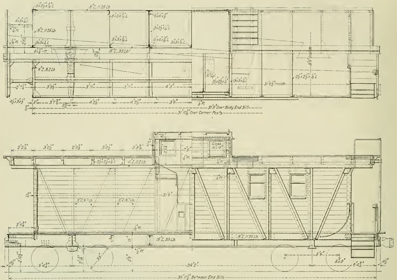
Plan and Elevation of the Caboose Cars
