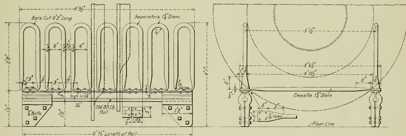
A Convenient Rack for Storing Smoke Box Fronts
