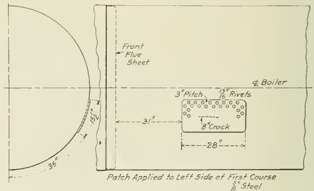
Fig. 4—This Patch Reduced the Factor of Safety to Less than Three
