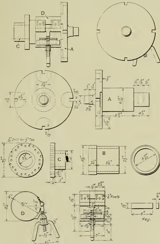
Jig for Finishing Air Pump Packing Rings
