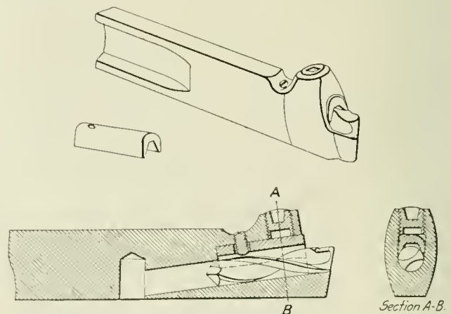
Holder Using Broken Drills for Cutting Tools
