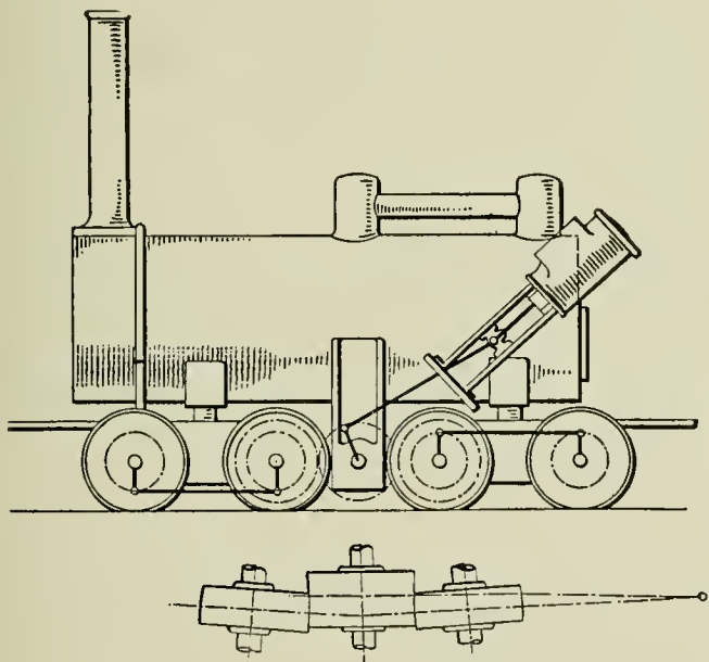
Fig. 1—Gear Transmission Locomotive
