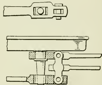
Fig. 11—Vogel System of Offset Rods
