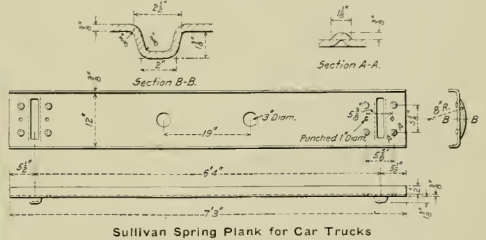
Sullivan Spring Plank for Car Trucks
