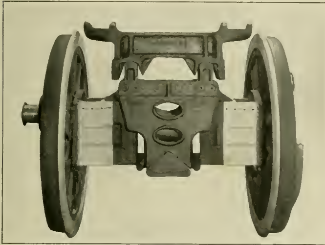
Lateral Motion Device Assembled on the Axle
