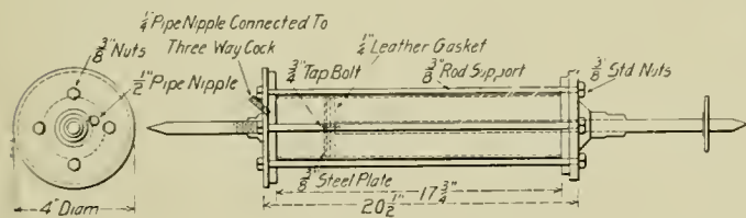
Fig. 13—Jack for Removing Expanded Tires in the Roundhouse
