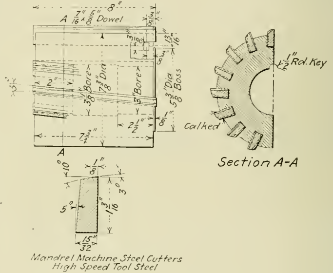
Fig. 16.—Details of the Milling Cutters Shown in Fig. 15
