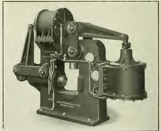
Spring Banding Press of 100 Tons Capacity
