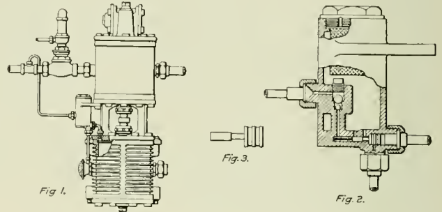
Air Pump Lubricator for Both Air and Steam Cylinders
