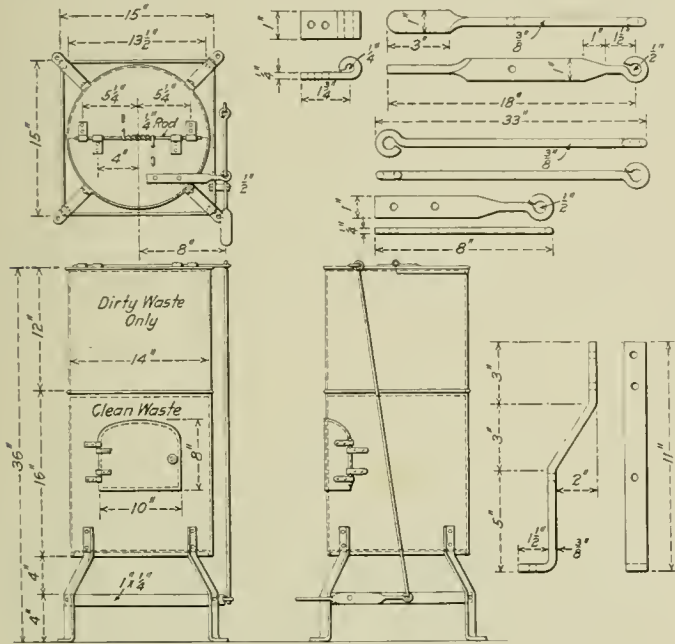
Storage Can for Waste
