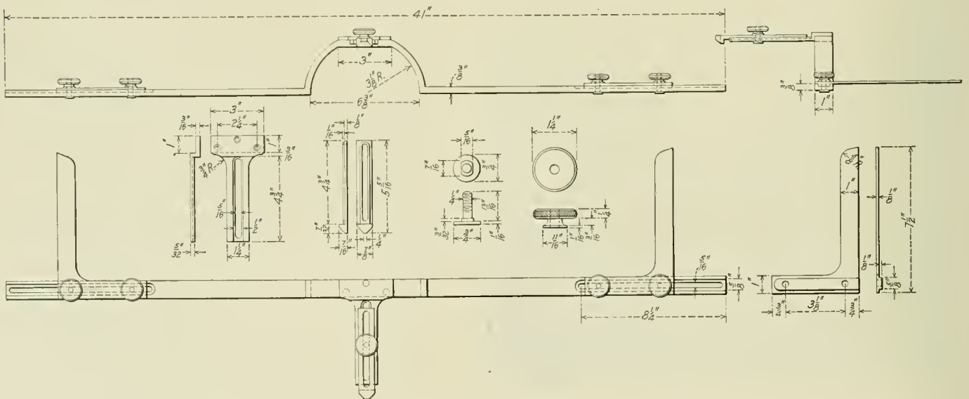
Details of the Gauge for Determining the Proper Location of Wheels on the Axle
