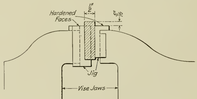
Jig Used in Testing Pneumatic Chipping Hammers
