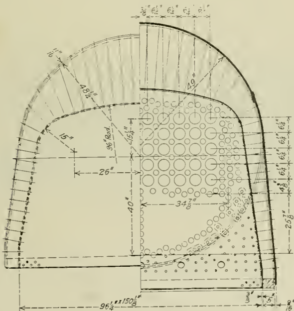
Cross Sections of the Boiler
