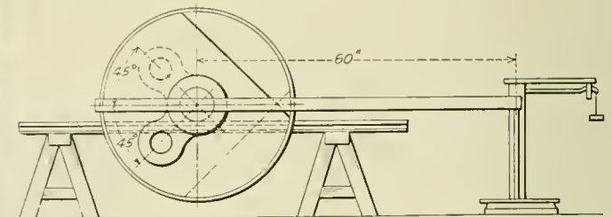
Method of Weighing Counterbalances on the Southern Pacific
