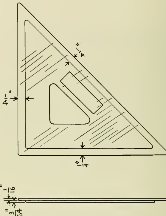
Convenient Triangle for Use in Tracing
