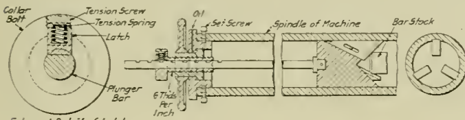
Enlarged Detail of Latch.
