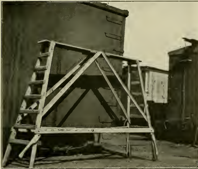
Portable Scaffold with Rollers and Drop Handles
