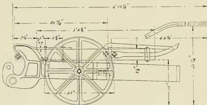
Fig. 2—Truck for Carrying Couplers
