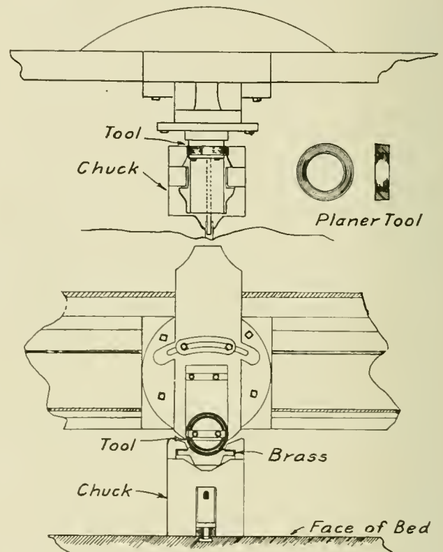
Fig. 3—Broaching Tool for Reclaiming Car Brasses
