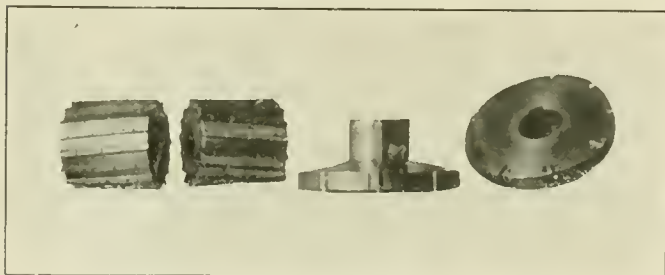
Fig. 15—Milling Cutters and Valve Chamber Boring Cutters
