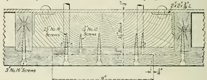
Canadian Northern Letter Board Splice
