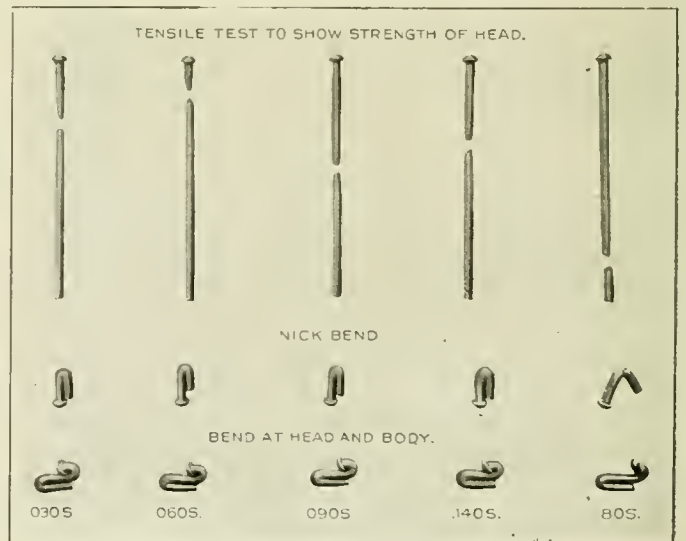
Fig. 6—Tests of Rivets Quenched from Driving Heat
