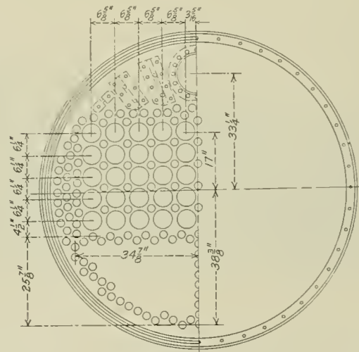
337, 2" Tubes 50, 5 3/8" Flues.
