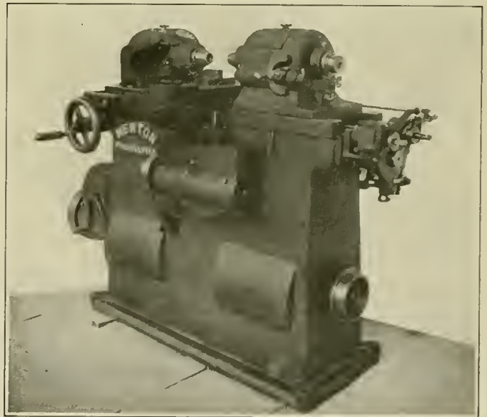
Duplex Keyseat Milling Machine
