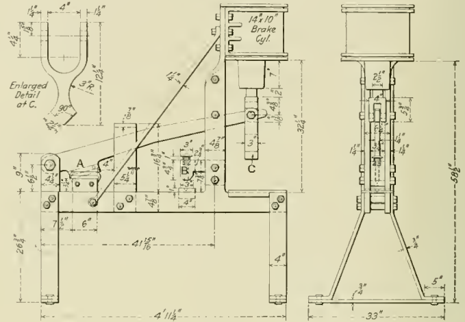
Details of Spring Shear and Bending Machine
