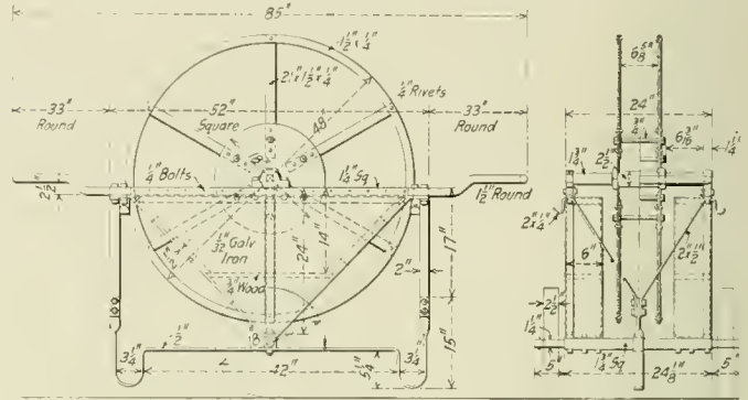
Washout Hose Car
