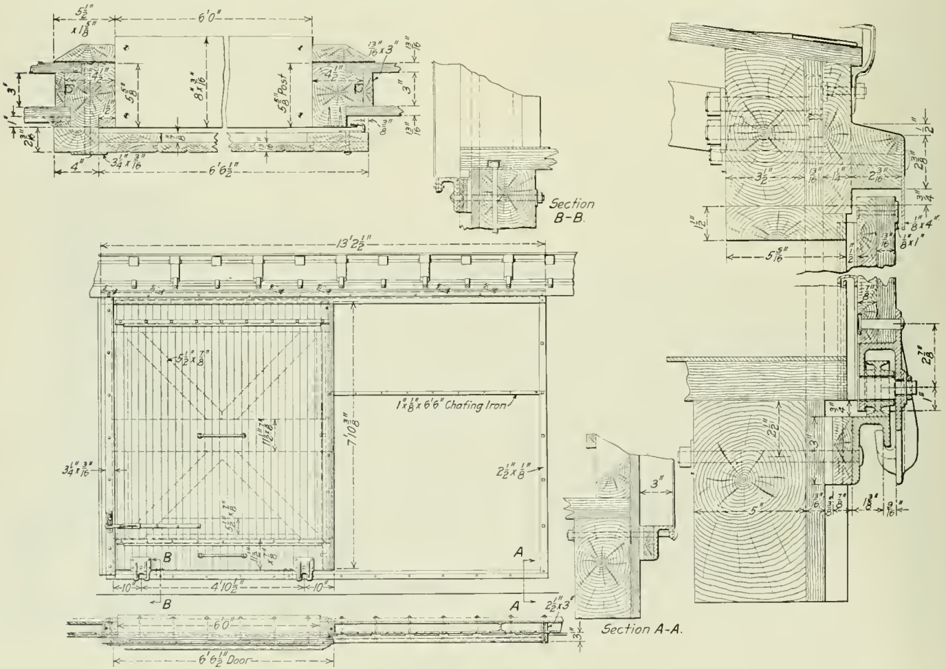
Santa Fe Box Car—Side Door Construction
