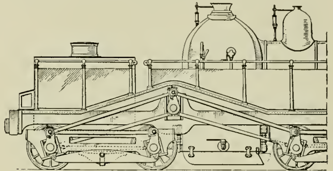
Fig. 8—Kirchweger Free-Axle Locomotive
