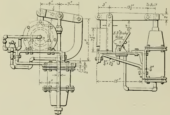
End Views of the Hose Stripping Machine
