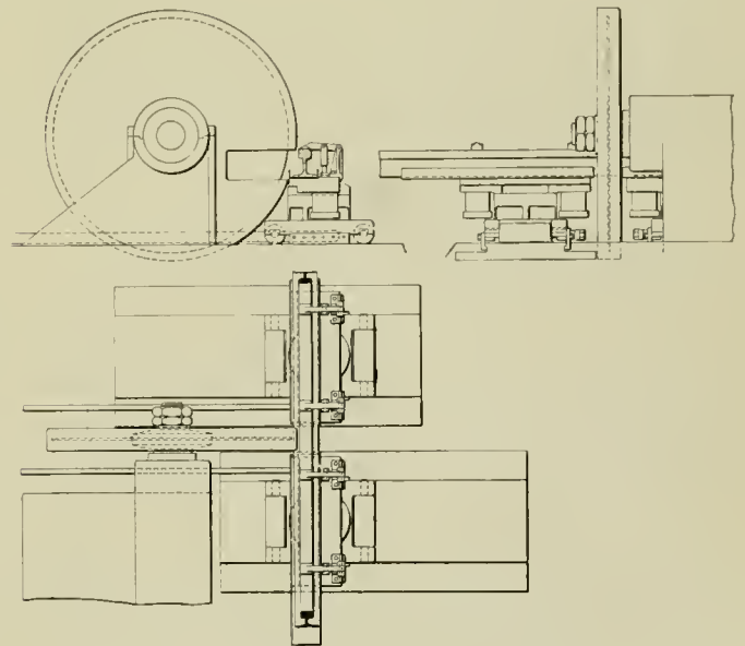
Arrangement of the Saw and Carriages
