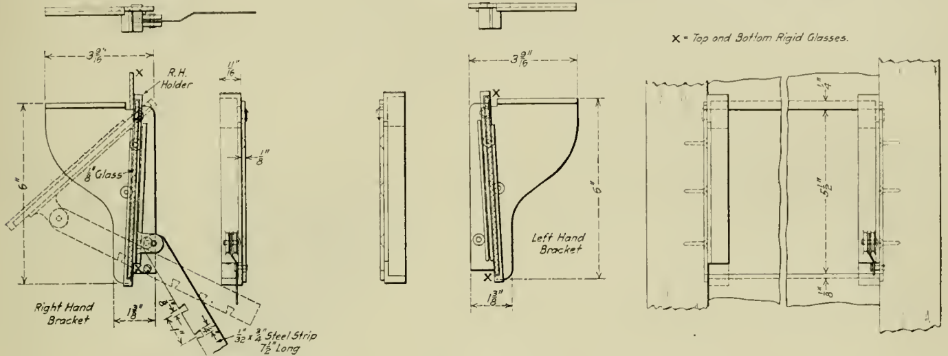
Details and Application of Clear Vision Window to Front Cab Windows
