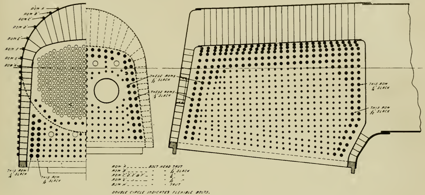
Fig. 4—Application of Flexible Staybolts to Relieve Working Stresses in Locomotive Fireboxes
