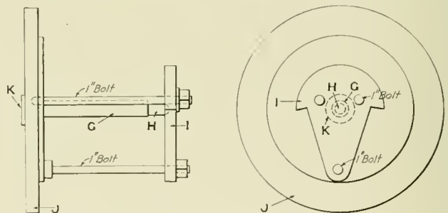
Fig. 2—Chuck for Clamping the Brass on the Slotter Table
