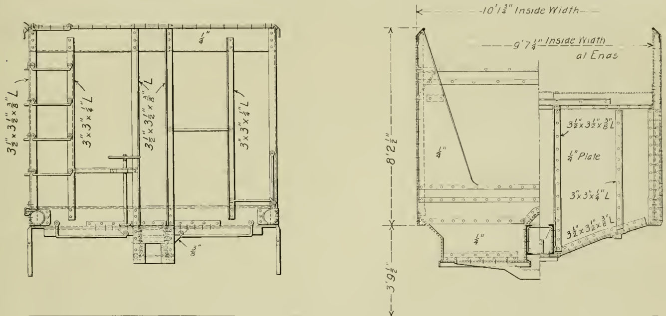
End Elevation and Cross Sections of the Woodward Iron Company's 100-Ton Car
