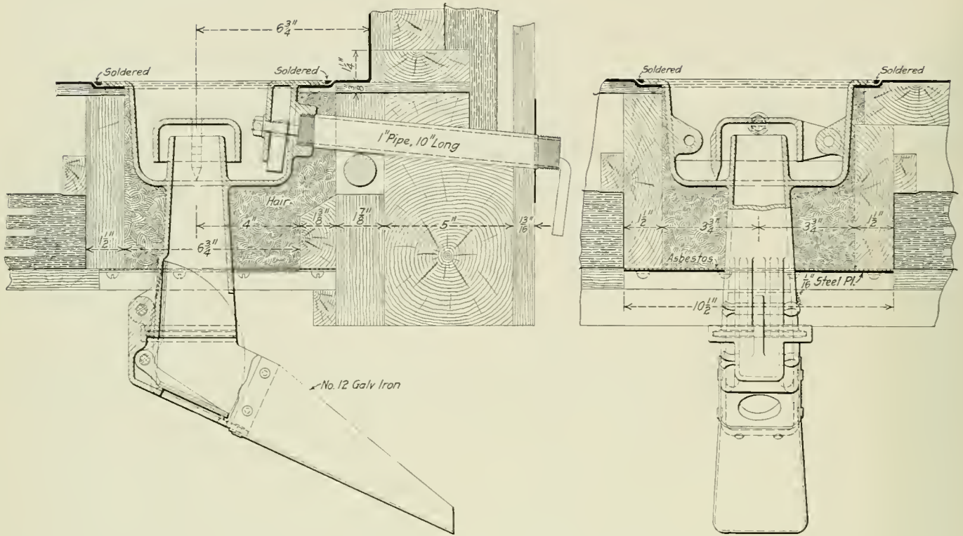
Malleable Iron Double Trap and Drain; Santa Fe Refrigerator Car
