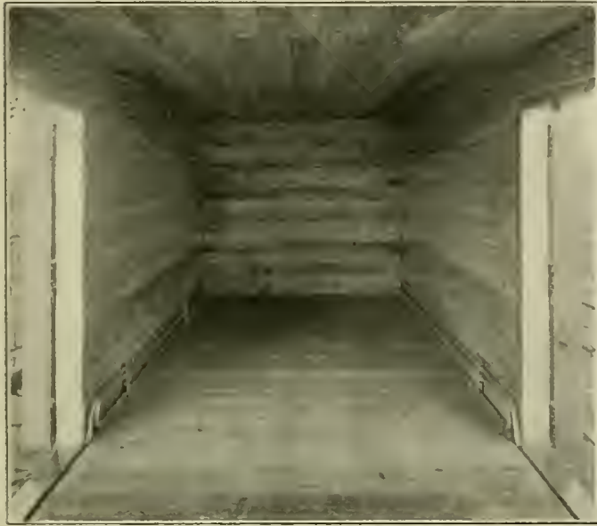
Interior View Showing Refrigerating Coils Located on Upper Side Walls and Near the Floor
