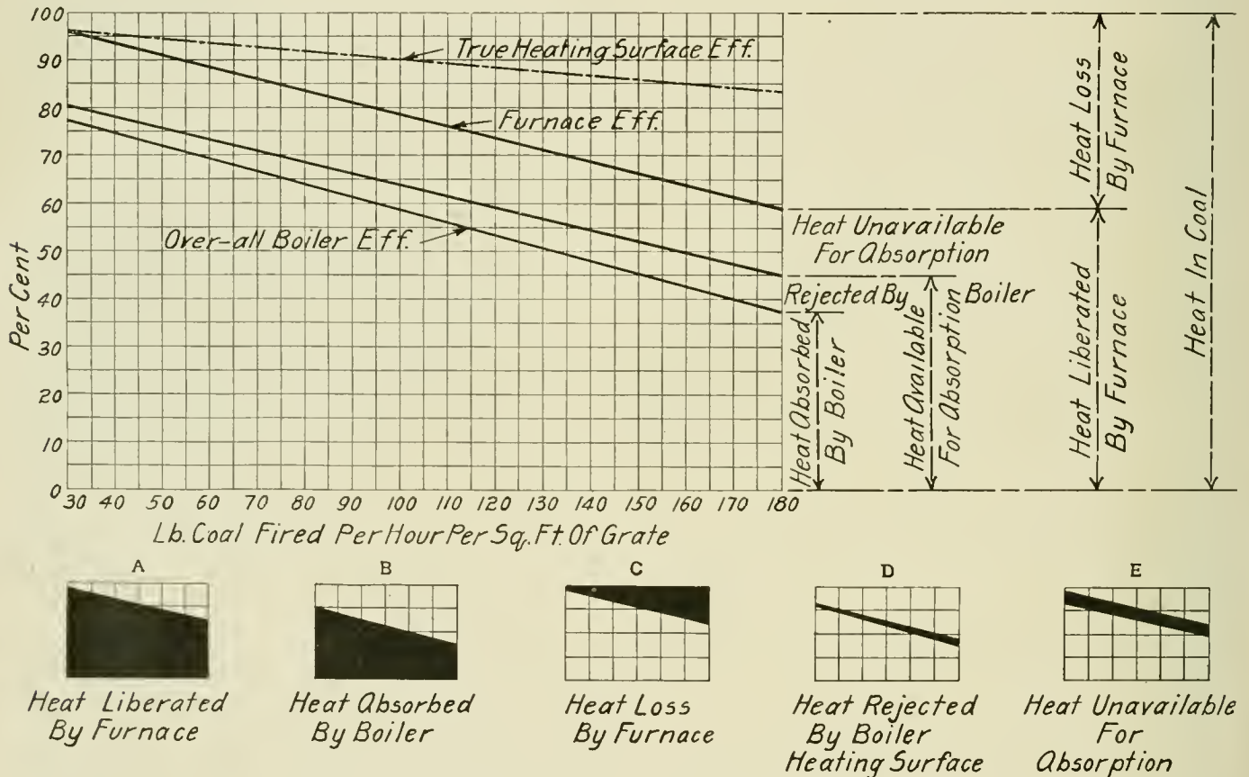
Fig. 2—Diagram Showing Heat Distribution in a Locomotive Boiler
