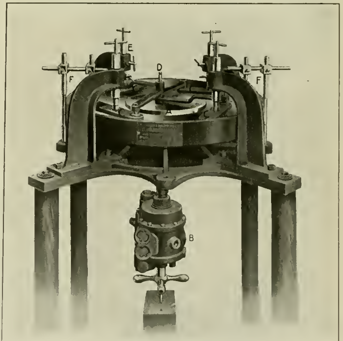
Reflex Water Glass Grinding Machine
