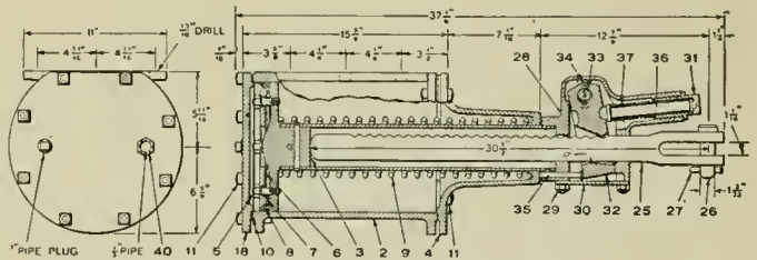
Fig. 2—Load Cylinder, Showing Notched Push Rod and Clutch
