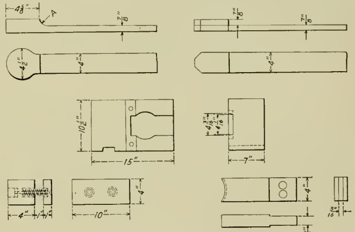
Fig. 3—Dies for Forming Spring Hanger Ends
