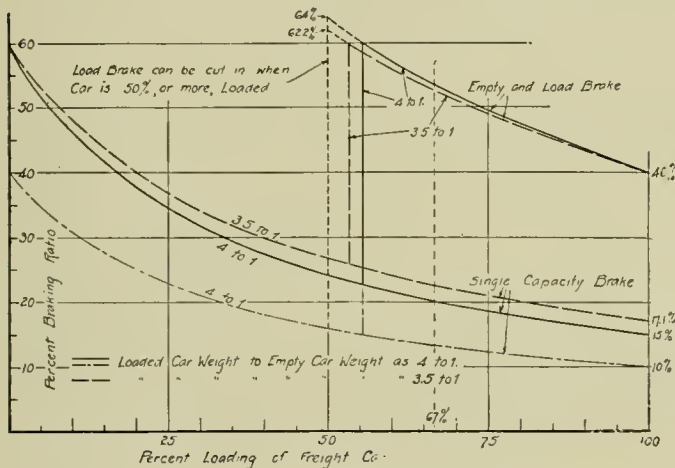
Fig. 1—Chart Showing Braking Ratios for Various Conditions of Freight Car Loading, with and without Empty and Load Brake
