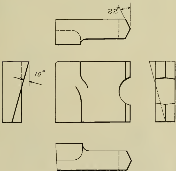
Fig. 7—Tool for Boring Car Wheels
