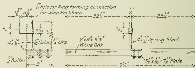
Journal Jack Block with Wheel Clamp
