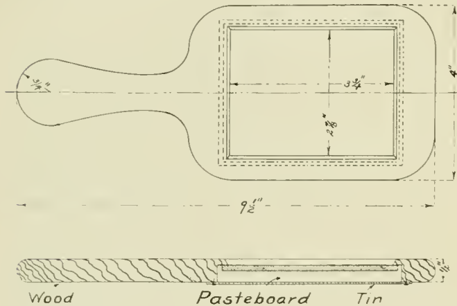
Fig. 1—Hand Mirror for Inspecting the Inner Side of Arch Bars
