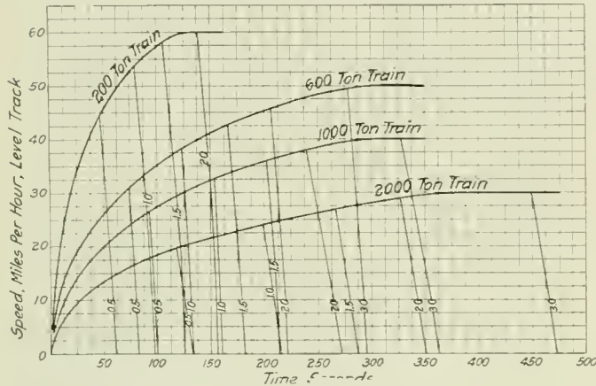
Fig. 2—Speed—Time Curves
