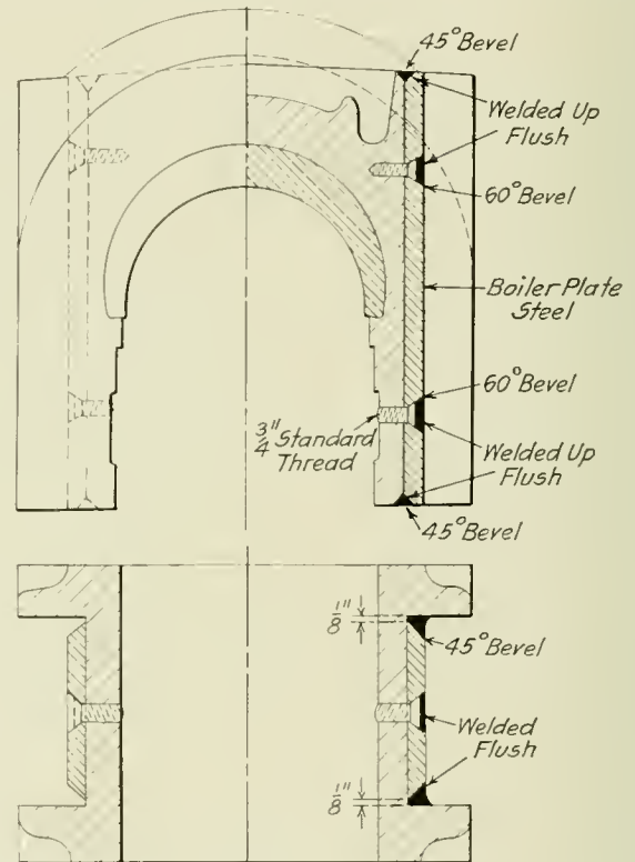
Driving Box with Steel Plates on the Shoe and Wedge Faces
