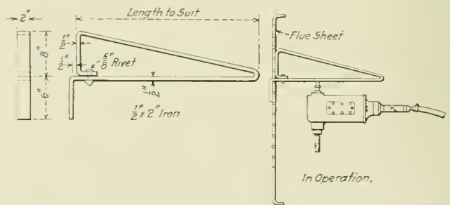
Old Man for Attachment to Tube Sheet
