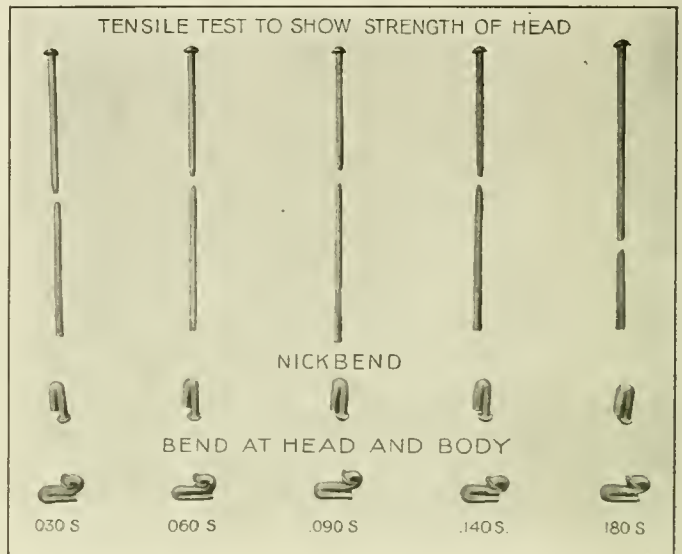
Fig. 5—Tests of Rivets in Ordinary Cold Condition
