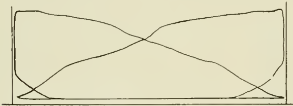
Fig. 2—Young Valve Gear Indicator Card at a Speed of 40 Miles per Hour
