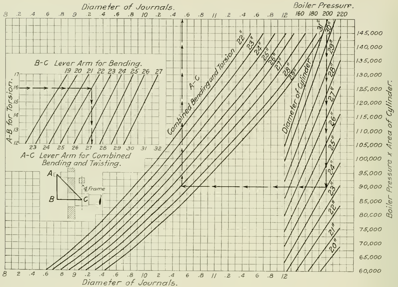
Fig. 1—Diagram for Determining the Diameter of Driving Axle Journals
