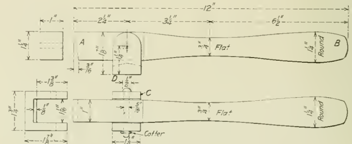
Window Raiser for Coaches
