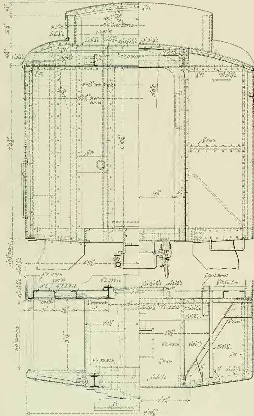
Details of the End Construction of the Boston & Maine Coach
