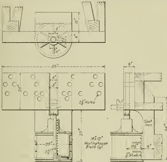
Apparatus for Bending Pipe
