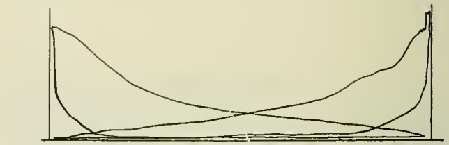
Fig. 4—Young Valve Gear Indicator Card at a Speed of 77 Miles per Hour
