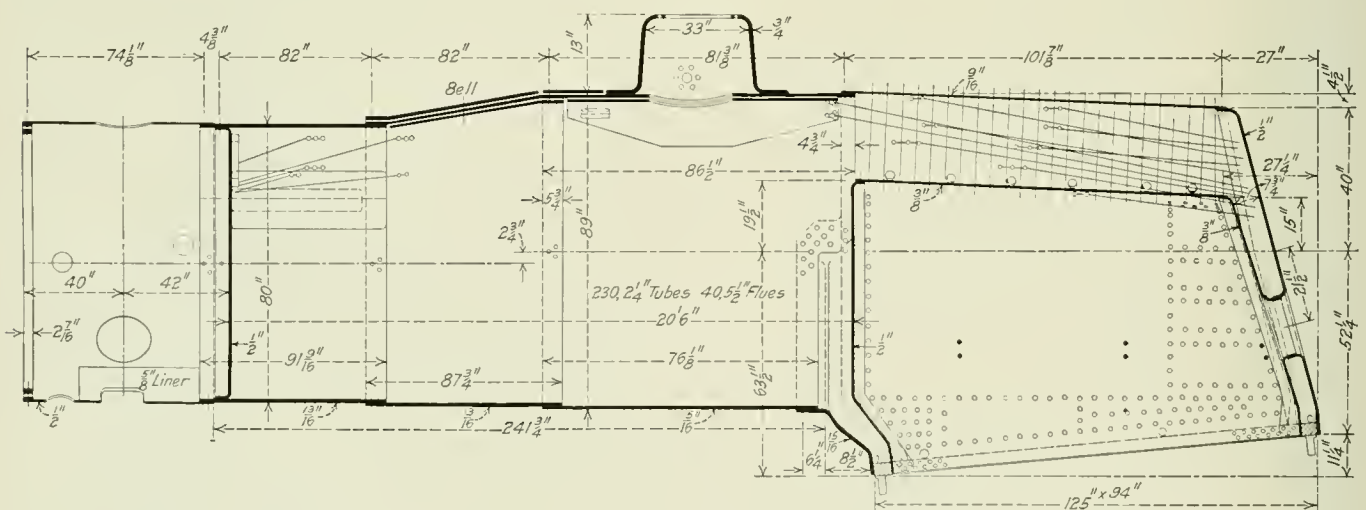
Boiler of the Richmond, Fredericksburg & Potomac Locomotive
