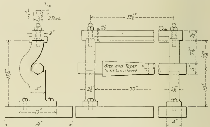
Mandrel and Jig for Babbitting Crossheads
