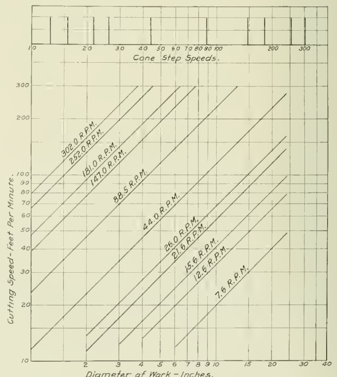
Fig. 6—Logarithmic Chart of Cutting Speeds of Lathe Referred to in Fig. 1
