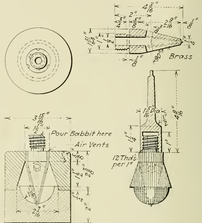
Fig. 10—Grinder for Superheater Header
