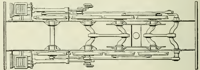
Fig. 5—Aliges' Four-Axle Locomotive
