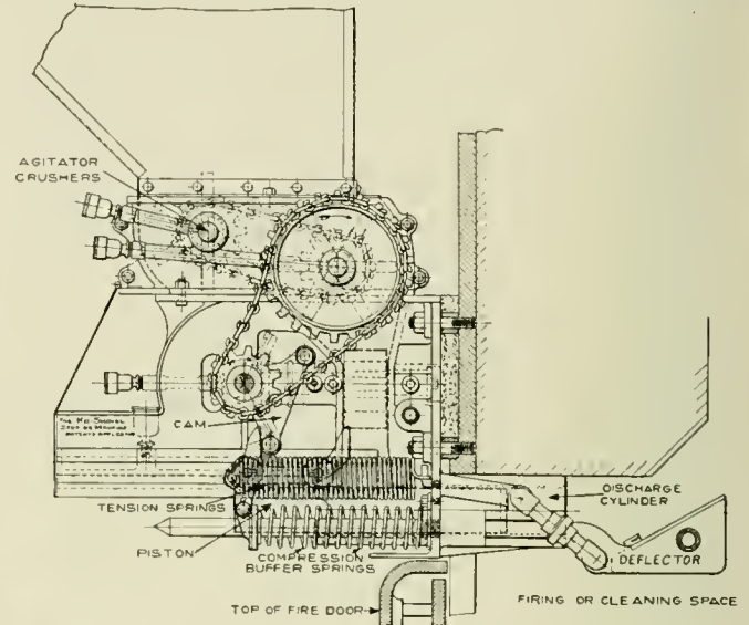
Section Through the Ko-Shovel Mechanical Stoker
