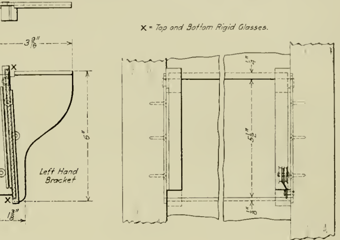
Details and Application of Clear Vision Window to Front Cab Windows
