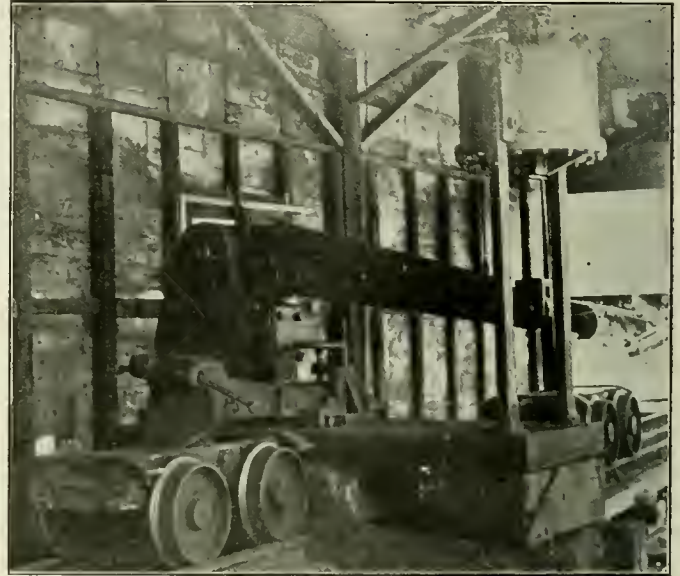
Machine for Removing Coupler Yokes
