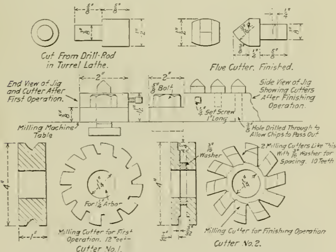
Jig for Making Tube Cutters on a Milling Machine
