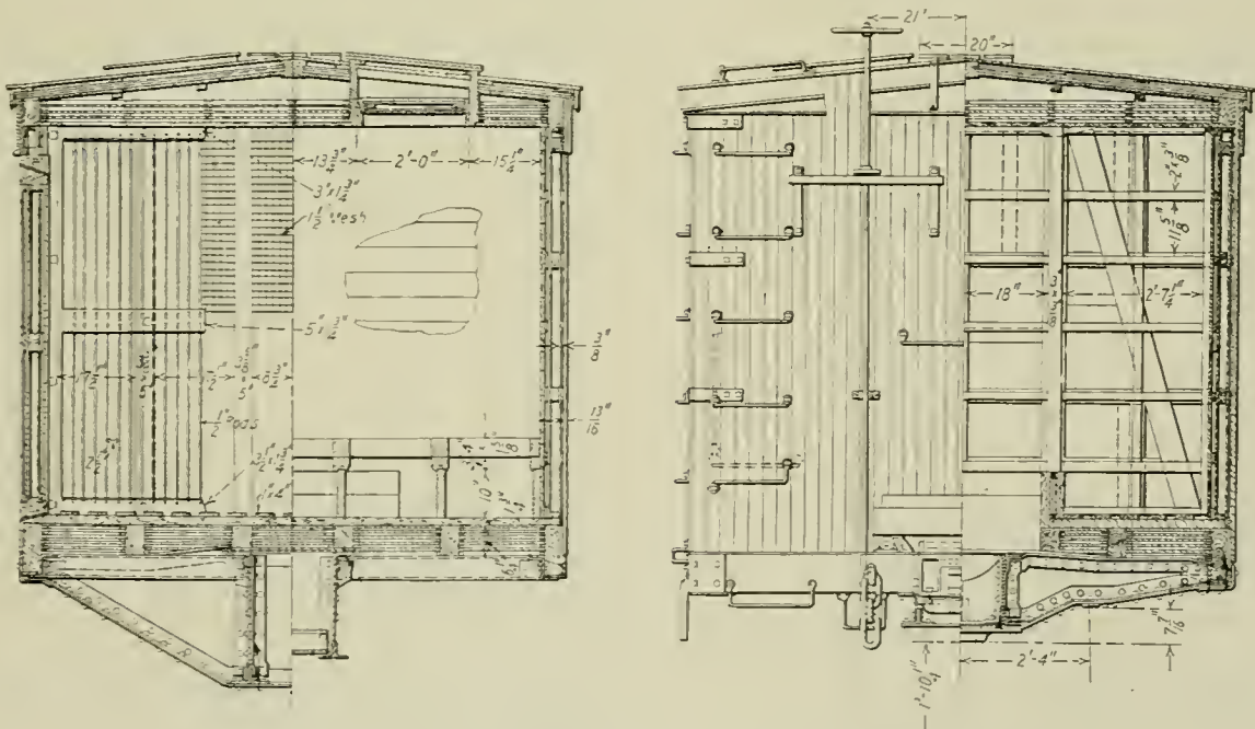
Cross Sections of the Northern Pacific Express Refrigerator Car
