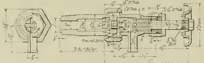
A Self-Grinding Gage Cock
