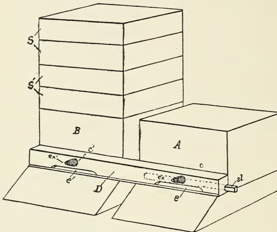
FIG. 70.—Beehives with Langdon non-swarmers attached: A, B , hives; S, S' , supers; D , non-swarming device; e, e' , entrances corresponding to hive entrances; sl , slide for closing entrance; e, e' , conical wire-cloth bee-escapes; ex, ex' , exits of same. (From Insect Life .)
