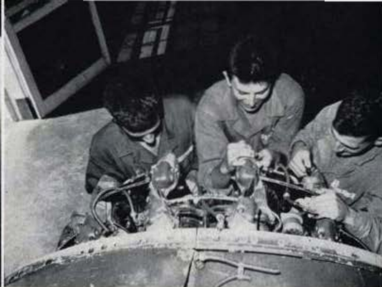
Safetying aircraft engine
