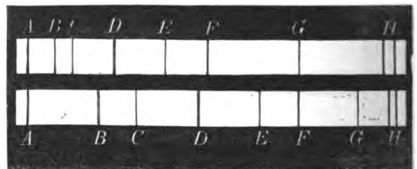
FIG. 7.—Comparison of prismatic with grating spectrum.
