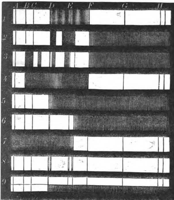
FIG. 5.—Absorption spectra.
