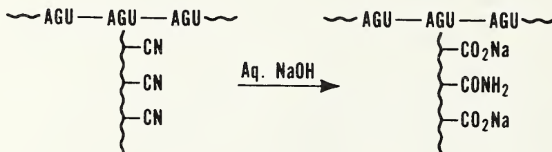
Figure 10.--Saponification of starch-polyacrylonitrile graft polymer.
