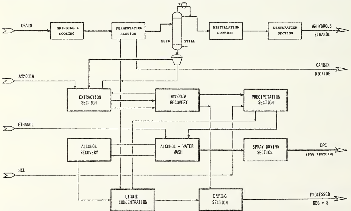
FIGURE 2 - Protein Recovery Process (Ammonia Case).
