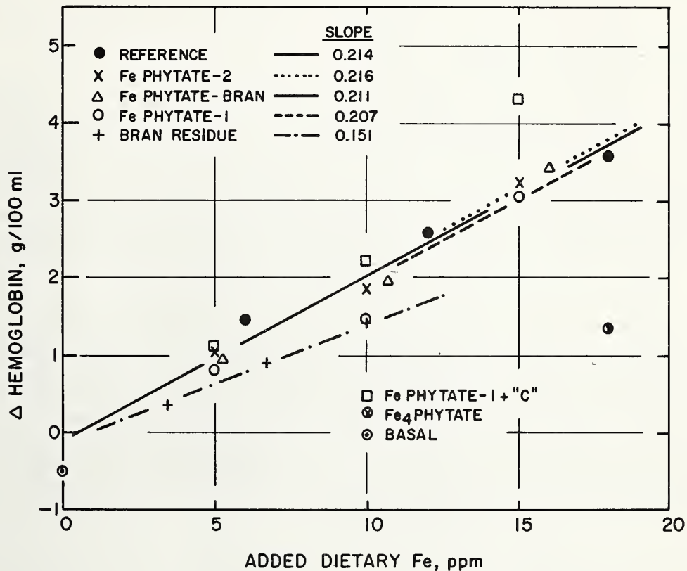
Figure 4. Slope ratio analysis of biological availability assay.
