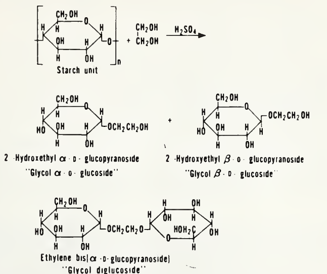
Figure 1.--Preparation of polyols from starch.
