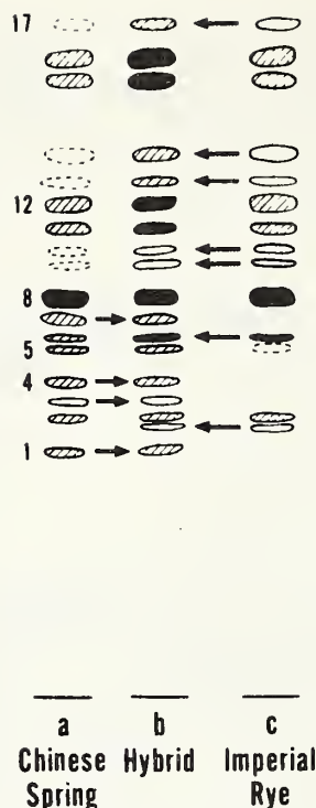
Figure 14. Glutenin analysis in a wheat-rye hybrid: (a) Chinese Spring wheat, (b) Chinese Spring X Imperial hybrid, and (c) Imperial rye.
