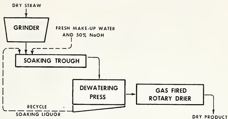
Fig. 4. Alkali soaking.
