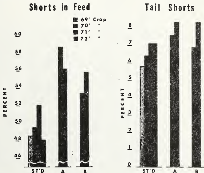
Figure 1. Percent shorts (head and tail) in total feed products and percent extraction of tail shorts.
