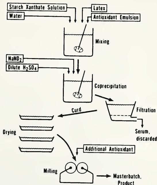
Figure 7.--Incorporation of starch xanthide in rubber.
