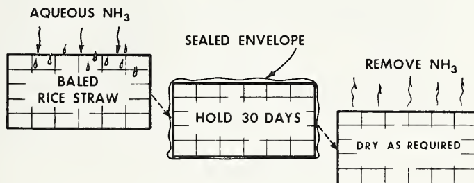
Fig. 5. Ambient temperature ammoniation.
