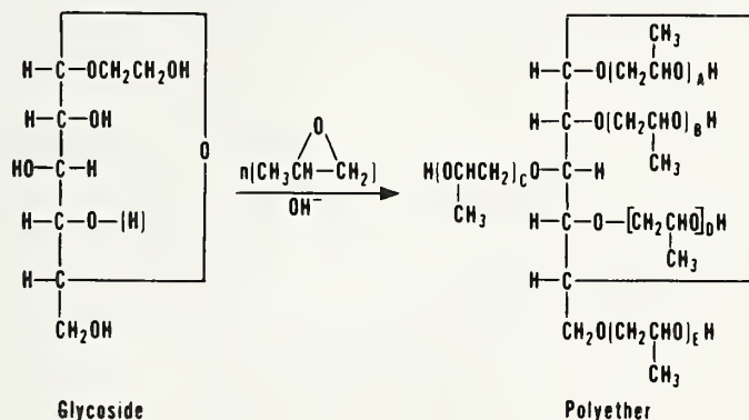
Figure 2.--Etherification of polyols.
