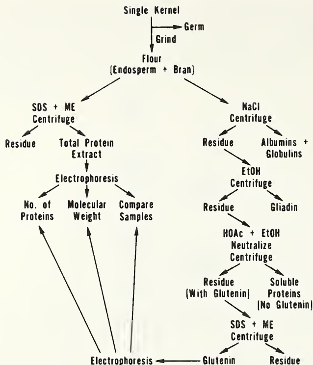
Figure 4. Single-kernel extraction of wheat proteins and analysis by SDS-PAGE after cleavage with 2-mercaptoethanol (ME).
