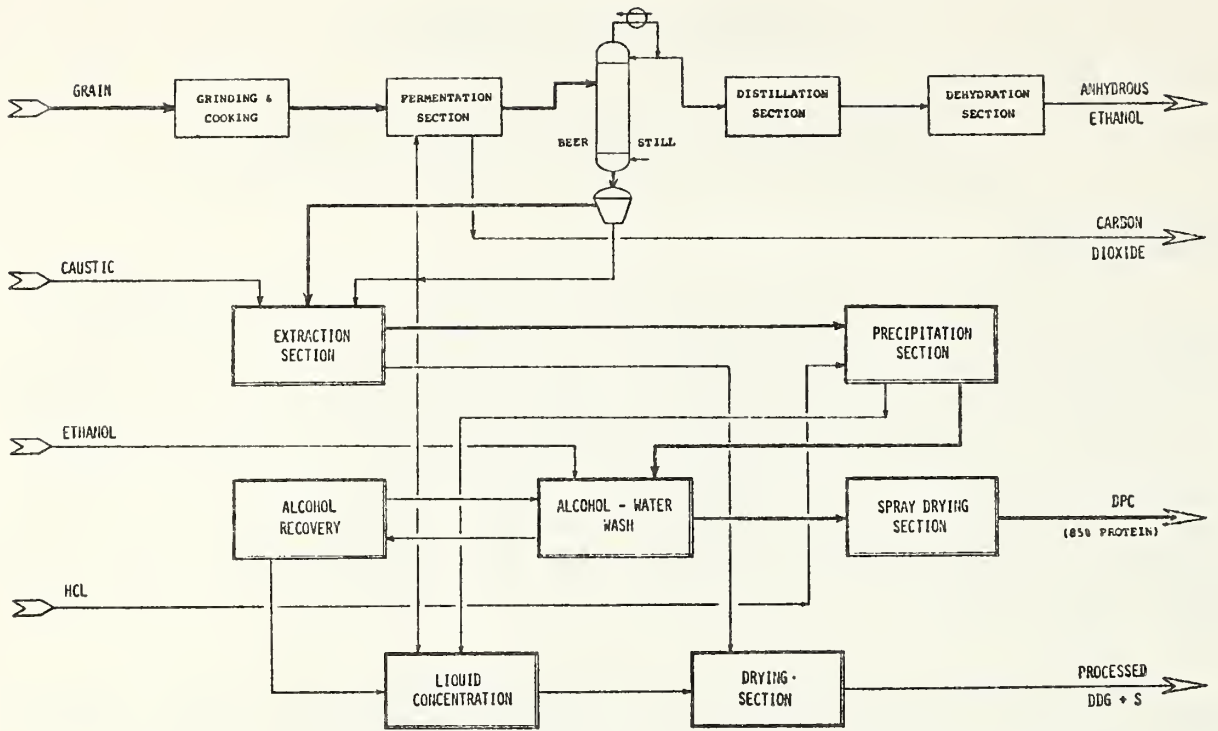
FIGURE 1 - Protein Recovery Process (Caustic Case).
