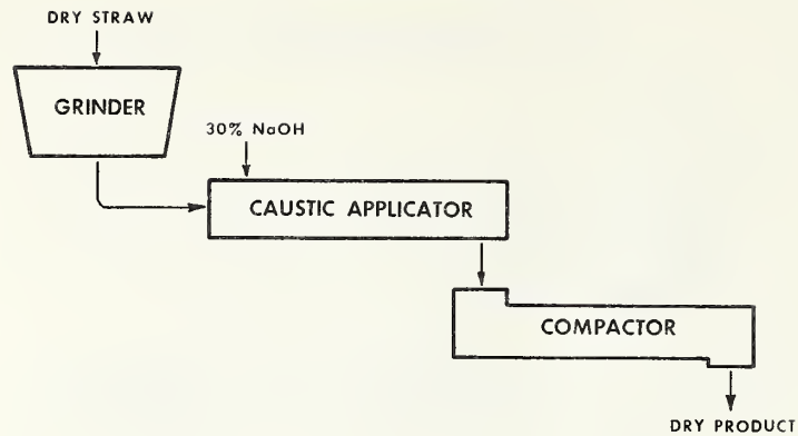
Fig. 6. Low moisture alkali compaction.
