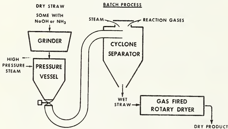
Fig. 3. High pressure steam treatment.
