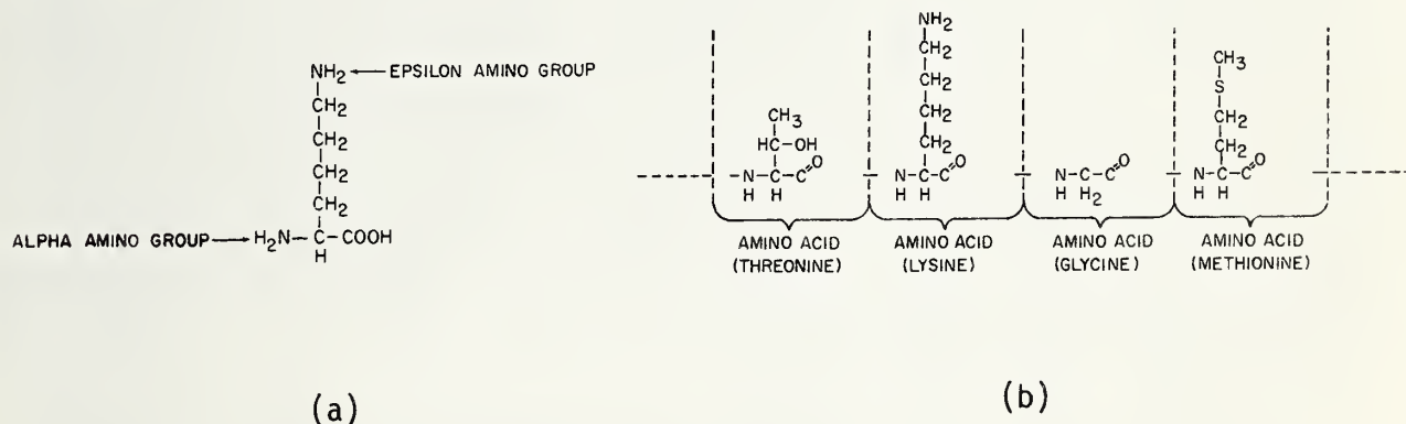
Figure 1. (a) Structure of free lysine showing free epsilon and alpha amino groups; (b) lysine as it would exist in a portion of a peptide chain of a theoretical protein; note free epsilon amino group.
