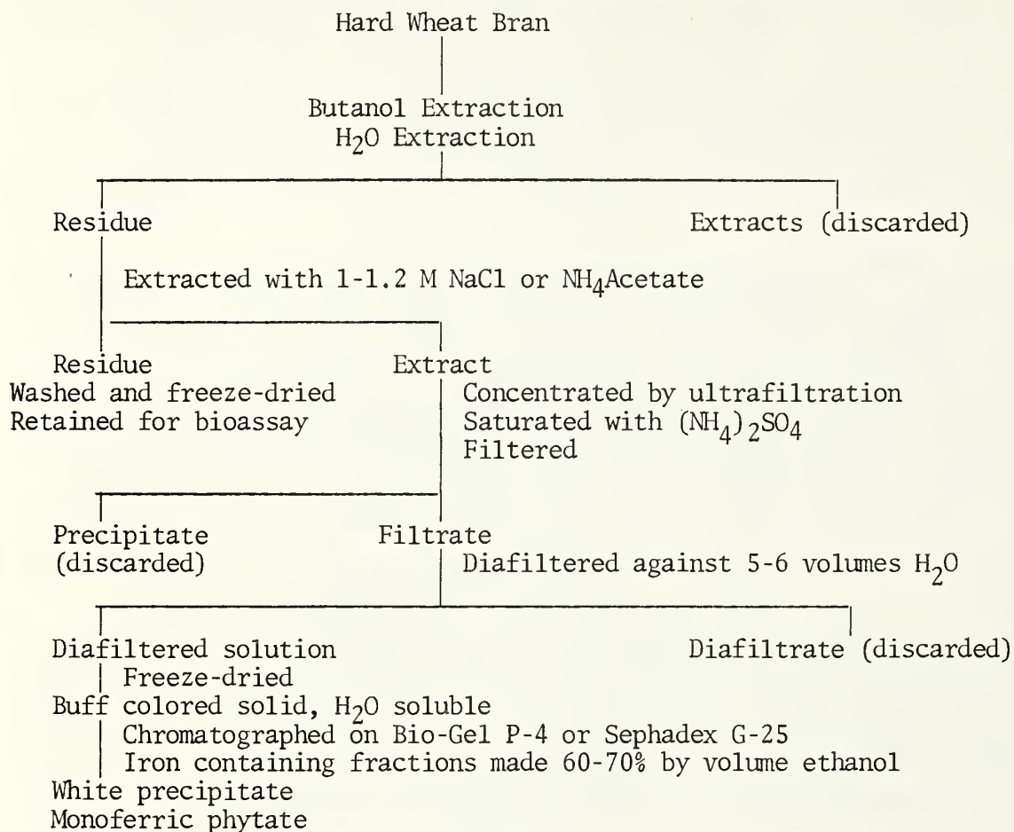
Figure 1. Isolation and purification of monoferric phytate from wheat bran.
