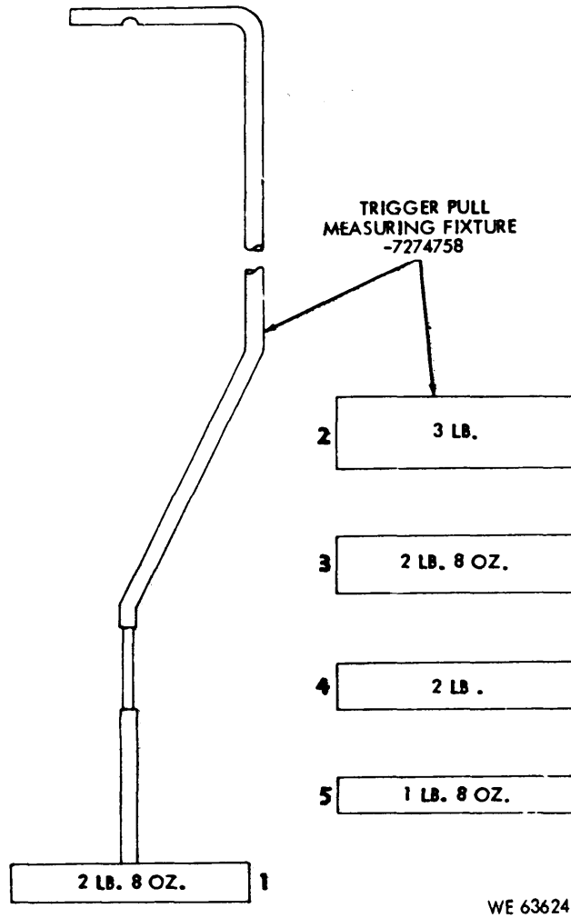
Figure 2-1. Trigger pull measuring fixture.
