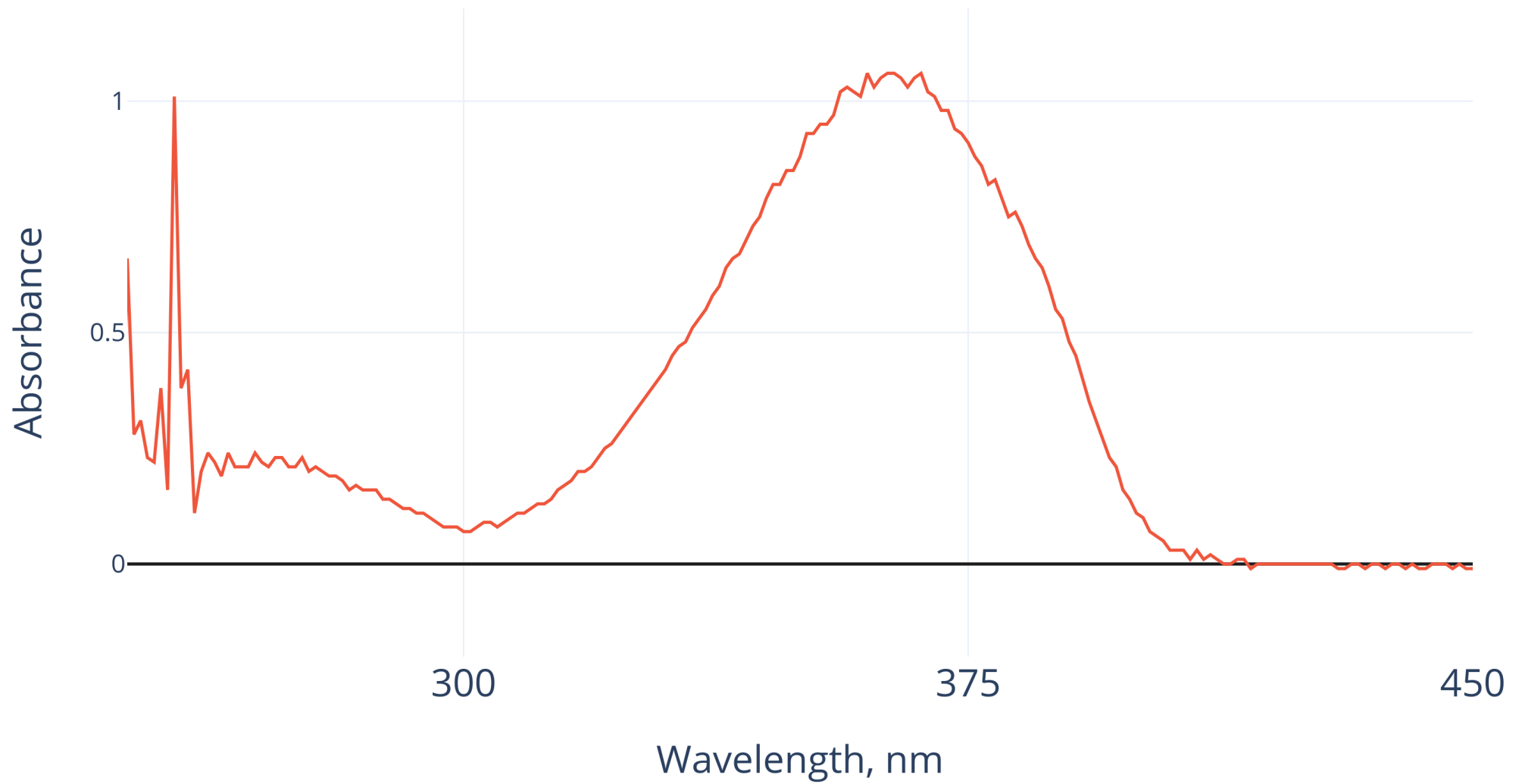
Absorbance of 0.01g/L avobenzene in dimethyl sulfoxide
