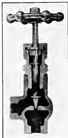
Fig. 56. The York Expansion Valve.
