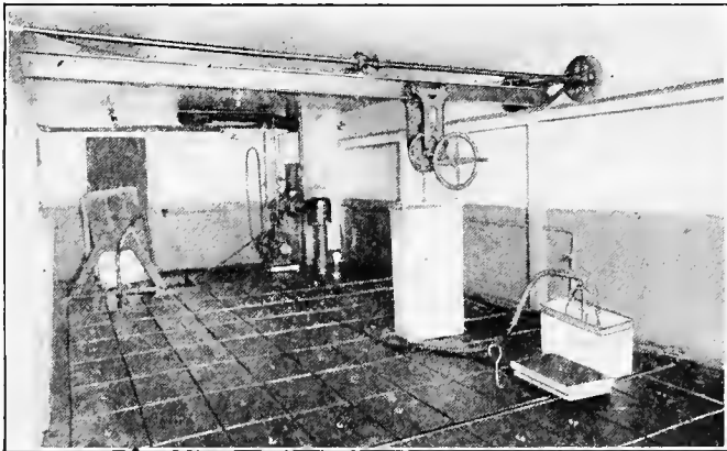
Fig. 60. Freezing Tank, Can Filler, Hoist, and Dump in an ice cream factory.
