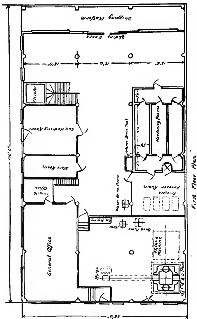
Fig. 63. First-floor Plan of a factory in which there is ample provision for future growth.
