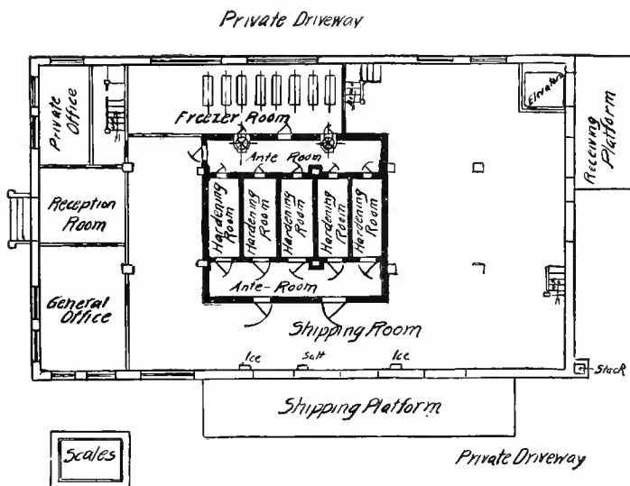
Fig. 61. First-floor Plan of a well-arranged factory.
