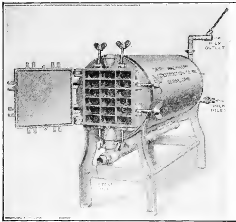
Fig. 16. The Progress Barrel Heater.
