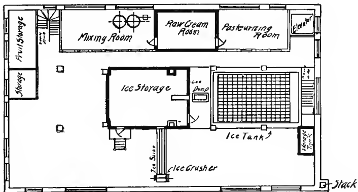
Fig. 62. Second-floor Plan of the same factory.
