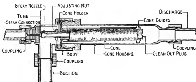
Fig. 89. A sectional view of Hawk's Emulser.
