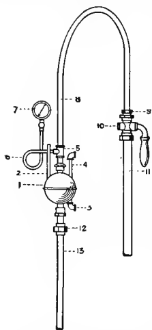
Fig. 90. The DeWitt & McCaddon Converter. (1) body of the converter; (2) \frac{3}{8} inch steam outlet; (3) \frac{1}{4} inch water inlet; (4) \frac{1}{4} inch water outlet; (5) \frac{1}{2} inch T; (6) \frac{1}{4} inch syphon; (7) steam gauge; (8) \frac{1}{2} inch discharge pipe; (9) 1 inch to \frac{1}{2} inch bushing; (10) 1 inch straight water cock; (11) 1 inch pipe; (12) \frac{3}{4} inch union; (13) \frac{3}{4} inch suction pipe.
