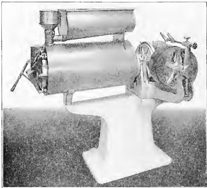
Fig. 74 The Ft. Atkinson Freezer.
