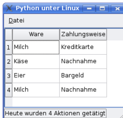
Abbildung 8: guiqt3.py Dialogfenster
