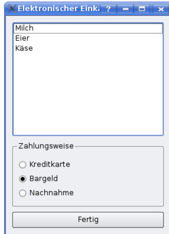
Abb. 9 guiqt3.py Dialogfenster
