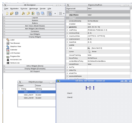
Abb. 11 Unser Dialogfenster
