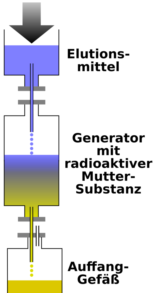
Abb. 94 Technetium-99m Generator
