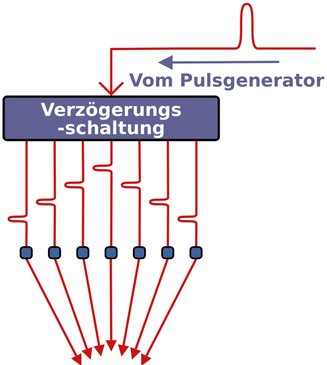
Abb. 165 Ultrasektorscanner / Phased Array Technik
