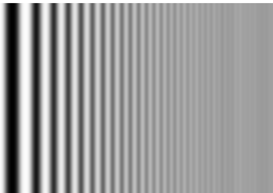
Abb. 139 reales abbildendes System
