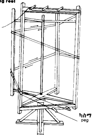
ግድራያ warping reel
