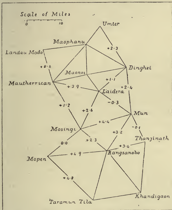
FIG. 77.—Re-triangulation of Khasi hills. (Oldham.)
