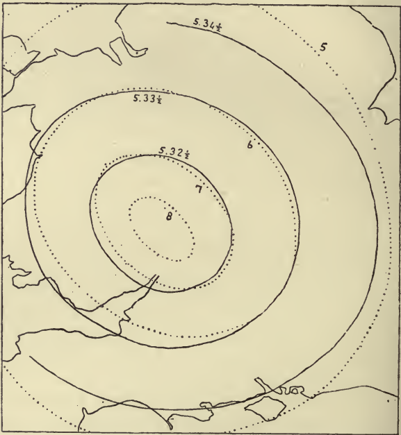
FIG. 62.—Coseismal lines of the Hereford earthquake. ( Davison. )
