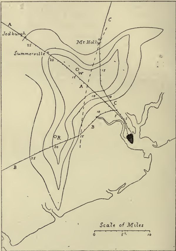
FIG. 28.—Epicentral isoseismal lines of Charleston earthquake according to Mr. Sloan. (Dutton.)
