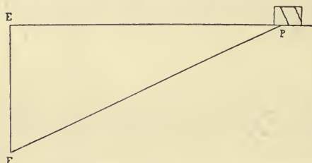
FIG. 11.—Diagram to illustrate Mallet's method of determining depth of seismic focus.
