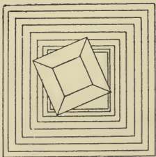
FIG. 74.—Twisting of monument at Chhatak. (Oldham.)
