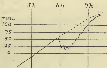
FIG. 38.—Record of tide-gauge at Nice. (Issel.)
