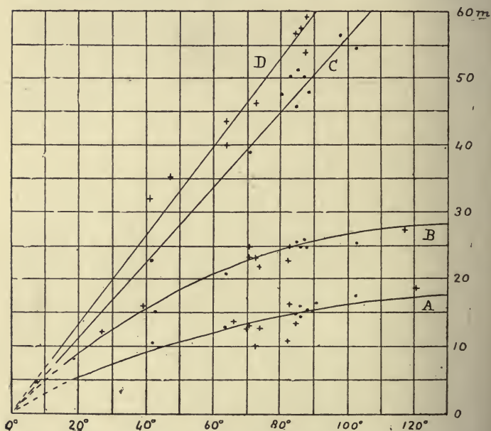
FIG. 80.—Time-curves of principal epochs of earthquake-waves of distant origin. (Oldham.)
