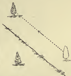
FIG. 50.—Shifting of Trees by Fault at Uméhara. (Koto.)
