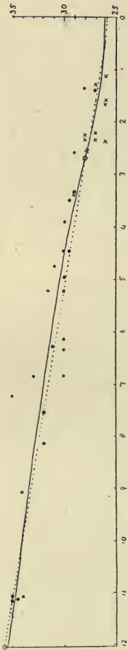
FIG. 70.—Time-curve of Indian earthquake. ( Oldham. )
