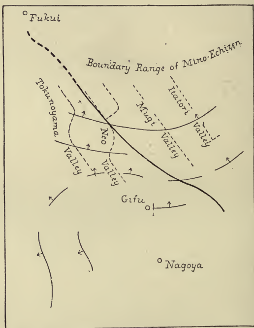
FIG. 42.—General Plan of Geological Structure of Meizoseismal Area. (Koto.)
