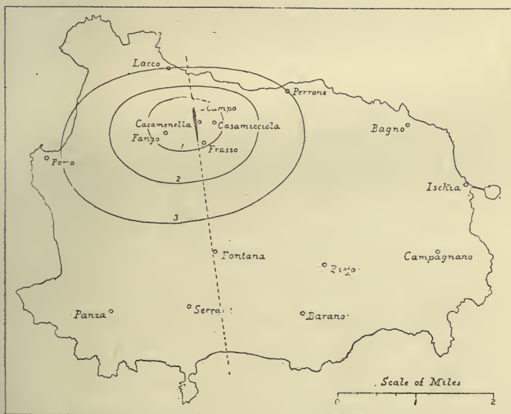
FIG. 15.—Isoseismal lines of the Ischian earthquake of 1881.
