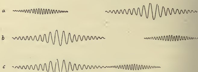
FIG. 61.—Nature of shock of Hereford earthquake.
