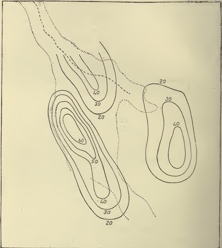
FIG. 58.—Distribution of Audible After-shocks in Space (November 1891–December 1892). (Davison.)
