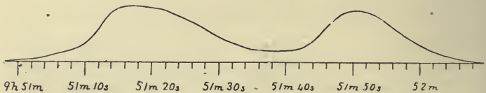
FIG. 26.—Curve of intensity at Charleston. ( Dutton. )
