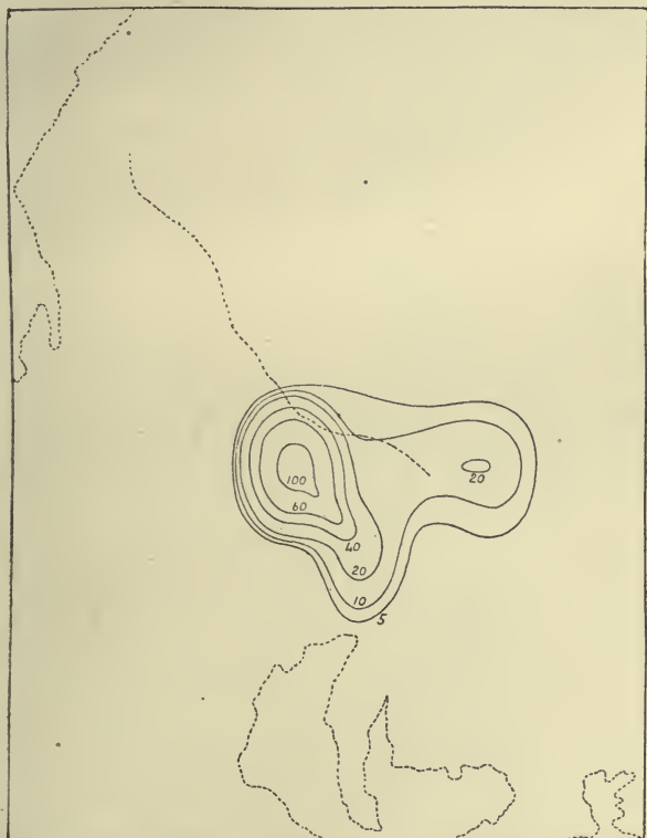
FIG. 56.—Distribution of After-shocks in Space (March-April). ( Davison. )
