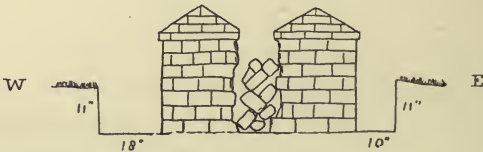
FIG. 69.—Section of Tombs in the Cemetery at Cherrapunji. (Oldham.)
