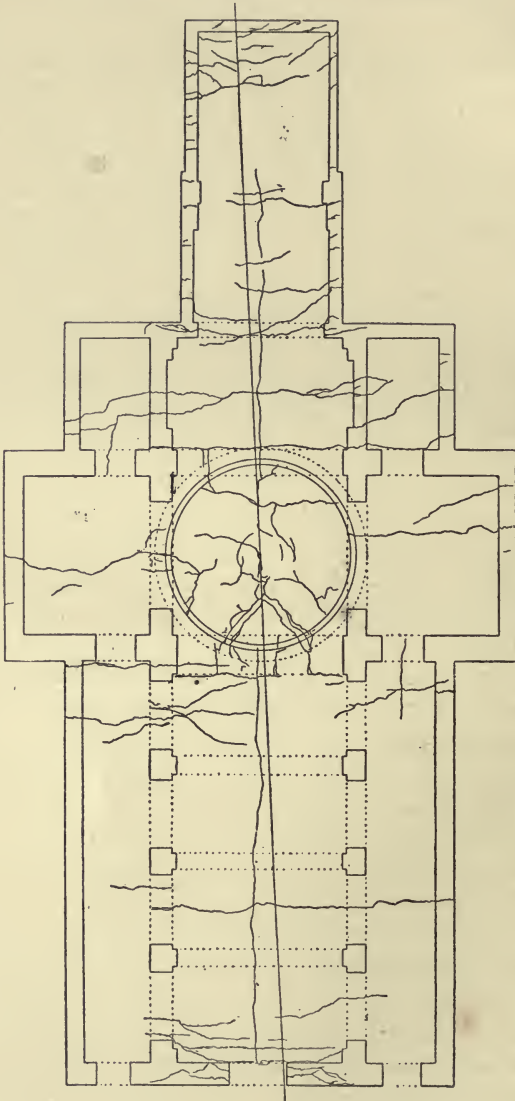
FIG. 5.—Plan of Cathedral Church at Potenza. ( Mallet. )
