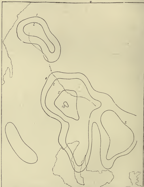
FIG. 53.—Distribution of preliminary Shocks in Space. ( Davison. )
