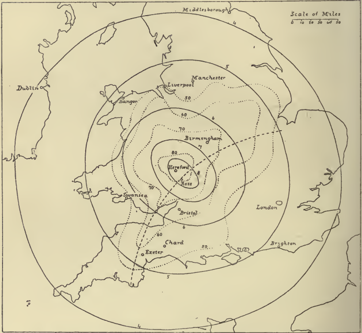
FIG. 60.—Iseisimal and Isacoustic lines of Hereford earthquake. (Davison.)
