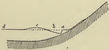
FIG. 73.—Displacement of alluvium at foot of a hill. (Oldham.)
