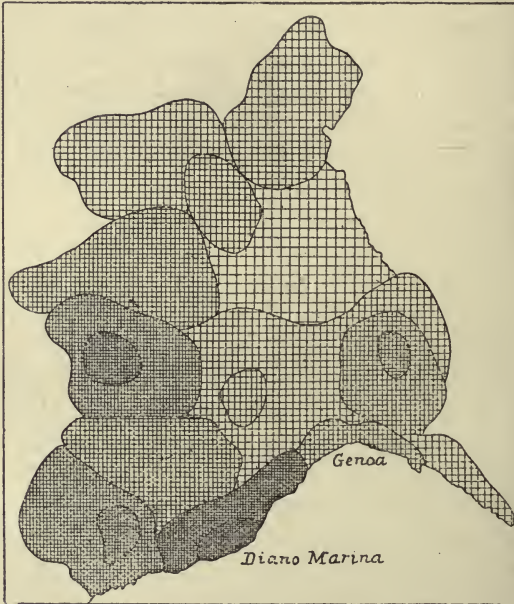
FIG. 40.—Distribution of seismic activity in the Riviera. (Mercalli.)
