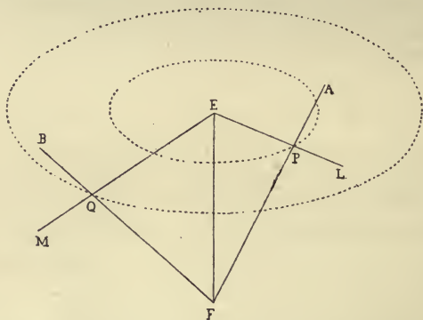
FIG. 3.—Diagram to illustrate wave-path and angle of emergence.
