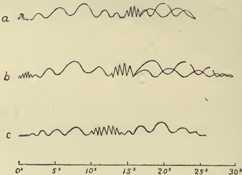
FIG. 35.—Nature of shock of Riviera earthquake. ( Taramelli and Mercalli. )
