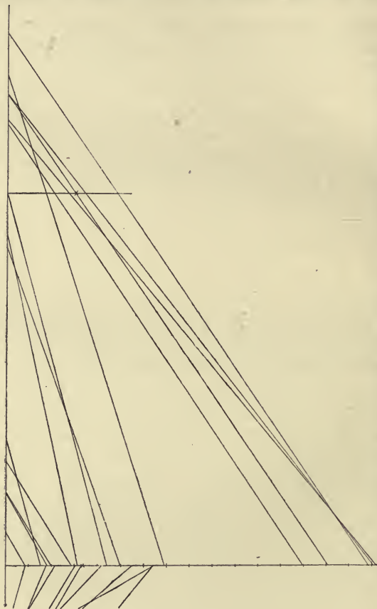
FIG. 17.—Diagram of wave-paths at seismic vertical of Ischian earthquake of 1883. ( Johnston-Lavis. )
