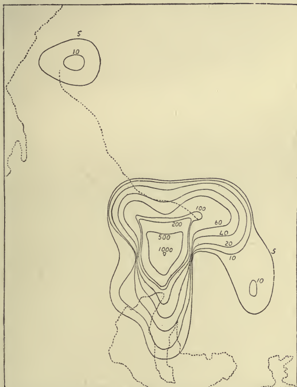
FIG. 54.—Distribution of After-shocks in Space (November-December 1891). (Davison).
