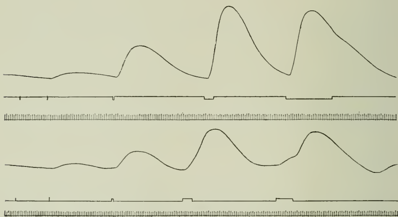
FIGURE 10. — In the upper line, the effect of the make followed by the break, with intervals of \frac{1}{20} , \frac{1}{5} , 1, 5, and 25 seconds: below, the effect of the break followed by the make, intervals of \frac{1}{20} , \frac{1}{5} , 1, 5, and 10 seconds, the current flowing meanwhile. Time in seconds. Original size.
