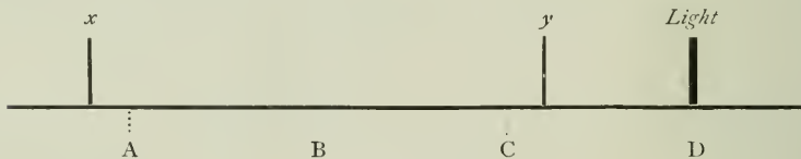
FIGURE 4.— x, y , ends of trough; A, point at which animal started; C, point at which trip was finished; distance A C = 50 cm.; distance A B and B C each 25 cm.; distance of light from starting point (A D) 75 cm.
