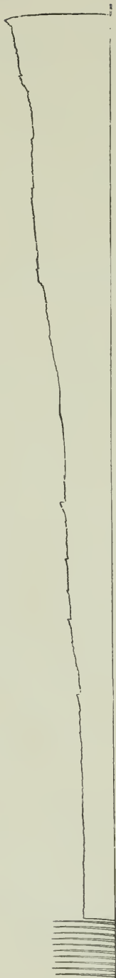
FIGURE 8. — Voluntary tetanus. Spring, 4 mm. = 1 kg., original magnification of movement, 2. Tracing here reduced to two-fifths the original size.
