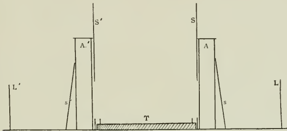
FIGURE 5. — Heliotropic apparatus, one-sixth actual size. T, tin trough; S, S', screens with rectangular openings for light; A, A', vessels of alum solution; s , s' , cardboard screens; L, L', Welsbach burners.
