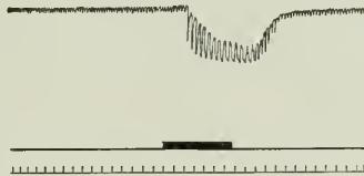
FIGURE 3.—October 21, 1899. Original size. The uppermost line is the curve of blood-pressure in the carotid artery registered by a Hürthle membrane manometer. The middle line is atmospheric pressure; this line was drawn by the writing point of an electro-magnetic signal, which recorded with a broad black line the duration of depressor stimulation. The lowest line marks the time in seconds. Both splanchnic nerves were severed. The blood-pressure was raised after this section by the injection of 0.8 per cent NaCl solution into the jugular vein. On simultaneous stimulation of both depressor nerves the blood-pressure fell from 90 mm. to 57 mm. (37 per cent).
