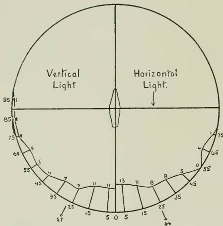
FIGURE 2. — Distribution of points at which planarians with eyes passed over the circumference of the circle, (1) when affected by horizontal light and directed away from its source (right half of figure), and (2) when under vertical light and directed toward 0^\circ (left half). For further explanation see page 379.
