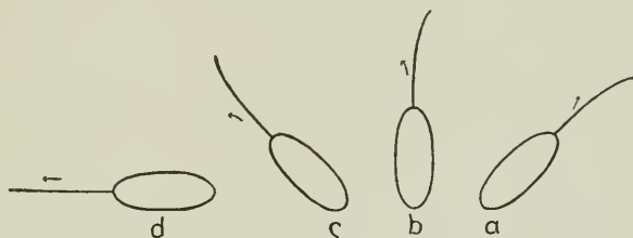
FIGURE 3.—Phototactic movements of a flagellated organism, according to VERWORN. (From VERWORN: Loc. cit. , 1899, p. 500.)
