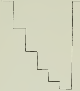
FIGURE 15. — Record showing the relative extension of the muscle under additional weights of 20, 40, 60, 80, and 100 grams. Drum turned by hand. One-half the original size.
