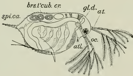
FIGURE 1. — Daphnia pulex DeGeer. \times 13 . at. antenna; atl. antennule; gl. d. dorsal gland; cr. heart; brs. 'cub. brood pouch; spi. ca. caudal spine; oc. eye.
