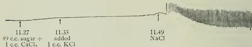
FIGURE 7. — At 10.37 a strip of heart muscle was placed in a solution of cane sugar, but it failed to beat; it was transferred to 49 c.c. sugar + 1 c.c. \text{CaCl}_2 solution at 11.27, and at 11.35 1 c.c. KCl solution was added without beats appearing. At 11.49 it was put into NaCl solution, and 30 seconds later beats appeared.
