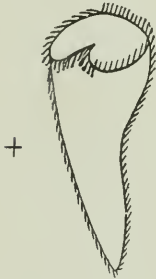
FIG. 7. — Diagram showing the relation of the adoral cilia in Stentor when the animal is at right angles to the current.
