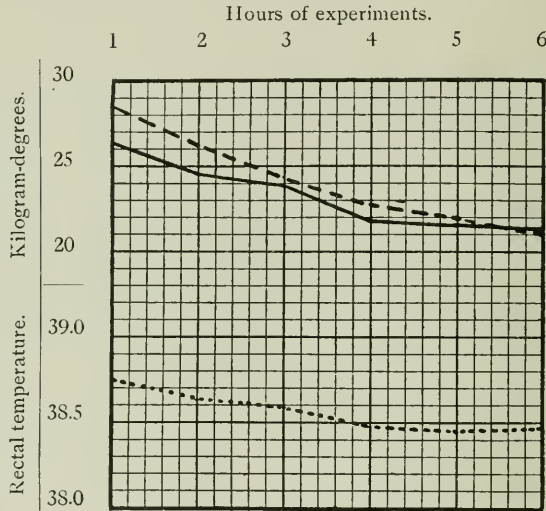
FIGURE 1. — Curves of heat production (—), heat dissipation (— — —), and body temperature (.....) in normal fasting animals.
