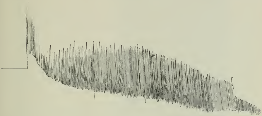
FIGURE 2. — A strip of ventricle put into a solution of cane sugar at 10.20 A.M. did not contract. At 11.35 it was transferred to a 0.7 per cent sodium chloride solution, when beats began instantly.
