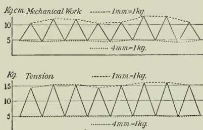
FIGURE 6. — Alternate contractions with different springs. 10 seconds interval between contractions. The successive contractions are joined by unbroken lines. This figure represents the results in Table VI.
