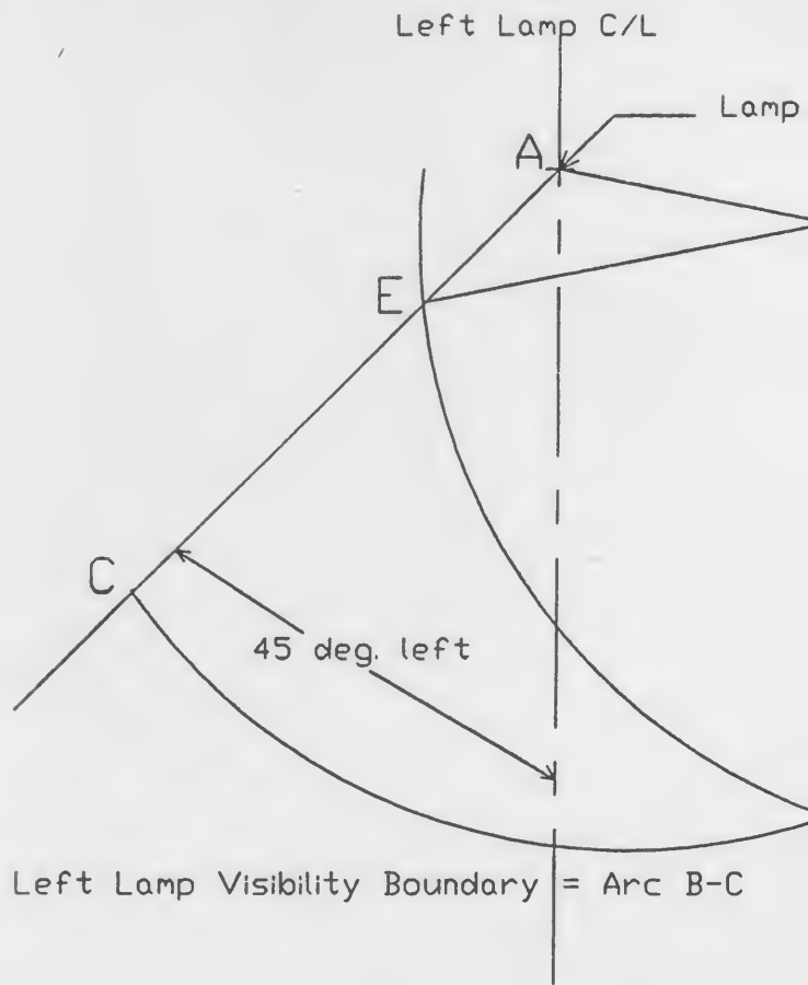
FIGURE 2 - PLAN VIEW, SIGN
