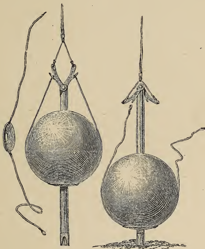
BROOKE'S SOUNDING APPARATUS.
