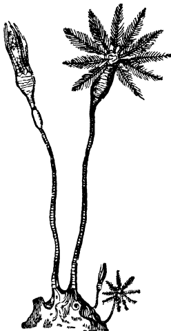
Fig. 72.— Apiocrinus rotunda .
