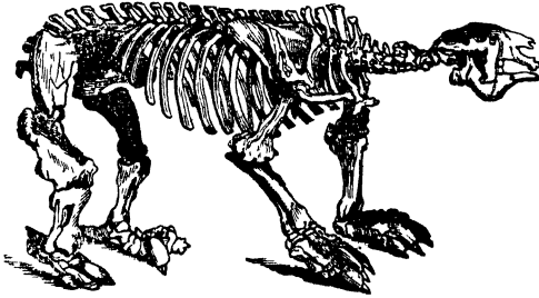
Fig. 390.—The Megatherium .
