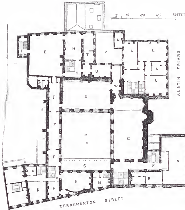
DRAPERS' HALL.—PLAN OF FIRST FLOOR.
