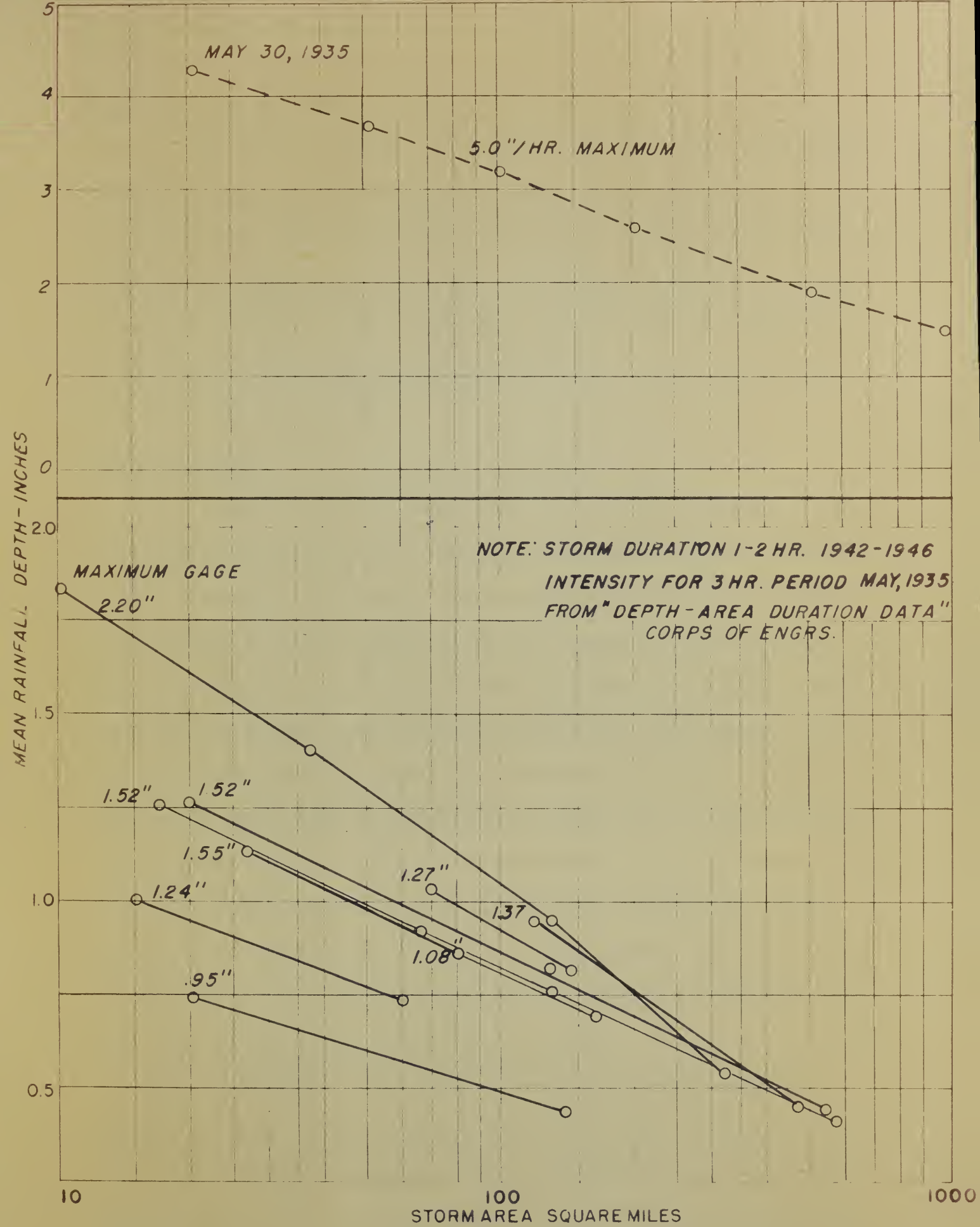
FIGURE 10 DEPTH VS AREA
