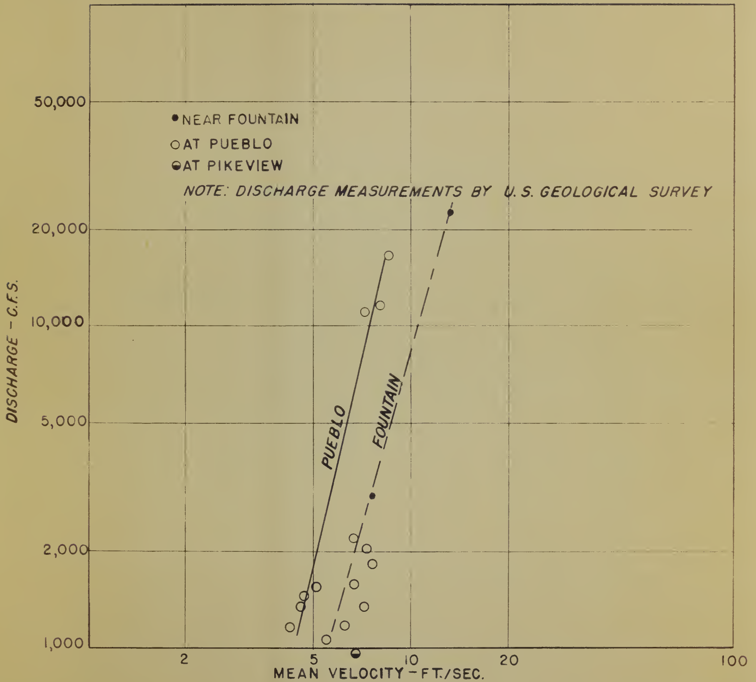
FIGURE 3 VELOCITY VS DISCHARGE
