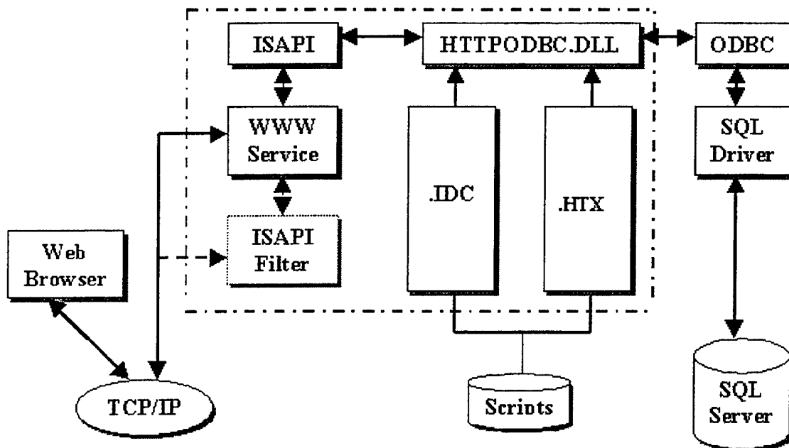
Figure 3.7 IDC to Access the Internet Information Server Log File, Stored in the SQL Server Database
