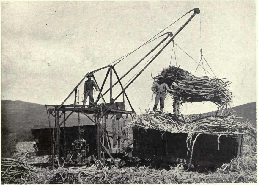
THE WHEELER-WILSON CANE LOADER.
