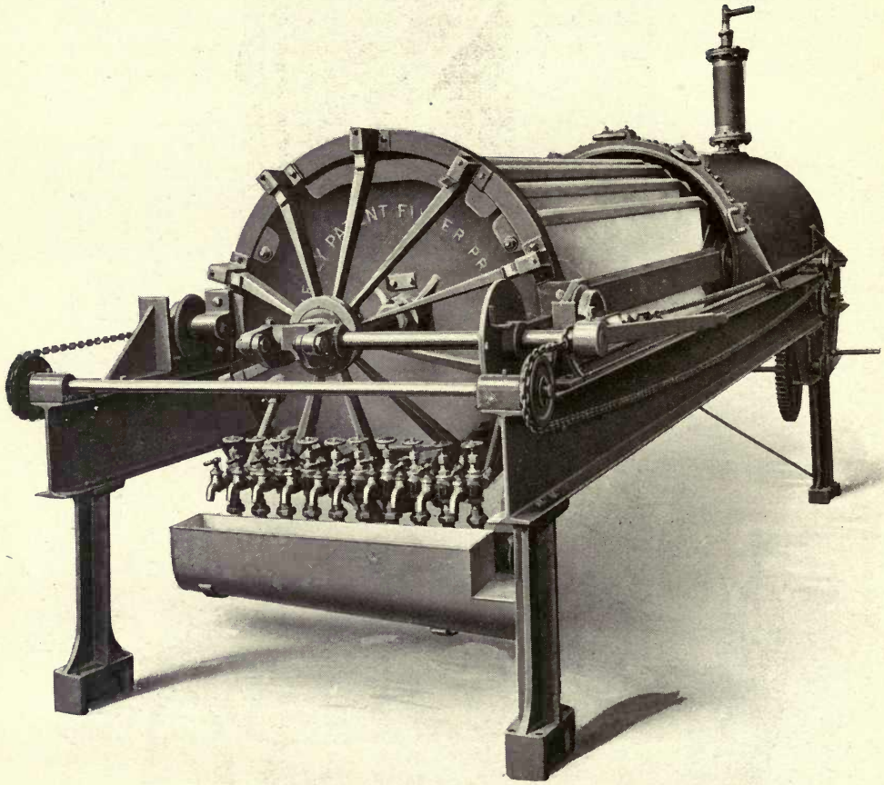
THE KELLY FILTER PRESS.
