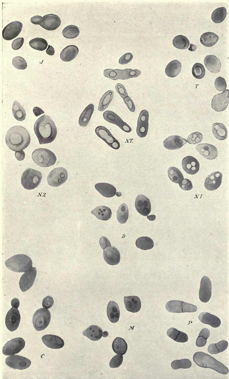
APPEARANCE OF YEASTS FROM VARIOUS COUNTRIES WHERE MOLASSES IS FERMENTED.
