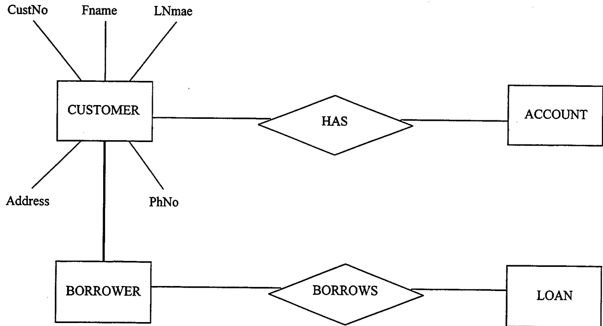
Figure 5.7. Integrated Schema.
