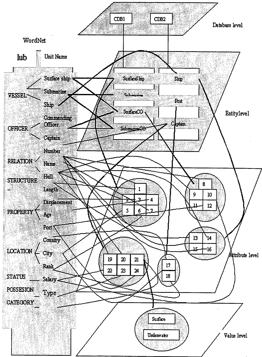
Figure 5.16. Semantic Network.
