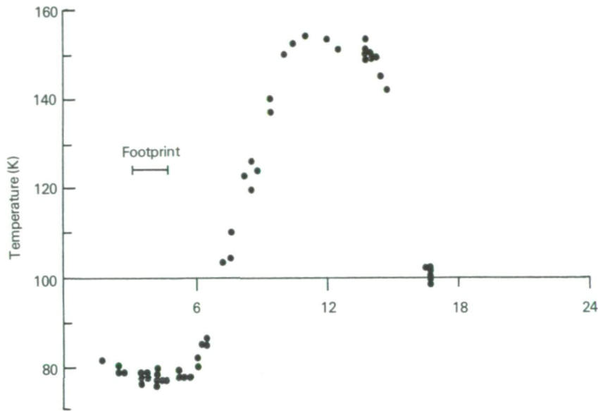
The IRIS instrument measured the temperature of spots on the surface of Callisto as each Voyager sped past. The measurements shown here were all made at equatorial latitudes (between -10^\circ and 25^\circ ). Shown are very low predawn temperatures ( -190^\circ\text{C} ) followed by an increase to a noon-time maximum of about -120^\circ\text{C} , and then a drop again as the Sun sets. [260-735]
