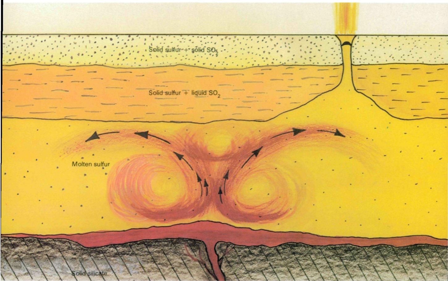
One model for the structure of Io indicates that an ocean of liquid sulfur with a solid sulfur crust covers most of the satellite. Heat escapes from the interior in the form of lava, which erupts beneath the sulfur ocean. Secondary eruptions in the sulfur ocean heat liquid sulfur dioxide, which is mixed with solid sulfur in the crust. The rapid expansion of sulfur dioxide gas then produces the great eruptive plumes, which consist of a mixture of solid sulfur, sulfur dioxide gas, and sulfur dioxide snow.
