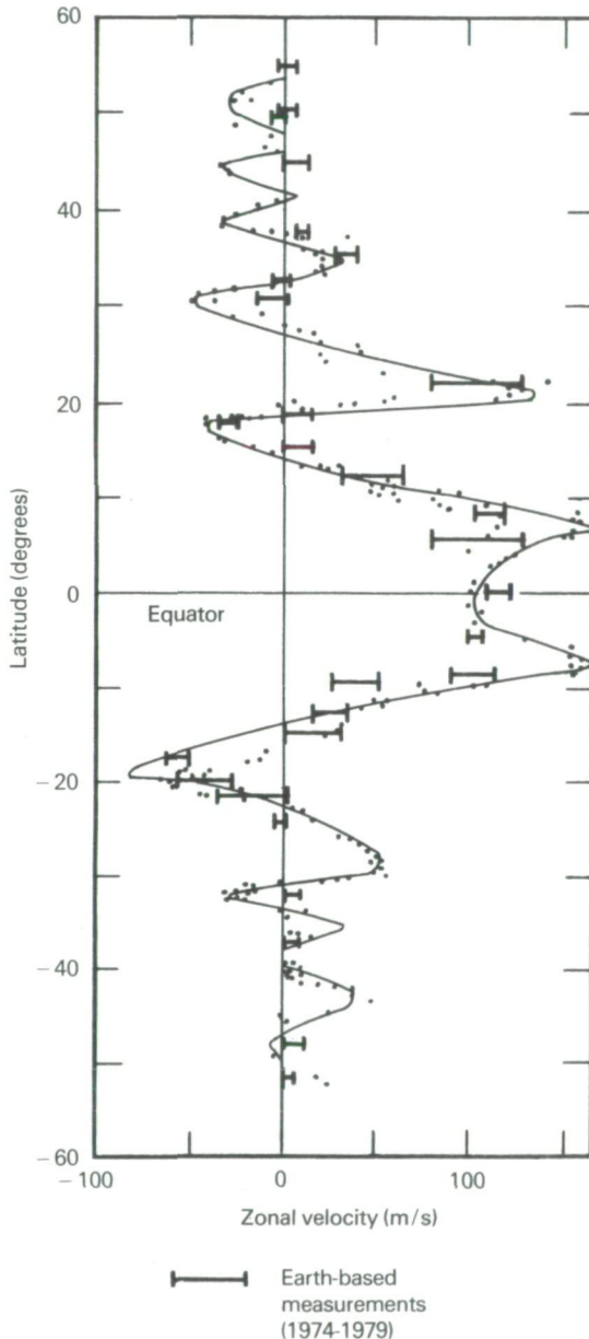
At different latitudes, the strong prevailing zonal winds produce different apparent rotation rates. Plotted here are the horizontal velocities measured from a pair of Voyager images taken one rotation (about ten hours) apart. Also shown for comparison are older ground-based measurements obtained from careful timings of the apparent rotation rate at different latitudes. The excellent agreement of the two plots indicates the stability of the zonal winds. Also, the wind pattern shows much greater symmetry between northern and southern hemispheres than do the more superficial cloud patterns.
