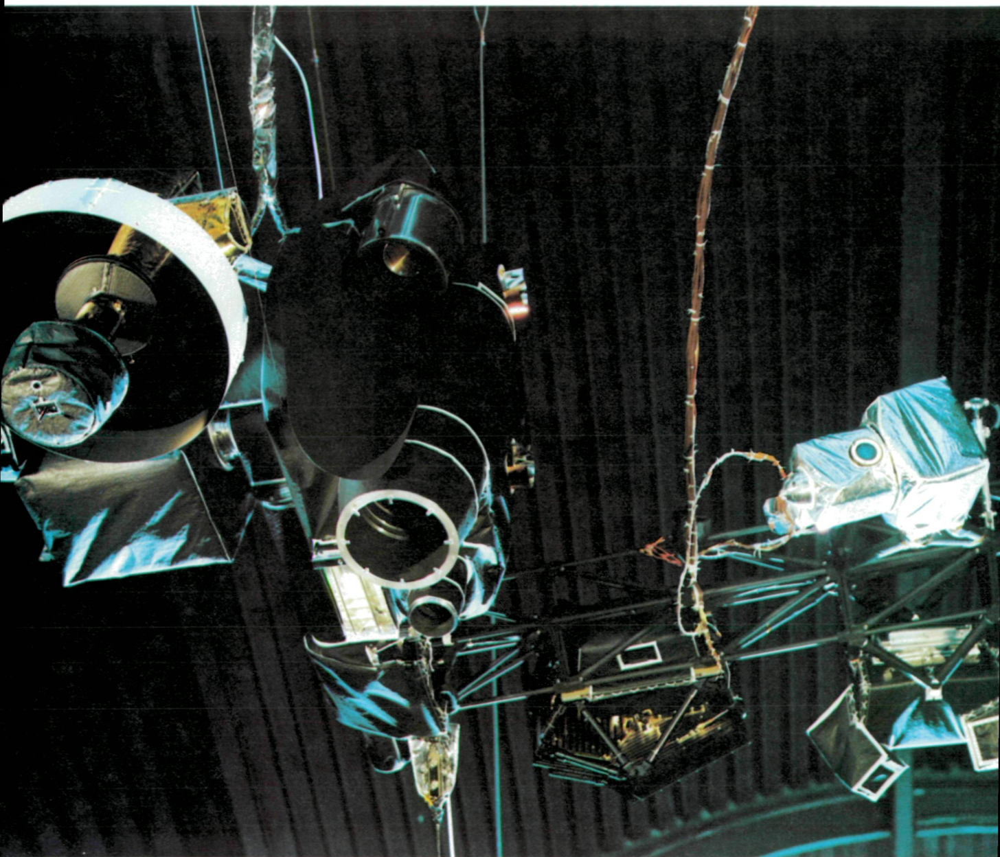
The Voyager scan platform contains sophisticated instruments that gather data for Voyager's remote sensing investigations. Five of the remote-sensing instruments—two TV cameras, the infrared spectrometer, the ultraviolet spectrometer, and the photopolarimeter—are mounted together on the scan platform, which can be pointed to almost any direction in space, allowing exact targeting of the observations. [373-7146BC]
