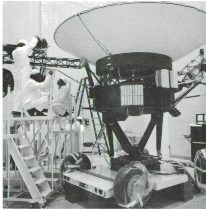
During the early assembly stage, technicians at Caltech's Jet Propulsion Laboratory equip Voyager's extendable boom with low- and high-field magnetometers that measure the intensity and direction of the outer planets' magnetic fields. [373-7179BC]
