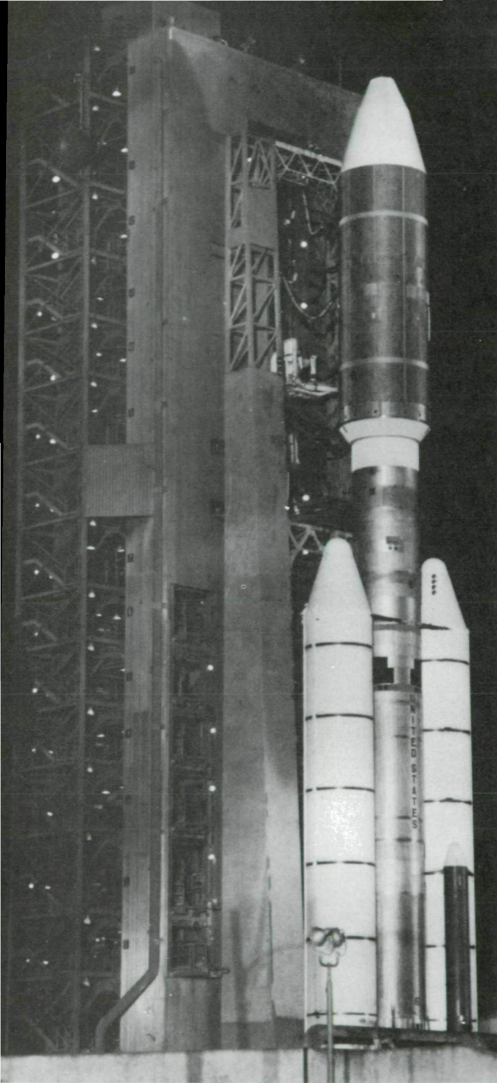
The Titan/Centaur rocket used to launch Voyager stood as tall as a 15-story building and weighed nearly 700 tons. Here the rocket waits for launch at Kennedy Space Center, with the Voyager spacecraft enclosed in the white protective shroud at the top. [P-19471A]
