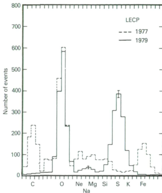
Direct measurement of the heavy ions associated with the Io torus were made by the Voyager 1 LECIP instrument. Here the amounts of various elements are shown for two cases: the Jovian inner magnetosphere (solid line) and a typical solar event. Both the Jovian and the solar particles have been scaled to show similar amounts of oxygen, but the solar particles are also rich in carbon and iron, whereas Jupiter has a great deal of sulfur. Evidence such as this demonstrates that the sulfur does not come from the Sun; rather, the sulfur and most of the oxygen appear to be the product of the Io sulfur dioxide volcanic eruptions.
