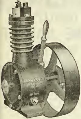
No. 101 Belt Driven Compressor.
