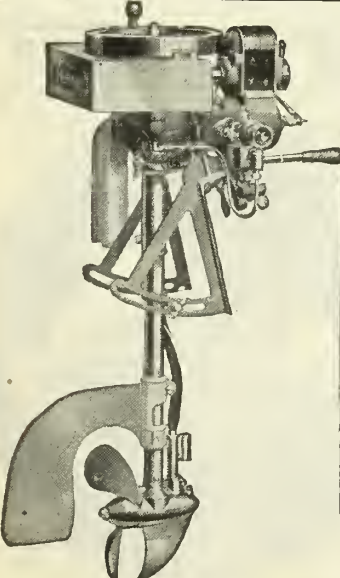
THE FERRO ROW BOAT MOTOR
