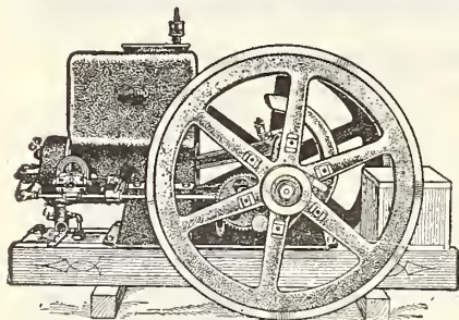
Field Type "W" 1 1/2 H. P.
