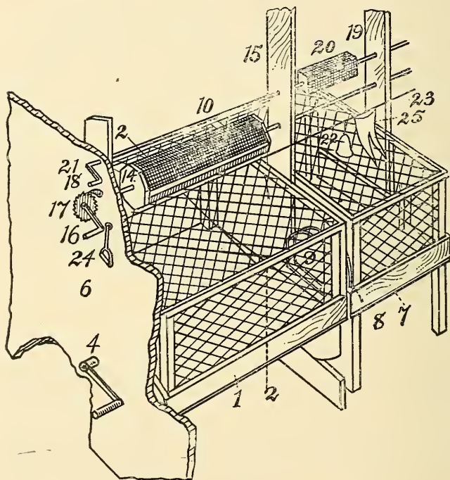
FIG. 71. DETAILS OF TILT BOX.
