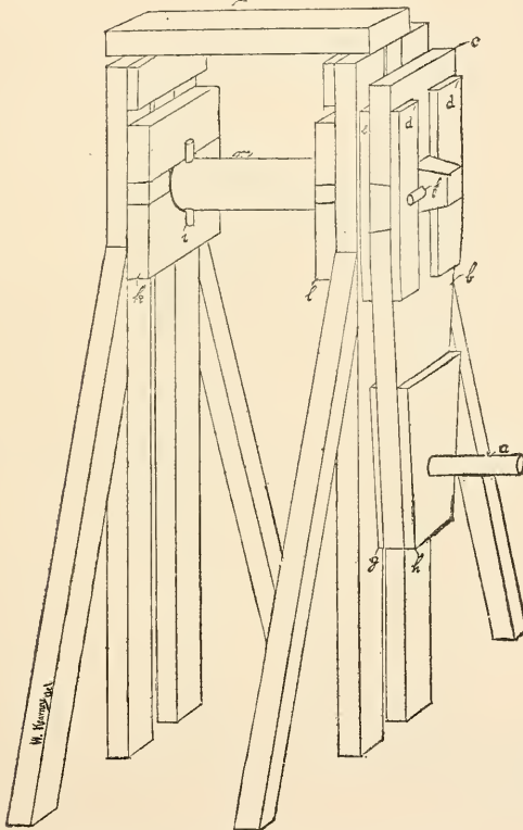
FIG. 99. WOODEN SPOOL, FRAME, ETC.
