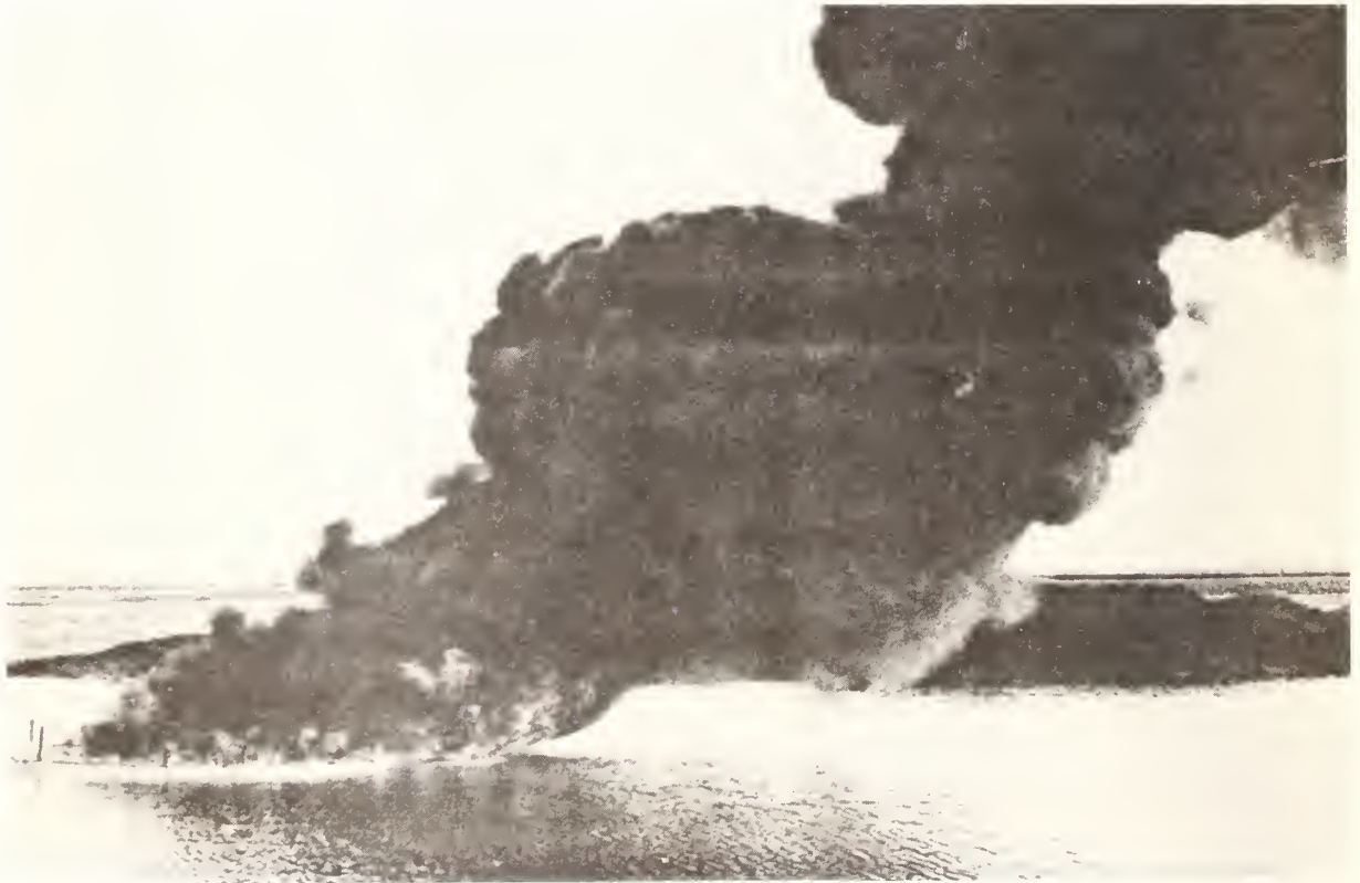
Figure 13 Large scale burn tests near Prudhoe Bay, Alaska [4]
