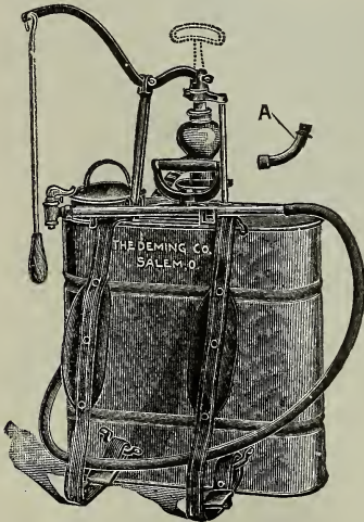
"Success" Sprayer.
