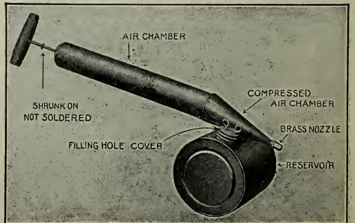
"U. T. K." Compressed Air Sprayer.
