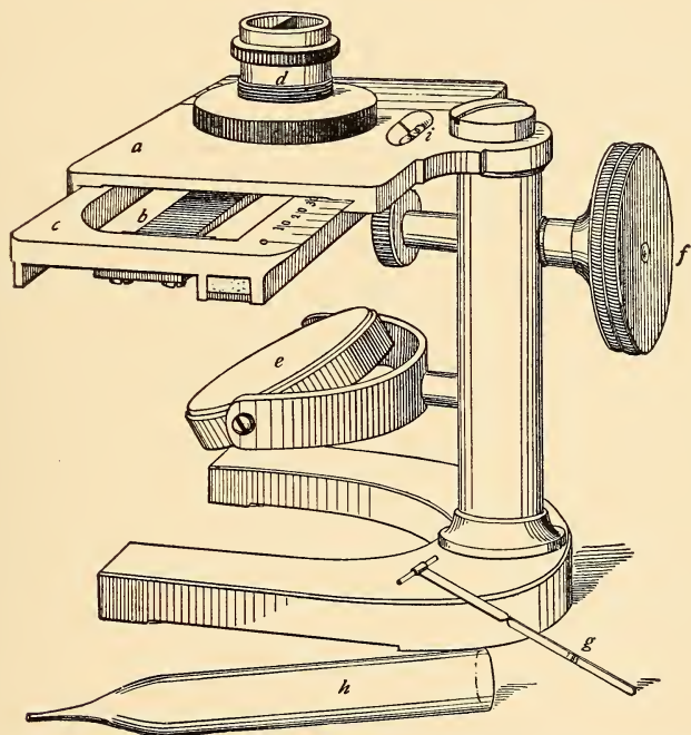
FIG. 118. —Von Fleischl's hemometer: a , stand; b , narrow wedge-shaped piece of colored glass fitted into a frame ( c ) which passes under the chamber; d , hollow metal cylinder, divided into two compartments, which holds the blood and water; e , white plate from which the light is reflected through the chamber; f , screw by which the frame containing the colored glass is moved; g , capillary tube to collect the blood; h , pipette for adding the water; i , opening through which may be seen the scale indicating percentage of hemoglobin.
