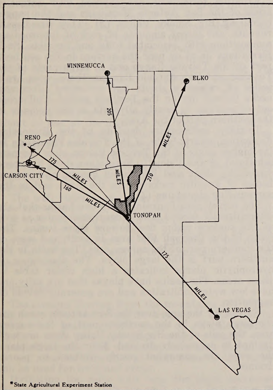
Figure 1. —Location of the Big Smoky Valley Area (part of Nye County) in Nevada.
