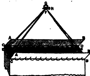
BALL'S DREDGE.
