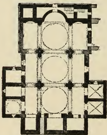
Fig. 248. Molfetta Cathedral.
