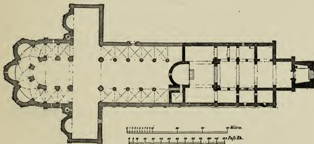
Fig. 264. Venosa. The Two Cathedrals.
