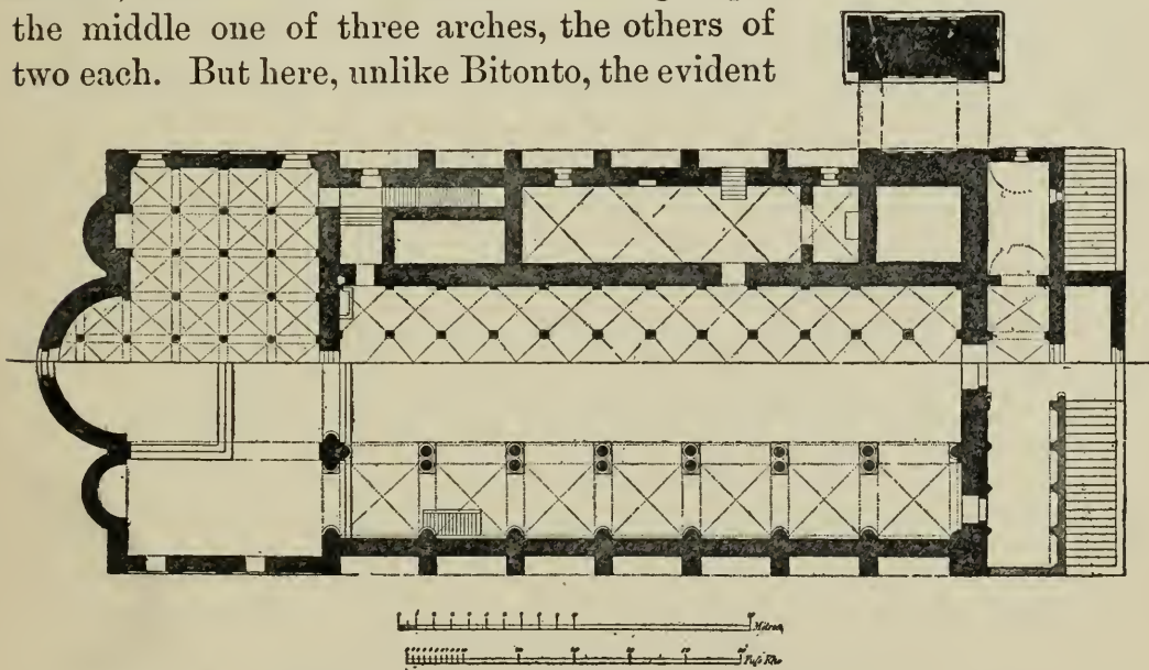
Fig. 260. Trani. Plan of Cathedral and Crypt.
