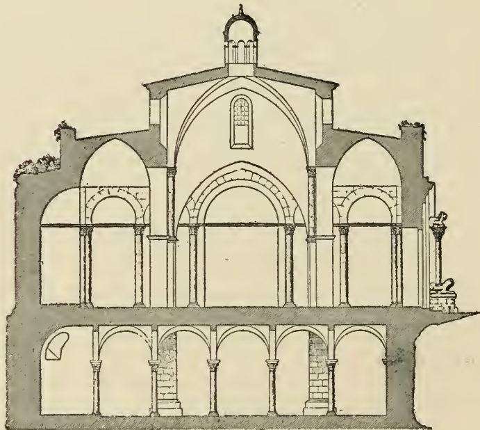
Fig. 257. Siponto. Section of Cathedral.
