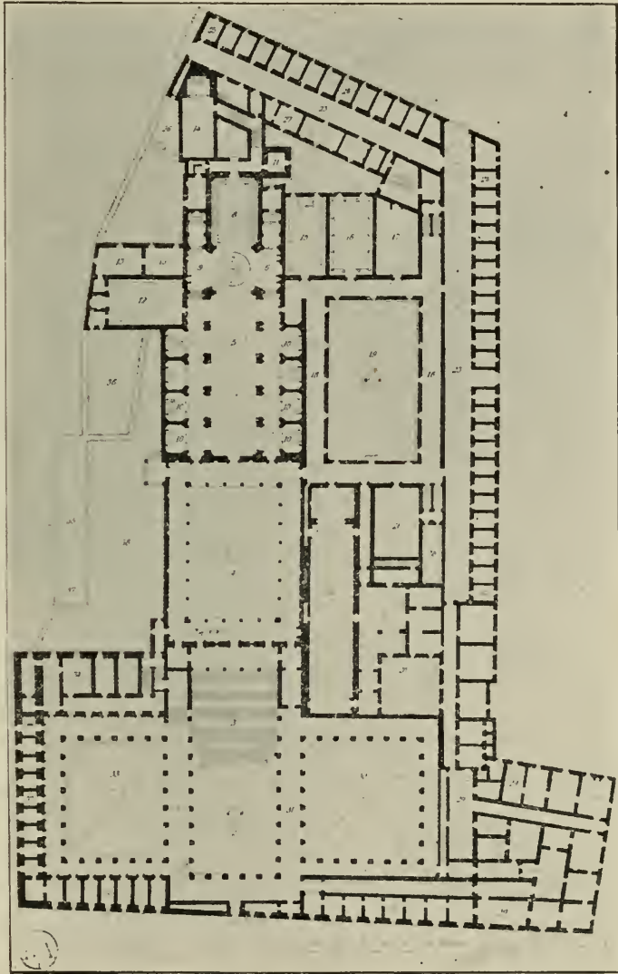
Fig. 326. Plan of Monte Cassino. Present Monastery.
