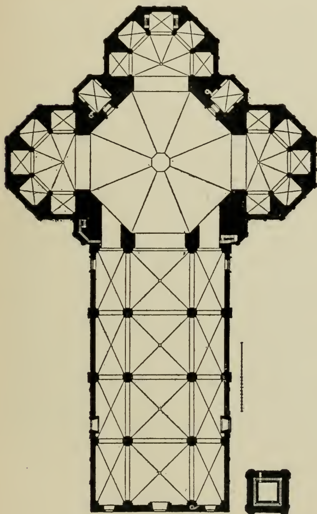
Fig. 373. Florence. Cathedral.
