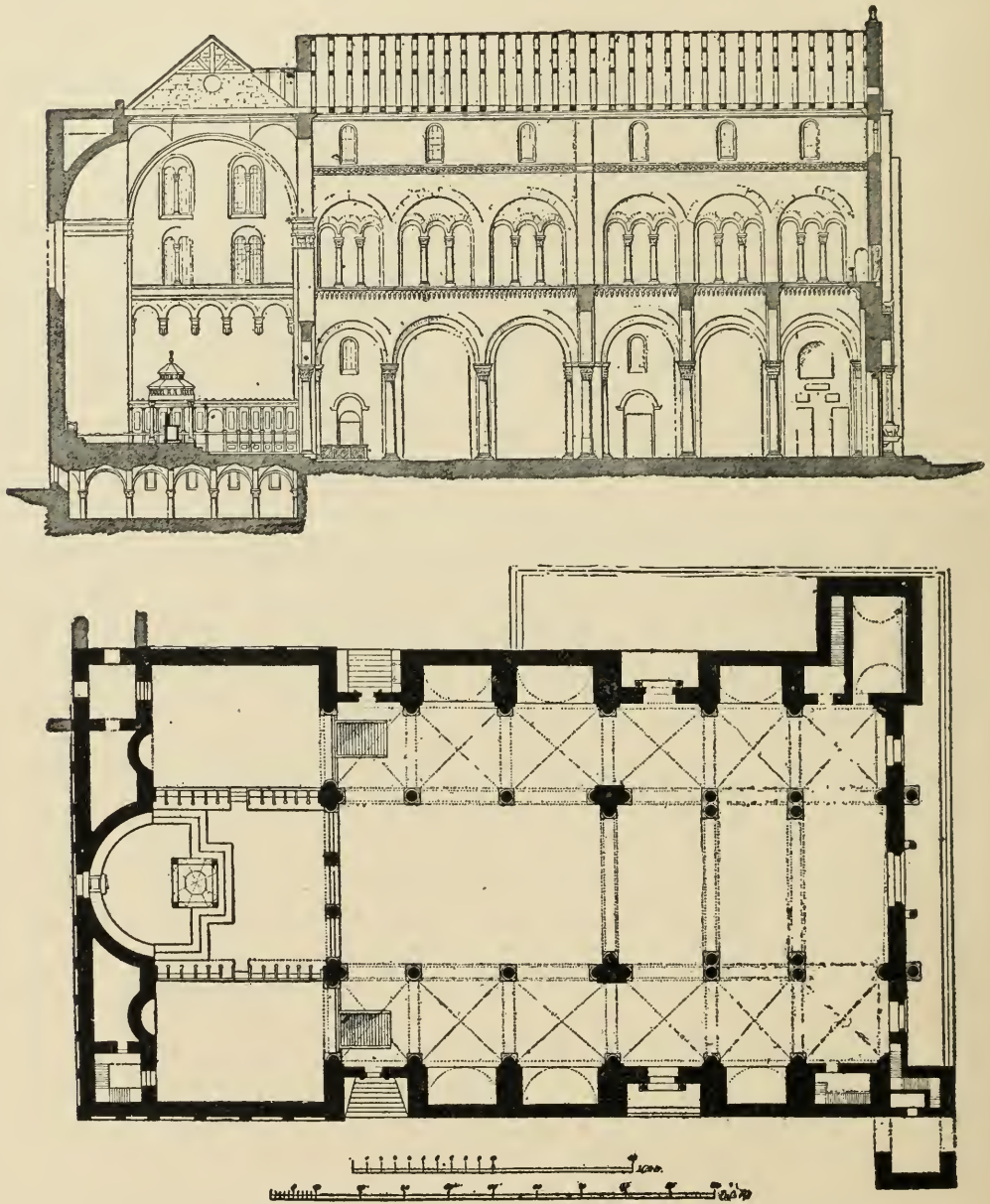
Fig. 242. Bari. S. Nicola. Plan and Section.
