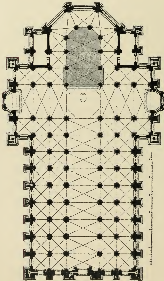
Fig. 381. Milan. Cathedral.
