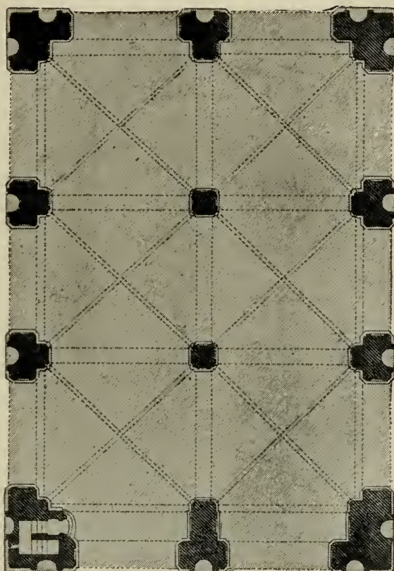
Fig. 451. Plan of Or San Michele.
