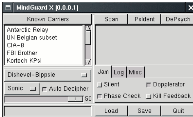
Software MindGuard(TM).
