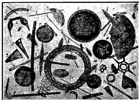
硅藻沈澱
