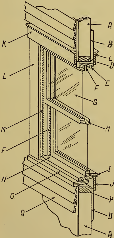
FIG. 153.—CROSS SECTION OF A WINDOW FRAME.
