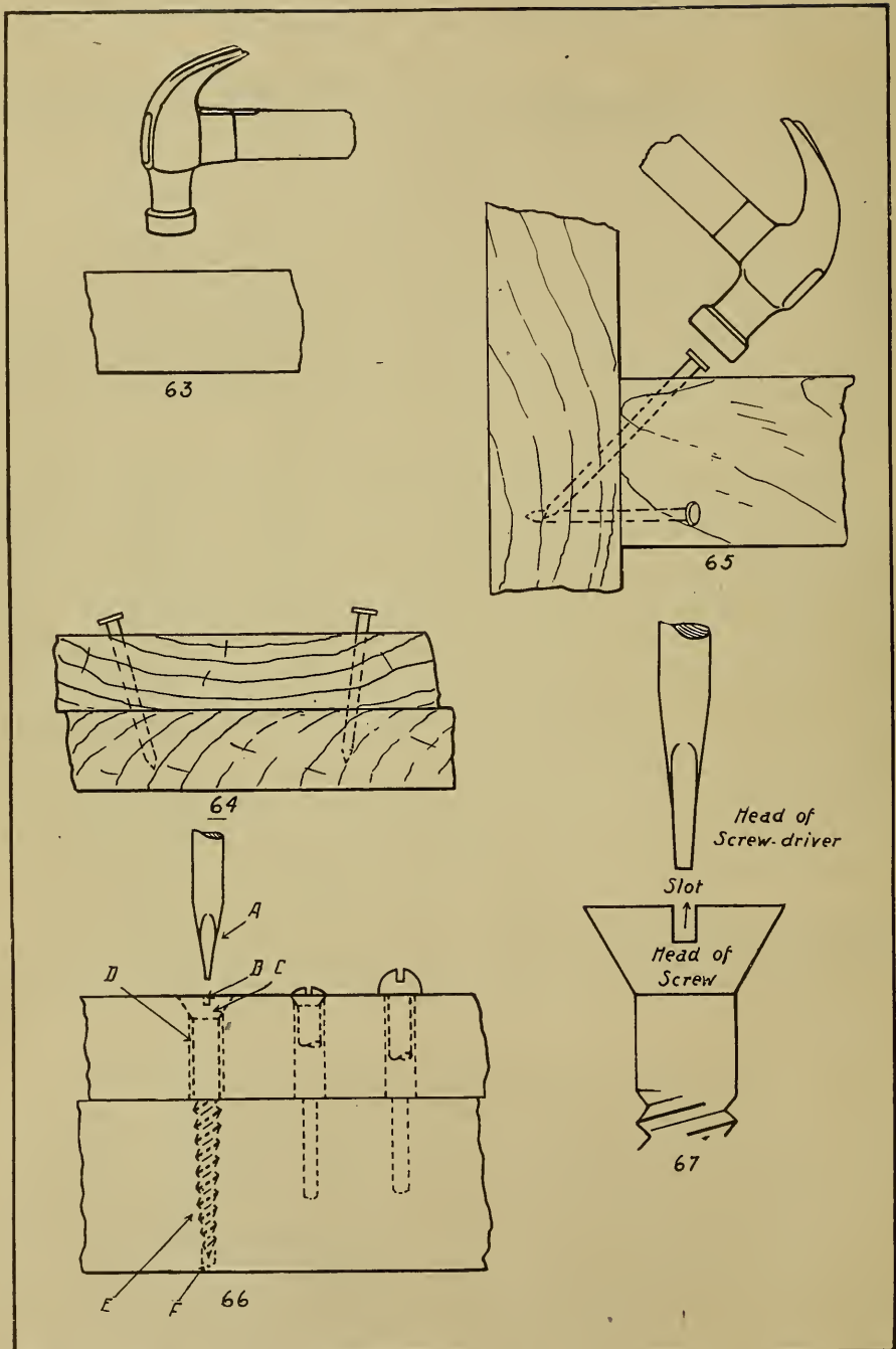
FIG. 63.—HAMMER POSITION. FIG. 64.—METHOD OF NAILING. FIG. 65.—TOE-NAILING. FIG. 66.—DRIVING SCREWS. FIG. 67.—ADJUSTMENT OF SCREW AND DRIVER.
