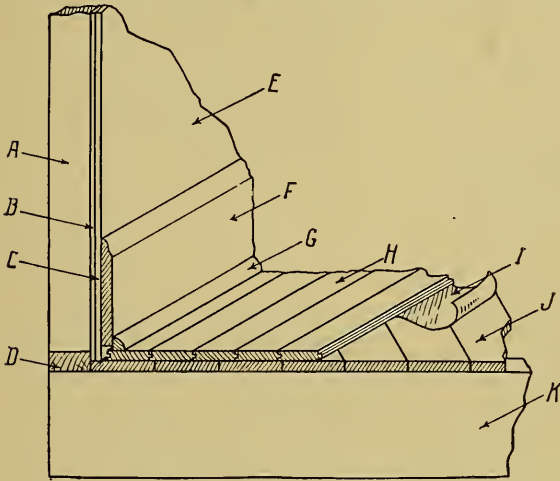
FIG. 155.—LAYING THE FLOOR.
