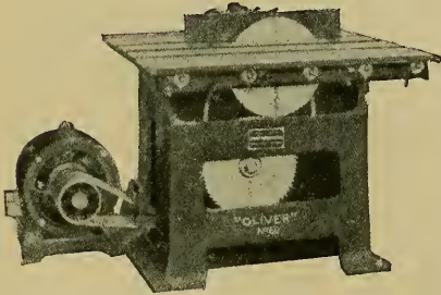
FIG. 100.—UNIVERSAL SAW BENCH.
