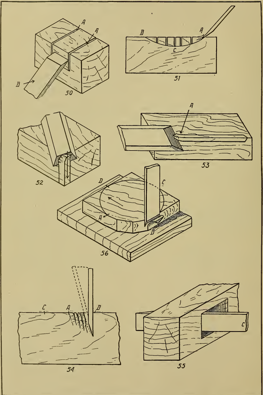
FIG. 50.—HALVING JOINTS. FIG. 51.—CUTTING CONCAVE SURFACE. FIG. 52.—CUTTING END BEVEL. FIG. 53.—CUTTING EDGE BEVEL. FIG. 54.—CUTTING MORTISE. FIG. 55.—TESTING MORTISE. FIG. 56.—CUTTING CIRCULAR PIECE.
