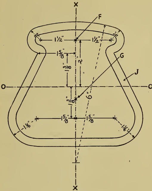
FIG. 91.—THE BACK.
