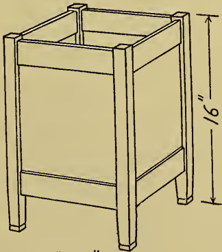
Top 12"X12" Base 12"X12"
