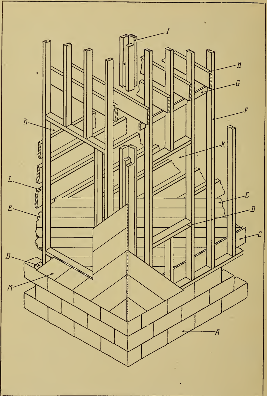
FIG. 150.—FRAME OF HOUSE (WITH T-SILL).
