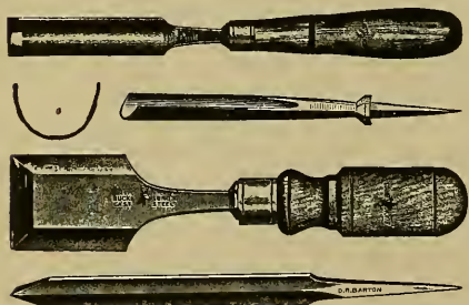
FIG. 49.—SPECIAL CHISEL TYPES. GOUGE, CARVING TOOL, BUTT CHISEL, CORNER CHISEL.
