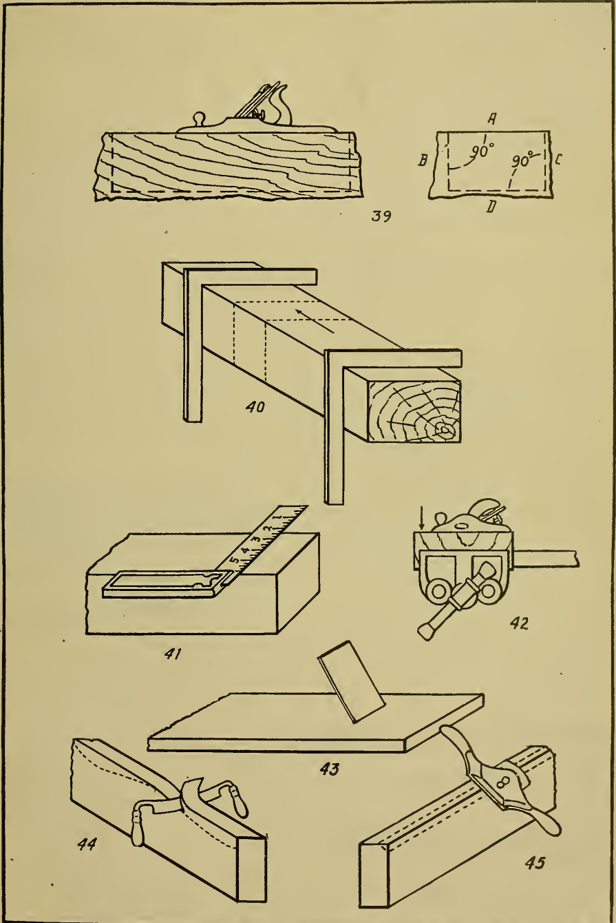
FIG. 39.—SQUARING STOCK. FIG. 40.—TESTING WITH SQUARE. FIG. 41.—MARKING END. FIG. 43.—USE OF CABINET SCRAPER. FIG. 44.—USE OF DRAW KNIFE. FIG. 45.—USE OF SPOKE SHAVE.
