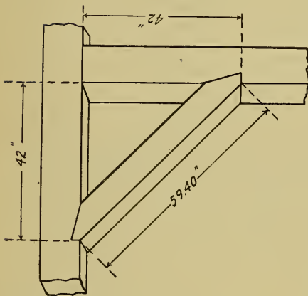
FIG. 174.—BRACE MEASURE.
