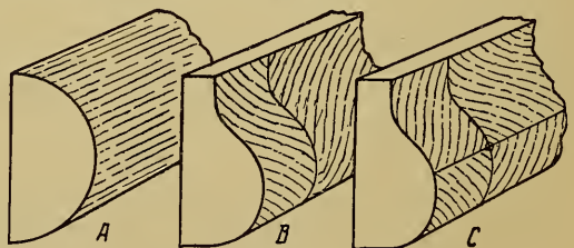
FIG 166.—SWELL DRAWER FRONTS.
