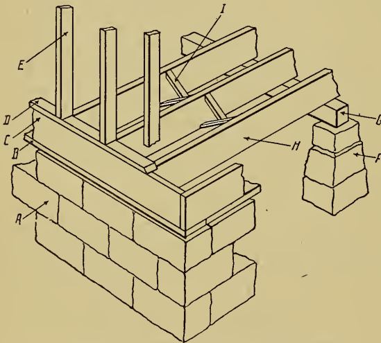
FIG. 149.—FOUNDATION FRAME. (BOX SILL.)
