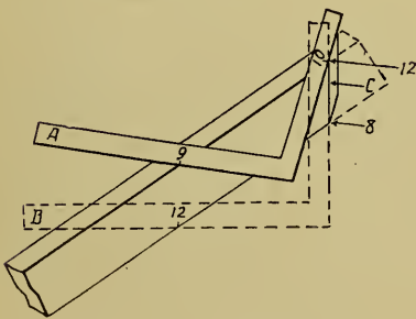
FIG. 180.—PLUMB AND HEEL OF RAFTERS.
