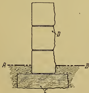
FIG. 148.—CROSS SECTION OF A FOUNDATION A B, Ground Level C, Footing D, Wall
