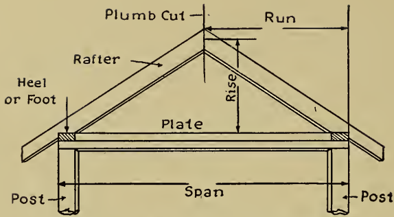
FIG. 177.—RUN AND RISE—COMMON RAFTER.
