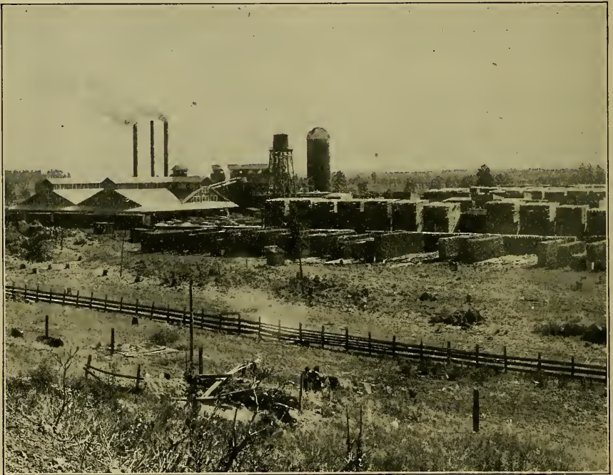
FIG. 241.—MILL AND YARD ON COCONINO NATIONAL FOREST, FLAGSTAFF, ARIZONA.
