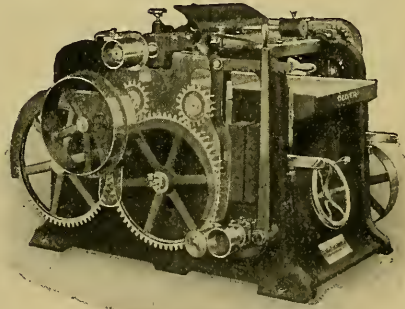
FIG. 102.—SURFACER.
