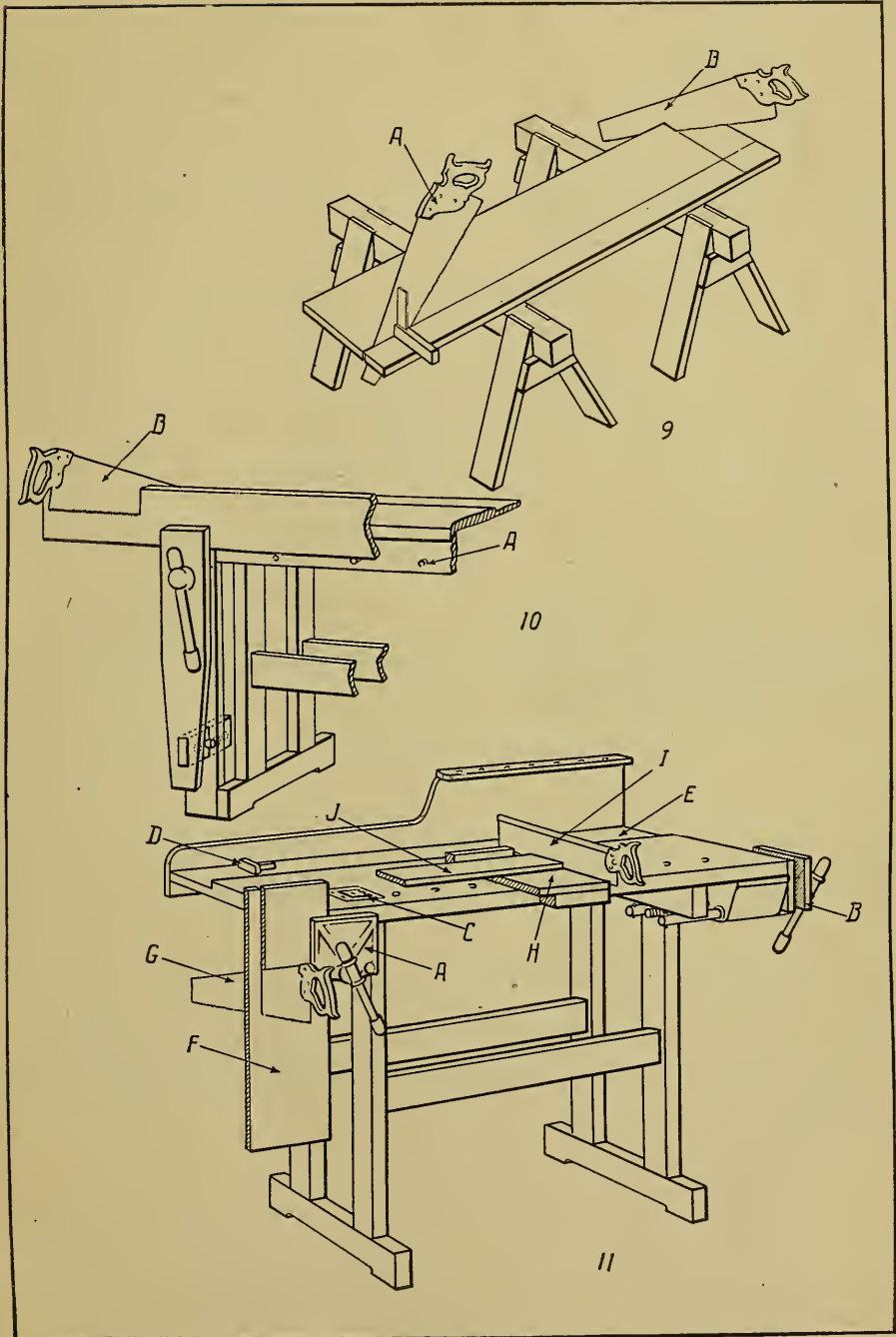
FIG. 9.—SAW HORSES. FIG. 10.—CARPENTER'S BENCH. FIG. 11.—SCHOOL SHOP BENCH.
