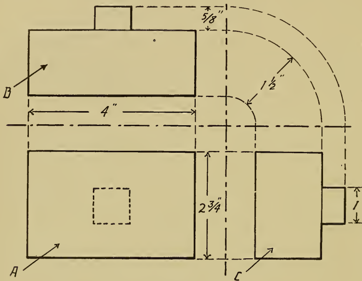
FIG. 1.—WORKING DRAWING.
