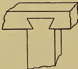
FIG. 118.—DOVETAIL DADO JOINT.
