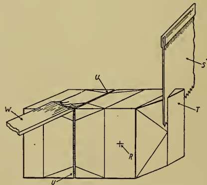
FIG. 94.—FORMING THE SUPPORT.
