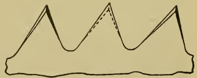
FIG. 197.—TEETH OF CUT-OFF SAW (CIRCULAR).
