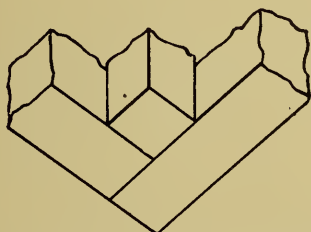
FIG. 115.—BUTT JOINT (BLOCKED AND GLUED).
