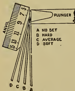
FIG. 200.—SAW SET SHOWING DEGREE OF SET.
