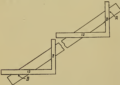
FIG. 181.—SIDE CUTS OF RAFTERS.
