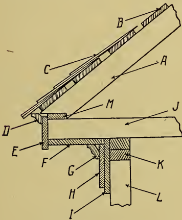
FIG. 151.—CORNICE.
