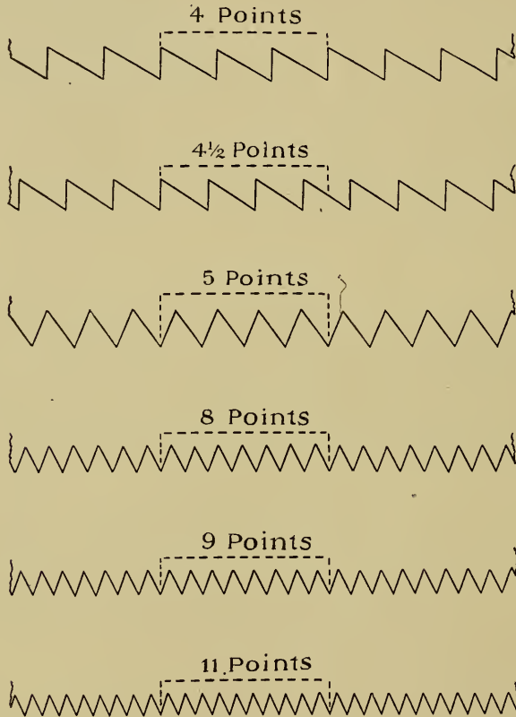
FIG. 190.—SIZE OF TEETH.
