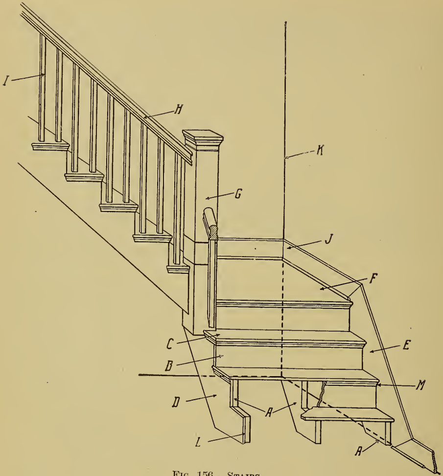
FIG. 156.—STAIRS.
