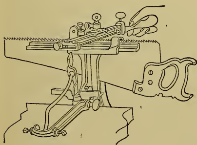
FIG. 194.—SAW CLAMP.
