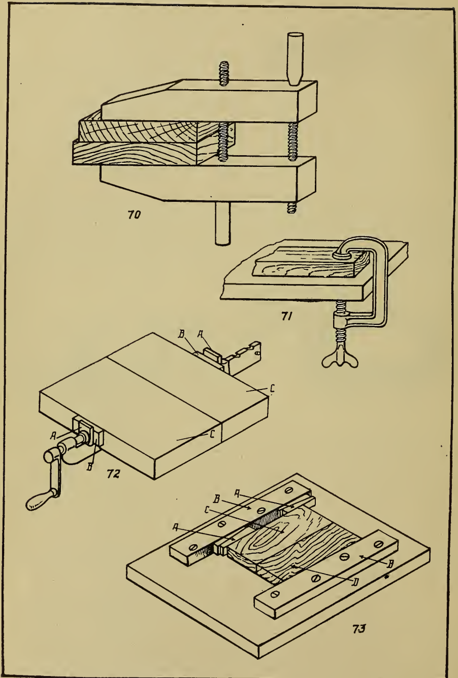
FIG. 70.—USE OF HAND SCREWS. FIG. 71.—USE OF C-CLAMP. FIG. 72.—USE OF BAR CLAMP. FIG. 73.—IMPROVISED CLAMP.
