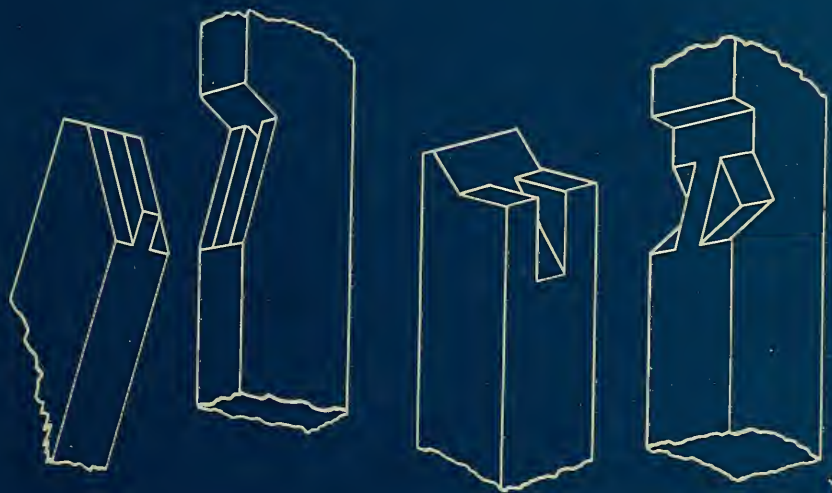
Oblique Mortise and Tenon Joint Scale \frac{3}{8}'' = 1'' 428
