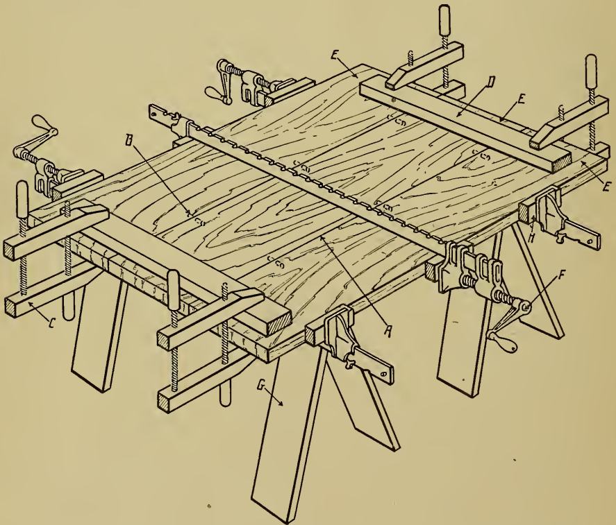
FIG. 140.—GLUING, SHOWING USE OF CLEATS, HAND SCREWS AND CLAMPS.
