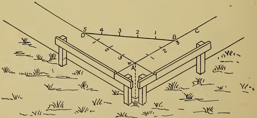
FIG. 147b. SQUARING THE FOUNDATION.
