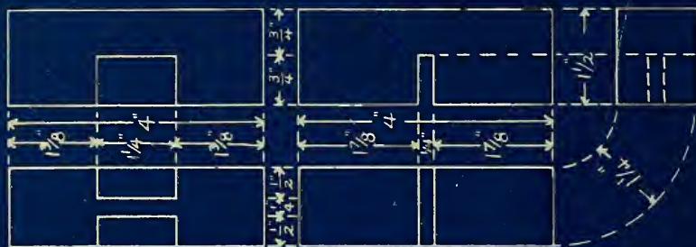
Lap Dovetail Joint Scale \frac{3}{8}'' = 1''
