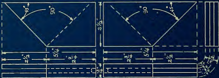
Splined Miter
