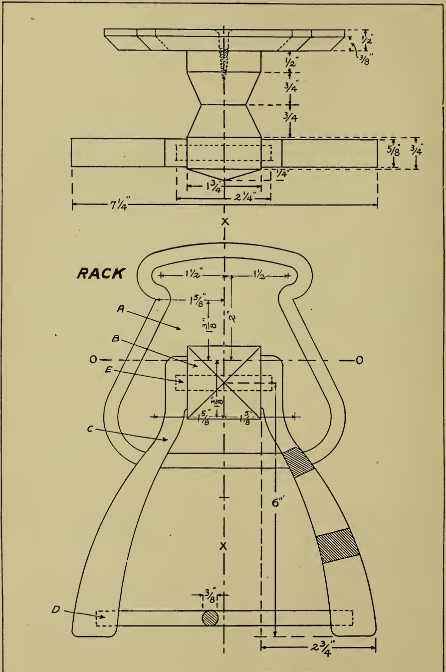
FIG. 90.—WORKING DRAWING OF A RACK.
