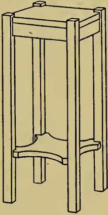
Top 10" X 10" Height 24½"
