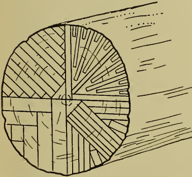
FIG. 243.—METHODS OF QUARTER-SAWING LUMBER.
