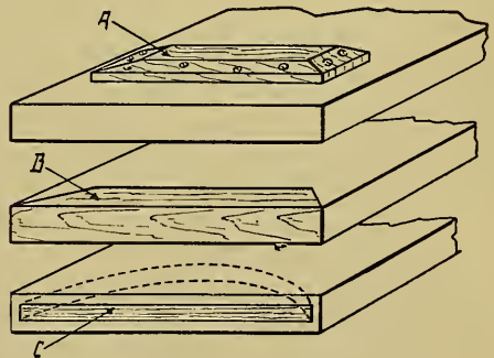
FIG. 142.—CLEATS.
