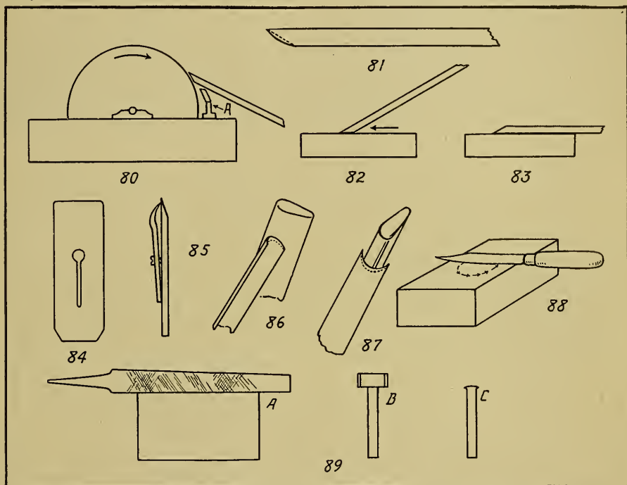
FIG. 80.—ADJUSTMENT OF TOOL TO GRINDSTONE. FIG. 81.—IMPROPER BEVEL. FIG. 82.—ADJUSTMENT OF TOOL TO OIL STONE. FIG. 83.—REMOVING WIRE EDGE. FIG. 84.—ROUNDED PLANE IRON EDGES. FIG. 85.—PLANE IRON AND CAP ATTACHED. FIG. 86.—SHARPENING OUTSIDE BEVELED GOUGE. FIG. 87.—SHARPENING INSIDE BEVELED GOUGE. FIG. 88.—SHARPENING KNIFE. FIG. 89.—SHARPENING CABINET SCRAPER.
