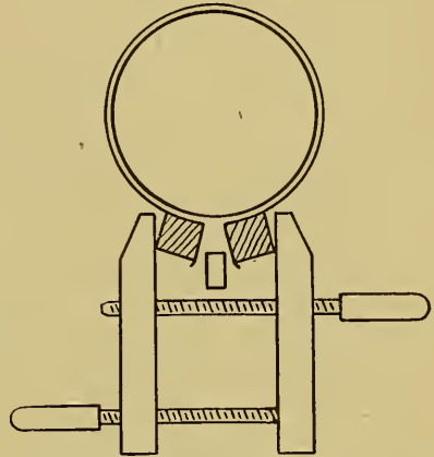
FIG. 168.—VENEER CLAMP FOR CYLINDERS.
