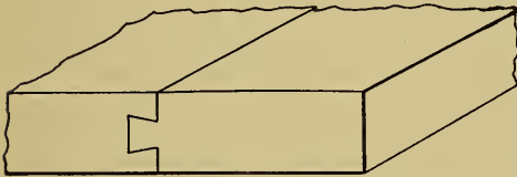
FIG. 141.—WEDGE DOVETAIL JOINT.
