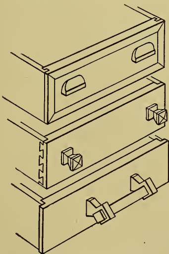
FIG. 139.—DRAWER FRONTS.
