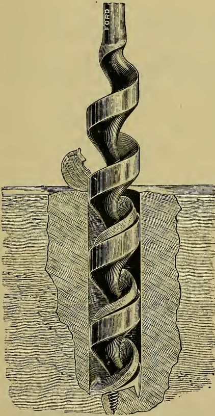
FIG. 214.—CUTTING ACTION OF A BIT.
