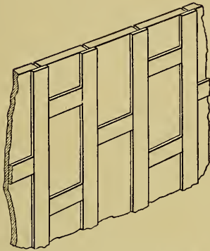
FIG. 138.—BATTED PANELS.
