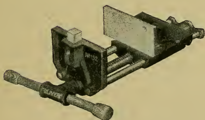
FIG. 5.—RAPID-ACTING VISE.
