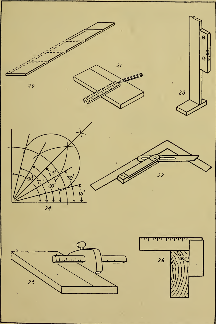
FIG. 20.—LAYING OFF LENGTHS. FIG. 21.—PENCIL LINING. FIG. 22.—DETERMINING ANGLES AND PITCHES. FIG. 23.—PLUMBING. FIG. 24.—ESTABLISHING ANGLES. FIG. 25.—ESTABLISHING LINES. FIG. 26.—TESTING WITH TRY SQUARE.
