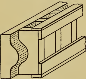
FIG. 165.—BUILT-UP CAUL.
