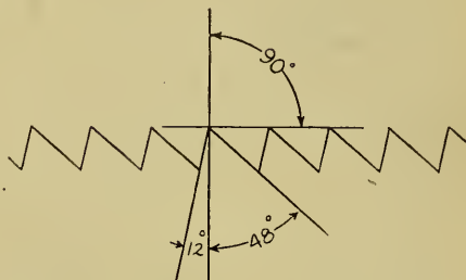
FIG. 192.—CROSS-CUT TEETH, SHOWING ONE-FOURTH PITCH.
