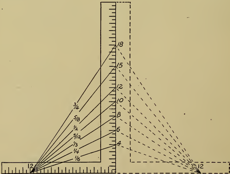
FIG. 178.—PITCH OF ROOFS.
