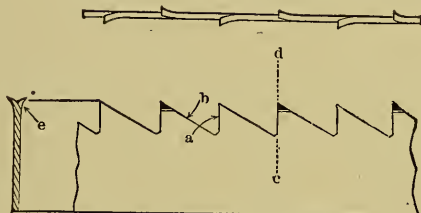
FIG. 193.—PARTS OF TEETH.
