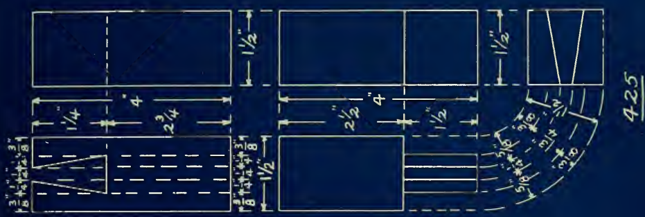
single Dovetail (Thru)
