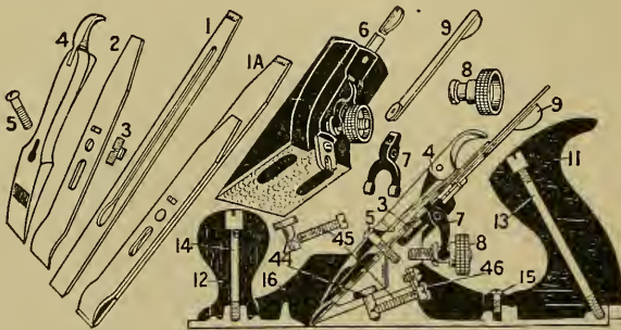
FIG. 32.—JACK PLANE AND PARTS.
