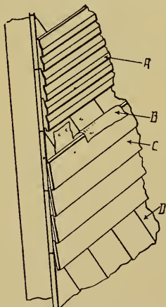
FIG. 154.—SIDING.
