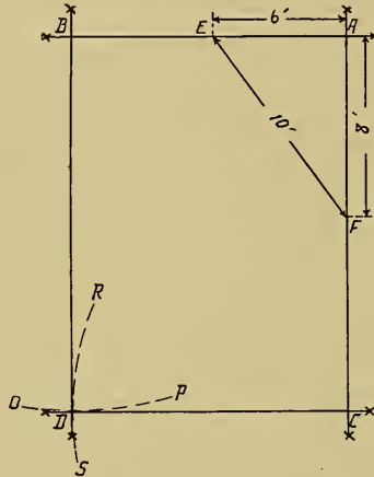
FIG. 147a. SQUARING THE FOUNDATION.
