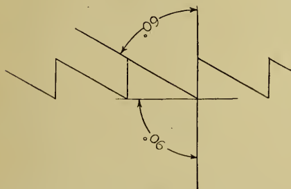
FIG. 191.—RIP-SAW TEETH, SHOWING ONE-HALF PITCH.
