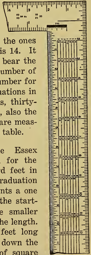
FIG. 171.—ESSEX BOARD MEASURE.
