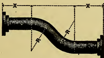
OFFSET BENDS
