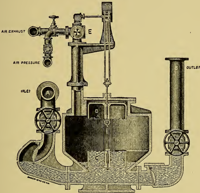
Fig. 179 Shone Pneumatic Ejector
