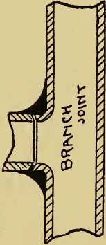
ROUND JOINT
