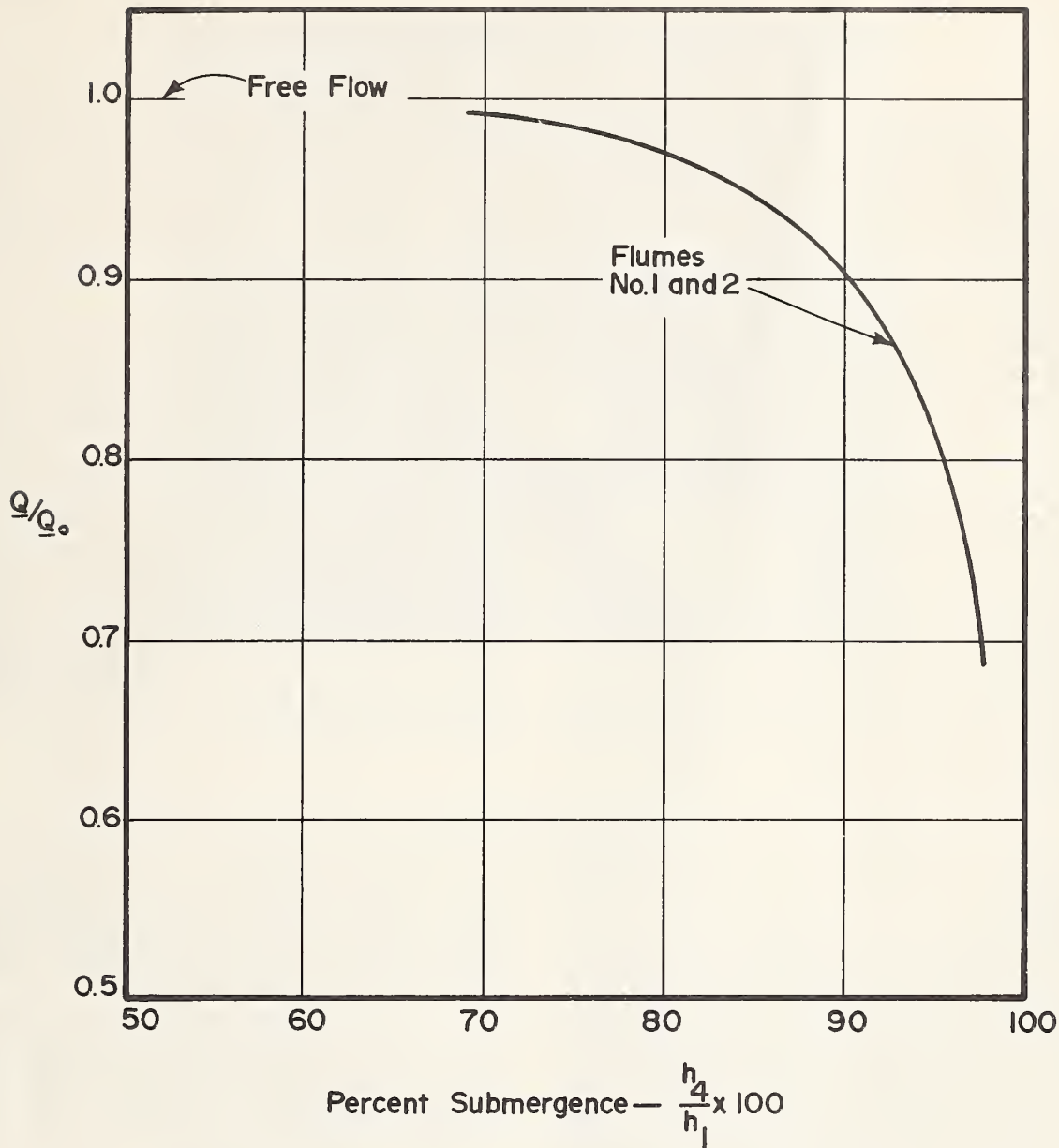
Figure 5.--Effect of submergence on discharge, flumes Nos. 1 and 2.
