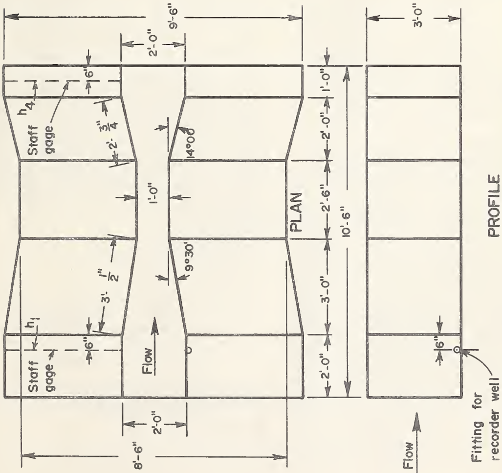
Figure 3.---Trapezoidal flume for 2-foot irrigation channels (flume No. 2).
