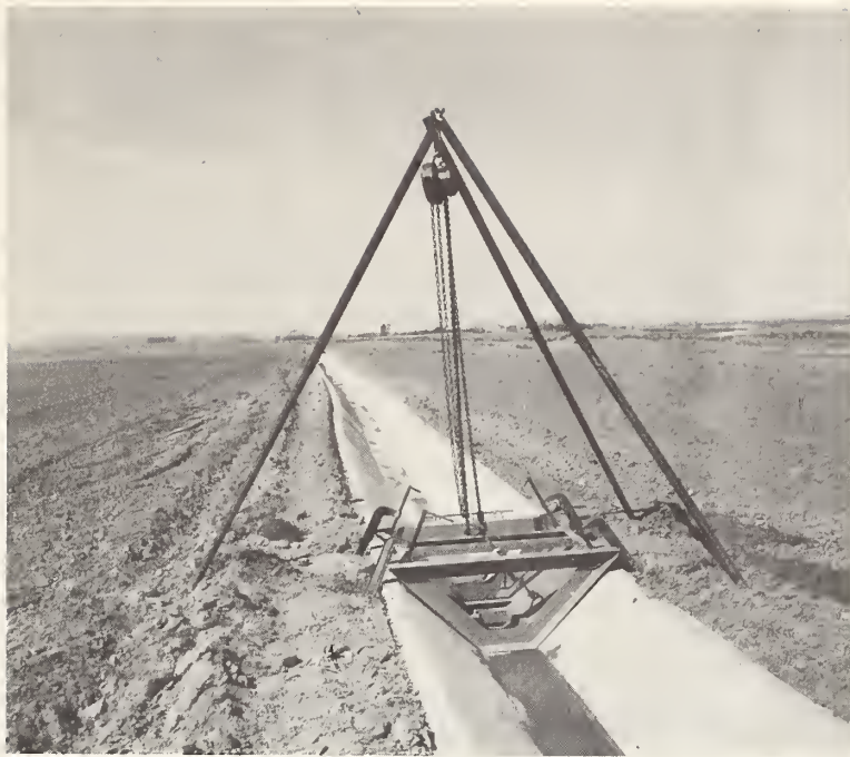
Figure 6.--Portable form used to pour trapezoidal flumes in concrete ditches
