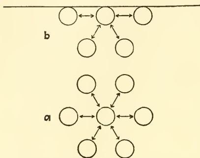
FIG. 2.—Diagram illustrating the balanced attraction exerted upon a molecule in a mass of liquid (a), and the unbalanced attraction upon a molecule at the surface (b). The two-pointed arrows ( \leftrightarrow ) indicate mutual attraction between two molecules.
