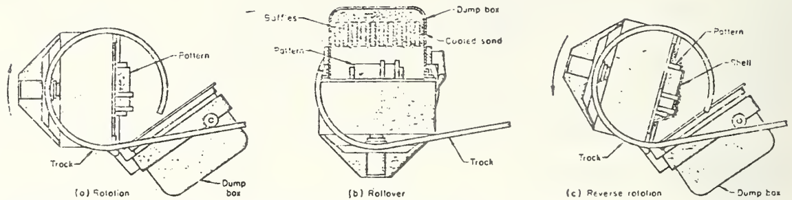
Variation A: Dump-box method in which pattern and dump box are rotated at high speed on a circular track
