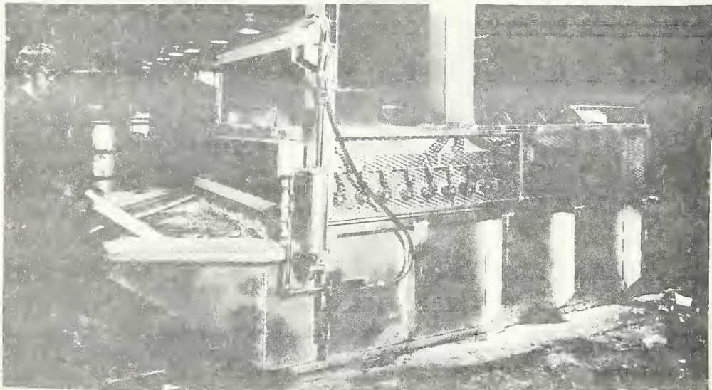
FIGURE 8 Electric Reverbatory Furnace for Melting Aluminum
