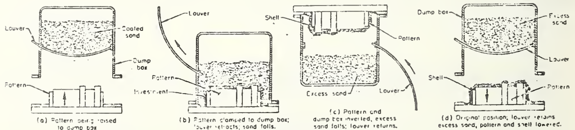
Variation B: Shell mold made by using a lower type dump box
