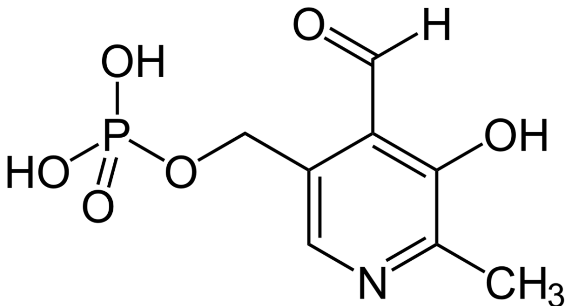
Abb. 1762 Pyridoxal-5'-phosphat.
