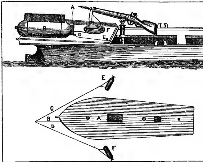
TORPEDOES.
