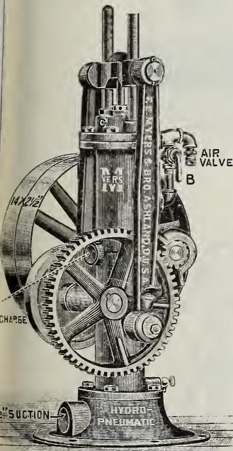
Vertical Power Hydro Pneumatic Pump Fig. 1440
