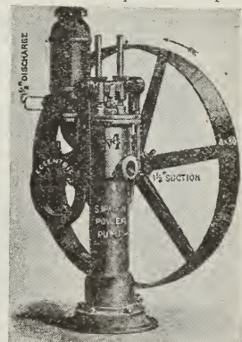
Power Siphon Pump Fig. 1226
