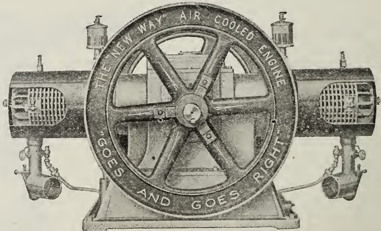
8 AND 12 H. P. TWIN CYLINDER
