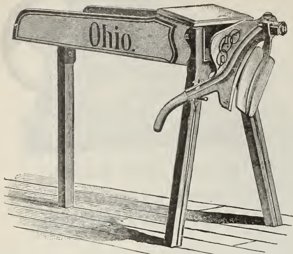
"Ohio" Lever Cutter
