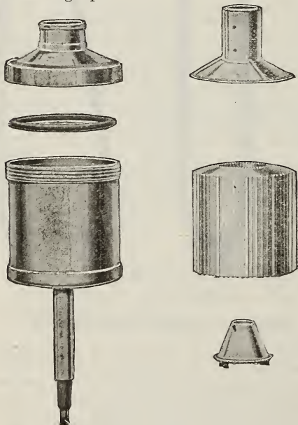
The LINK-BLADE Bowl complete. This bowl, 900 lbs. capacity, is only 4\frac{1}{2} " diameter, 5" deep, and runs at only 7700 R. P. M.
