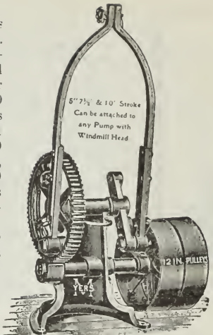
Fig. 1114, Pump Jack
