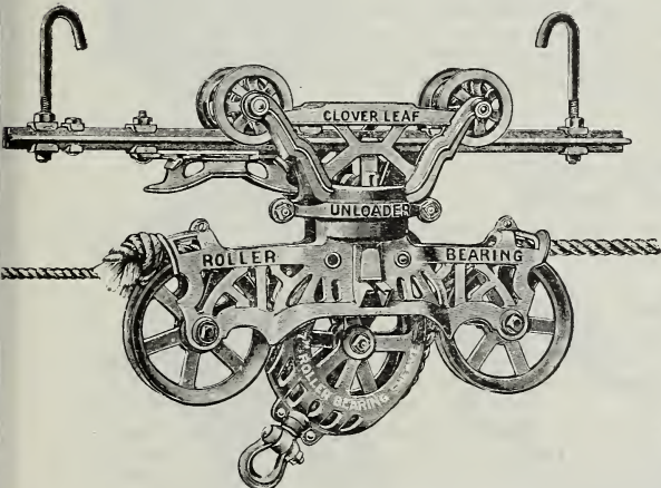
Myers Clover Leaf Unloader
