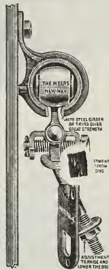
The Myers New-Way Adjustable Tandem Door Hanger For Tubular Girder Track Adjustable to and from Building and to Raise and Lower the Door
