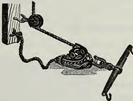
No. 628 Snatch Block Pulleys Price, each, $0.55 Useful in limited space, horse only travels half distance.
