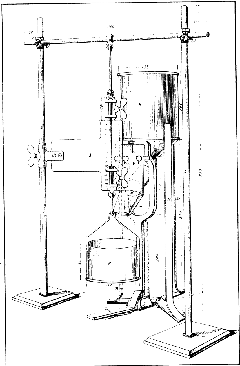
FIG. 1. Mechanical device for determining the elastic constants of coir and abacá filaments.
