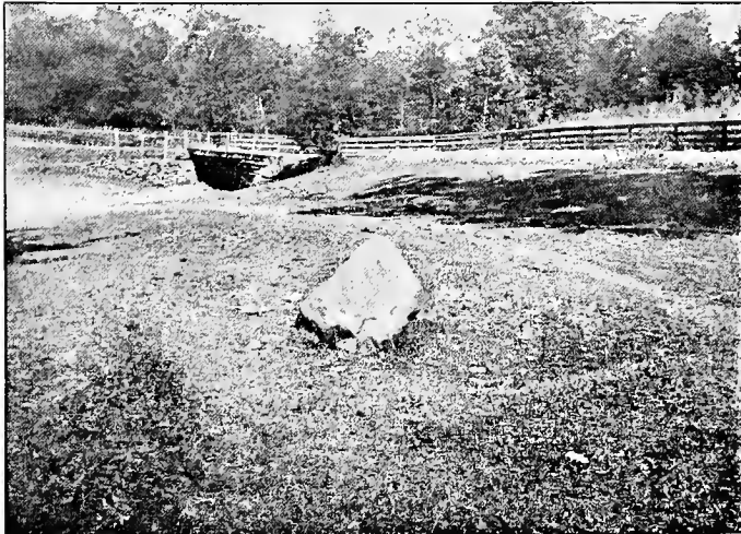
FIG. 90.—Conglomerate boulder found in Boone County, Kentucky. (See text.)
