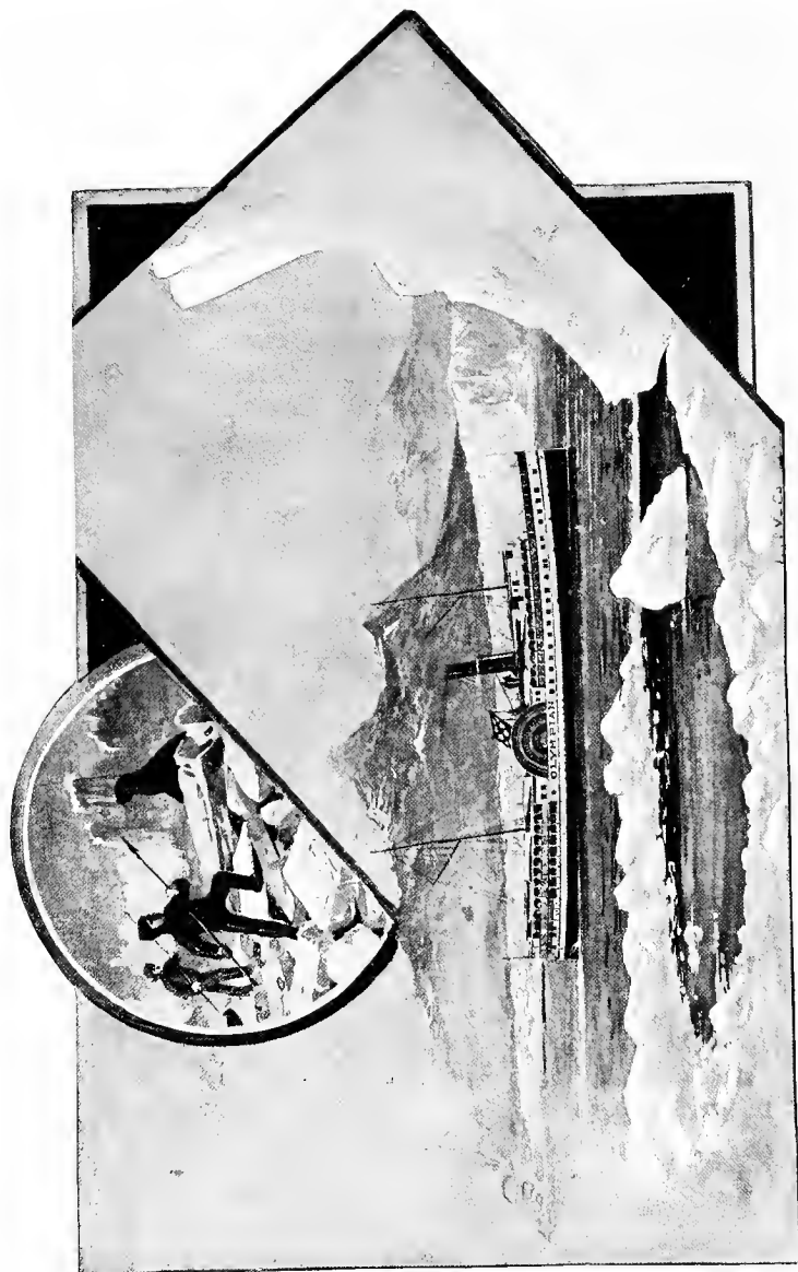
FIG. 21.—Front of Muir Glacier, side view. (By courtesy of C. S. Fee.)
