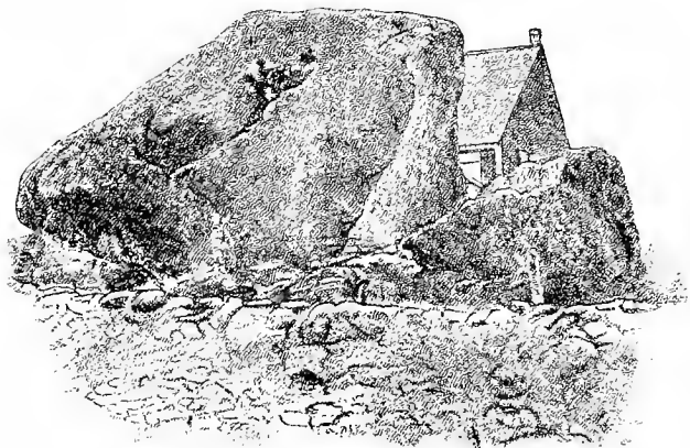
FIG. 60.—Vessel Rock, a glacial boulder in Gilsun, N. H. (C. H. Hitchcock.)
