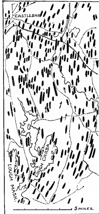
FIG. 79.—Drumlins in Ireland, after Kinnahan and Close. (Davis.)
