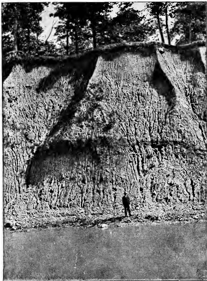
FIG. 118.—Section in till near Darrtown, Butler County, Ohio, sixty-five feet high. Coarse line of stratification near the middle. Fresh cedar logs at the bottom. (See text.) (United States Geological Survey.) (Wright.)
