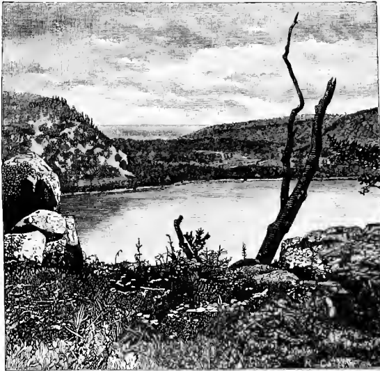
FIG. 120.—Devil's Lake, near Baraboo, Wisconsin. This is held in place in a preglacial channel by a dam of glacial débris several hundred feet above the river, and but a short distance from it. (United States Geological Survey.) (Chamberlin.)
