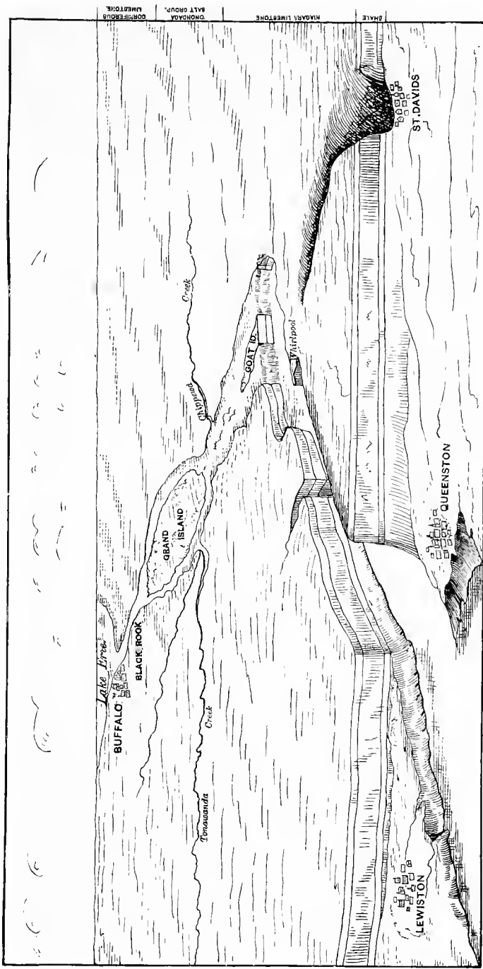
Fig. 107.—Bird's-eye view of Niagara River. (Pohlman.) (By courtesy of American Institute of Mining Engineers.)
