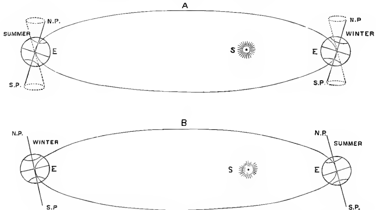
FIG. 103.—Exaggerated view of the earth's orbit, showing the effects of precession of the equinoxes. A, condition of things now; B, as it will be 10,500 years from now.
