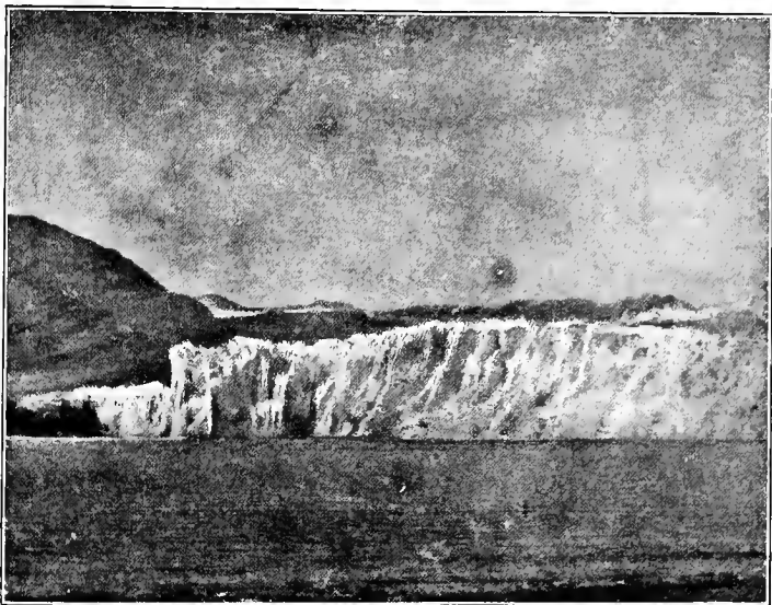
FIG. 27.—Shows central part of the front of Muir Glacier one half mile distant. Near the lower left hand corner the ice is seen one mile distant resting for about one half mile on gravel which it had overrun. The ice is now retreating in the channel. The buried forests described lie just beyond. (From photograph.)
