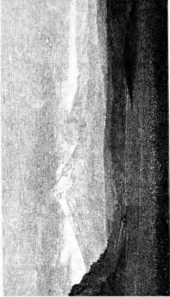
FIG. 13.—Mount Shasta, California. United States Geological Survey (Russell).
