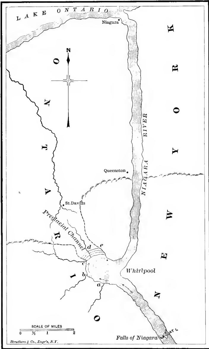
FIG. 109.—Map of the Niagara River below the falls, showing the buried channel from the whirlpool to St. Davids. Small streams a , b , c , fall into the main gorge over a rocky escarpment. No rock appears in the channel at d , but the rocky escarpment reappears at e .
