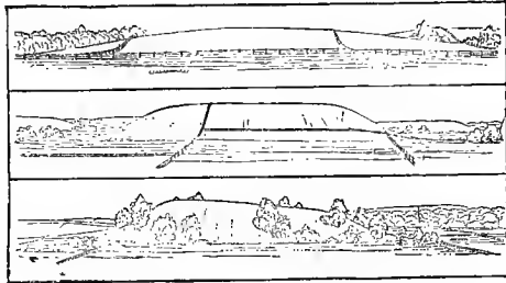
FIG. 76.—Outline of parallel drift-hills, in central New York. (Davis.)
