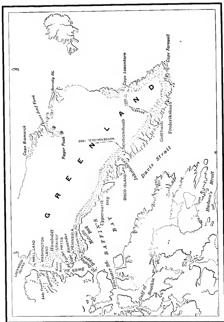
FIG. 20.—Map of Greenland. The arrow-points mark the margin of the ice-field.
