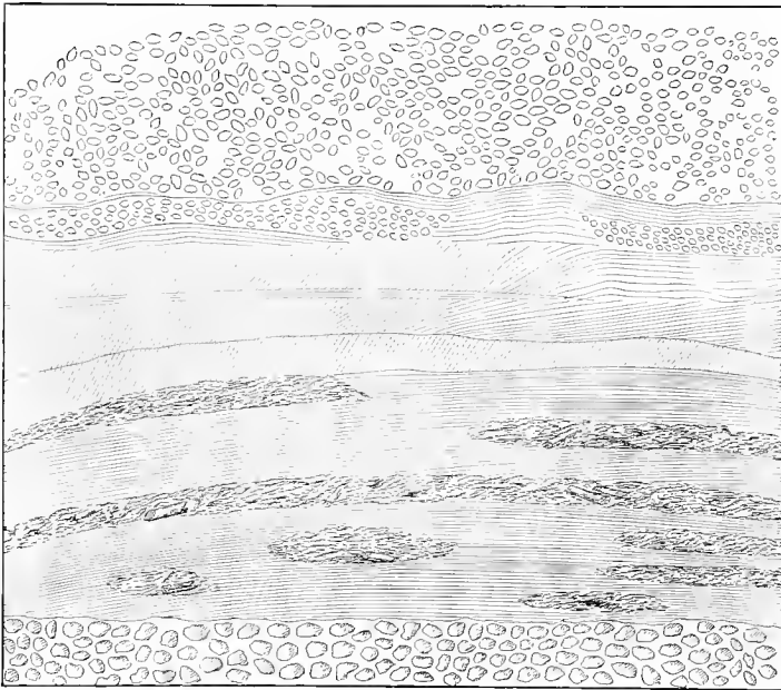
FIG. 49.—Section of the deposit at Point Wilson described in the text, showing one hundred and fifty feet in height, about one hundred of which is coarsely stratified, and contains layers of vegetable matter. Bowlders from till at the top have fallen down to form a talus at the water's edge.
