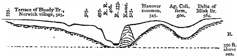
FIG. 87.—Section across the Connecticut Valley, from Norwich, Vermont, to Hanover, New Hampshire, distance three miles. The kame is nearly covered by later river silt. (Upham.)
