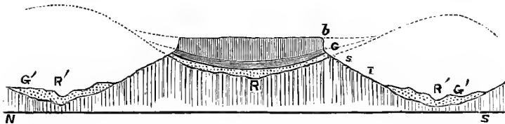
FIG. 143.—Section across Table Mountain, Tuolumne County, California. b, b , lava; G, G' , gravel; s, s , slate; R, R , old river-bed; R', R' , present river-bed. (Le Conte.)
