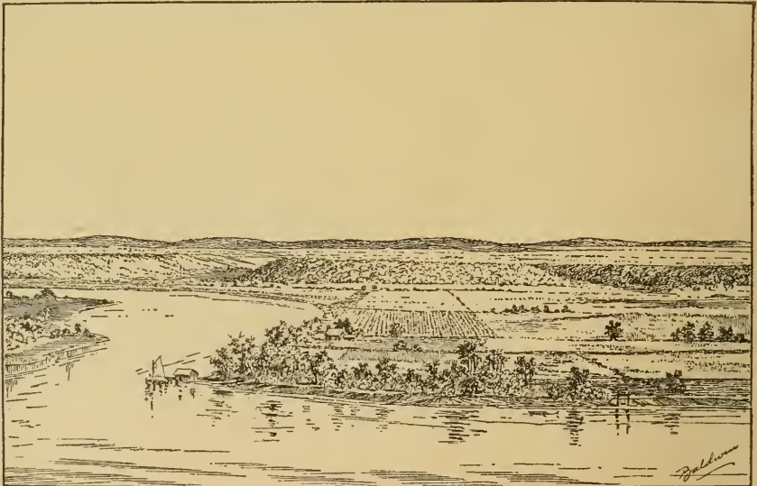
FIG. 14.—Meadow in foreground terrace of Leonardtown loam, with Norfolk loam and Windor sand in background.
