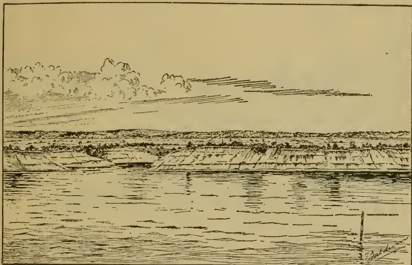
FIG. 15.—Leonardtown loam, with Norfolk loam and Windsor sand in background.
