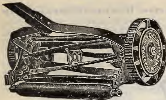
Style K Mower.
