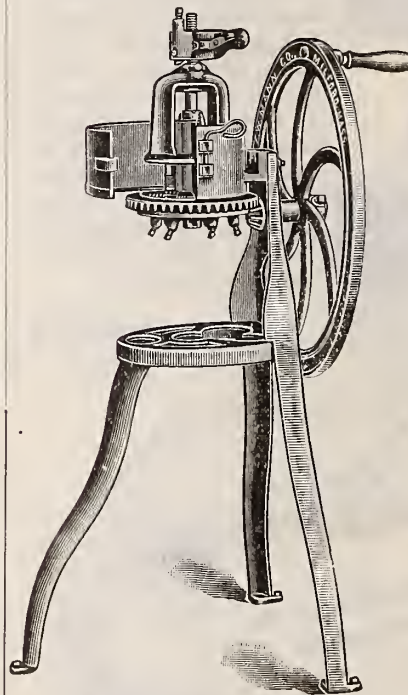
Mann Bone Cutter No. 7.
