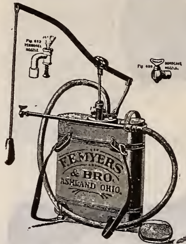
Myers Perfect Knapsack Spray Pump.
