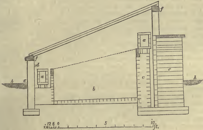
Fig. 336. Section of the pine pit at Oakhill.
