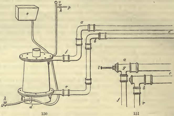
Fig. 150. Rogers's boiler, with the heating-pipe joined to it. Fig. 151. Rogers's substitute for a stop-cock.
