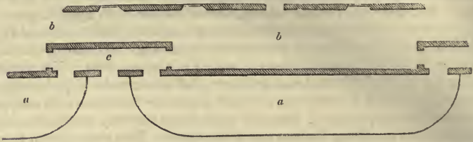
Fig. 129. Ground plan of a curvilinear plant-house, with the entrance through a lobby in the back walls.
