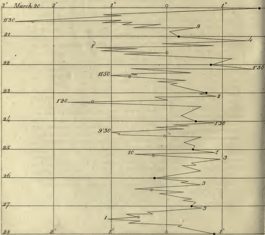
Graphical representation of the daily variation of the needle at Port Bowen
