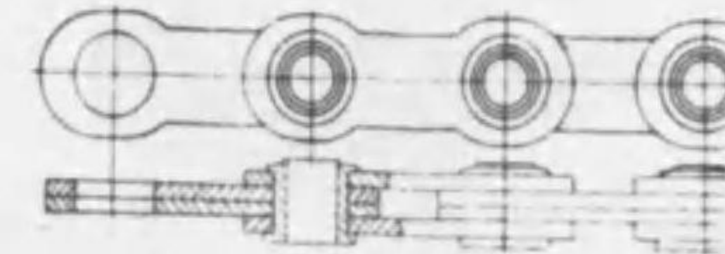
1x2 Balance Weight Chains
