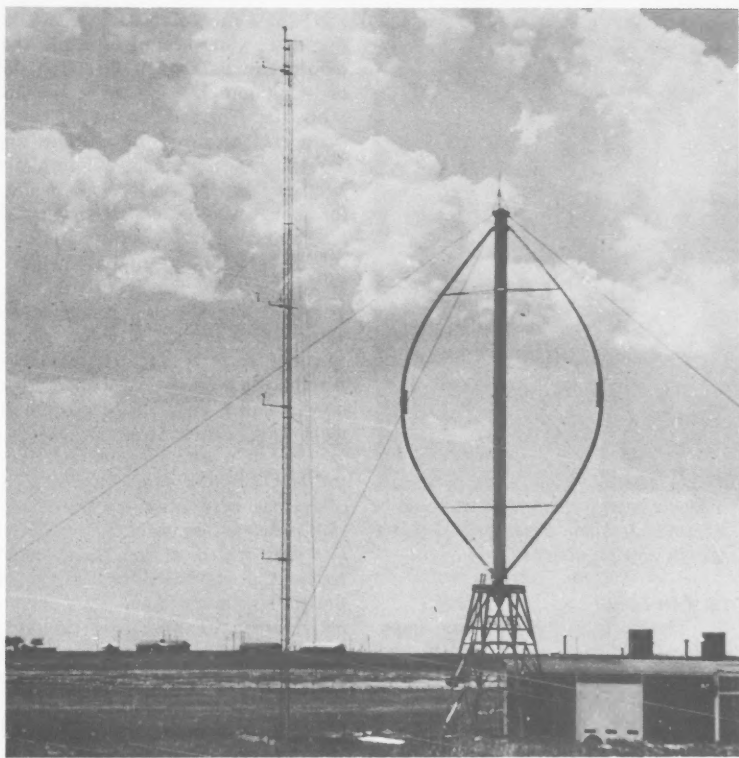
This is a 40-kilowatt, vertical-axis wind turbine. It's at the Department of Agriculture's research center in Bushland, Tex. The turbine is used for pumping, but electricity production is possible. Tower at left collects meteorological data for assessing turbine's performance. (Photo by Battelle Pacific Northwest Laboratories)
